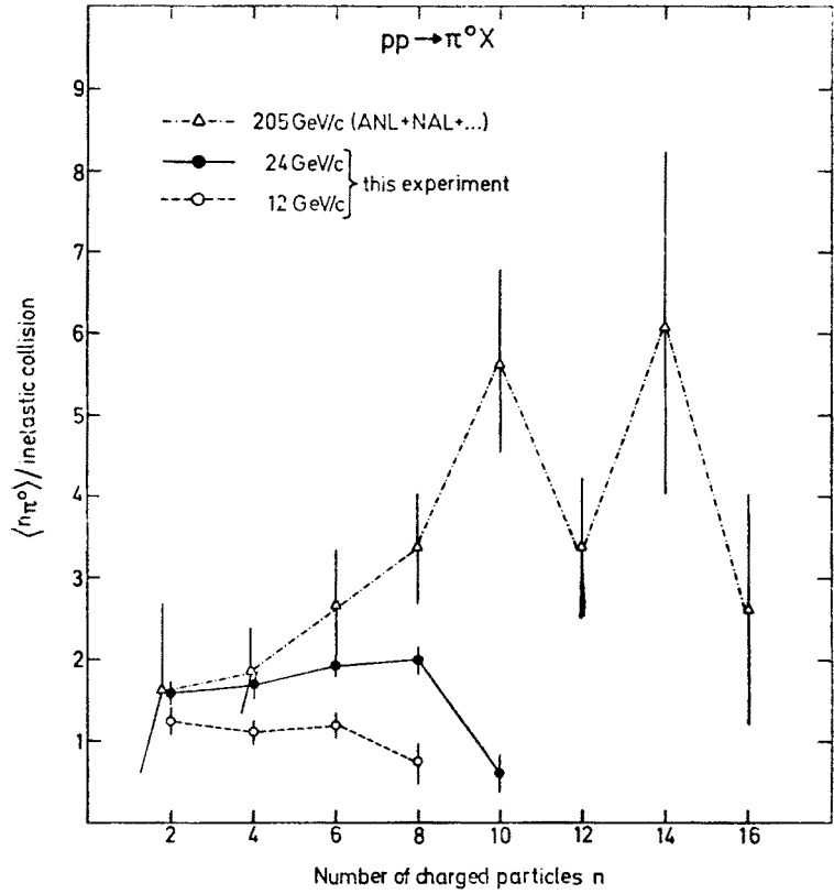
Fig. 3. \bar{n}_{\pi^0} vs prong number n at 12, 24 and 205 GeV/c (Bonn-Hamburg-München collaboration [57] and Ref. [21])
