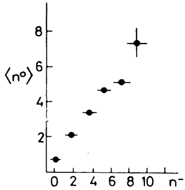
Fig. 2. \bar{n}_{\pi^0} vs number n_- of negative particles at \sqrt{s} = 53 \text{ GeV} (CERN-Hamburg-Vienna collaboration, from Ref. [7])
