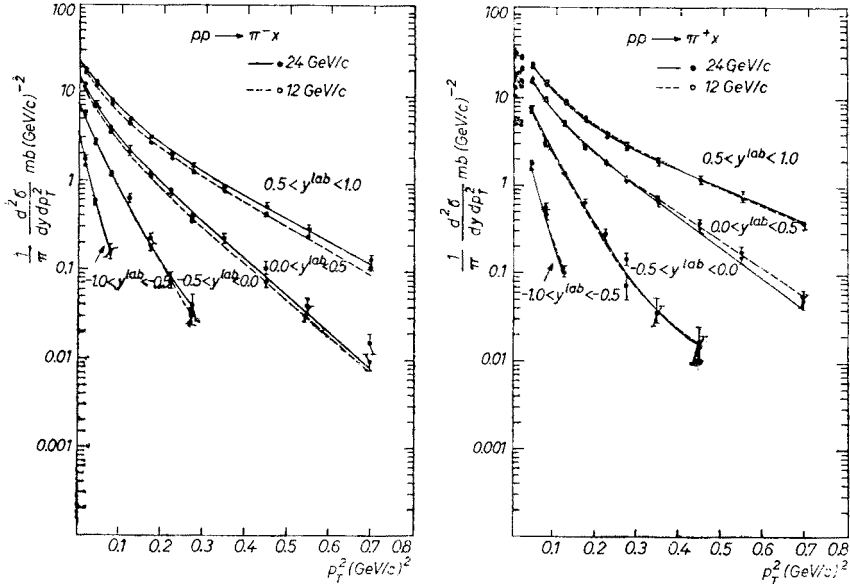
Fig. 49. Invariant cross sections vs p_T^2 for \pi^- and \pi^+ at 12 and 24 GeV/c for four intervals of the lab rapidity in the fragmentation region (from Ref. [57b])
