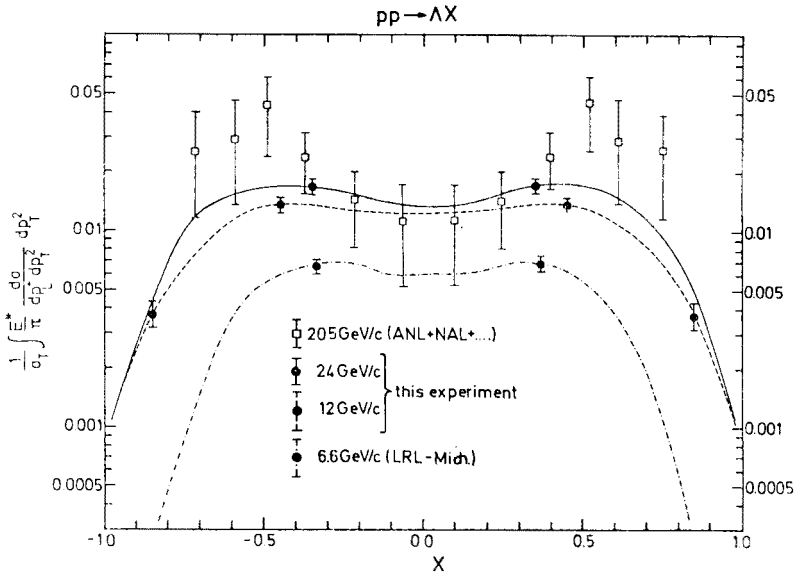
Fig. 37. Normalised x -distributions of \Lambda , integrated over p_T , at various lab momenta (from Ref. [57c])
