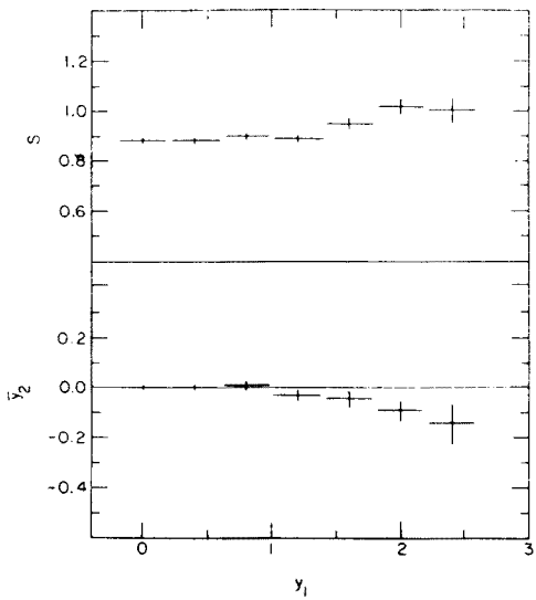
Fig. 59. Width S and position \bar{y}_2 of the maximum of the Gaussian fits in Fig. 58 vs y_1 (from Ref. [70])
