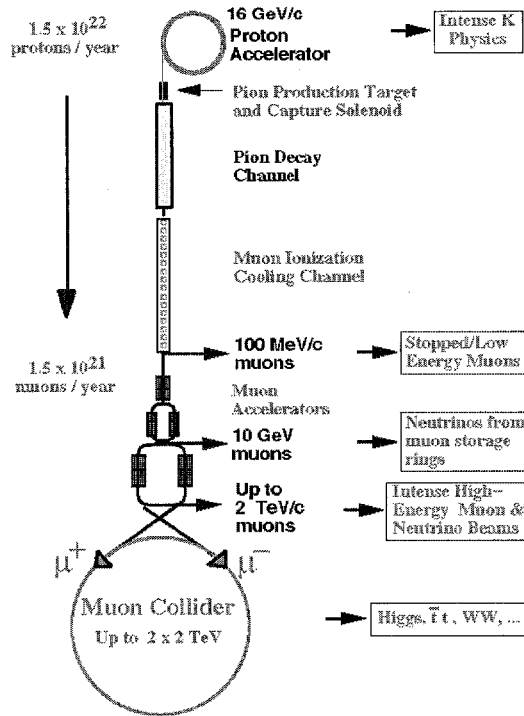
Figure 1. A schematic view of a \mu^+\mu^- collider facility, showing a high-intensity proton source which would produce pions. \pi decay produces \mu 's which are cooled to collider intensities, and accelerated. Counterrotating \mu^+ and \mu^- bunches are inserted into a storage ring for high-luminosity collisions.
