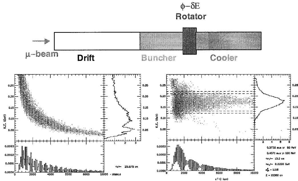
Figure 4: “High-frequency” buncher and phase rotation consisting of a \sim 100\text{m} drift followed by a \sim 60\text{m} “buncher” in which the beam is transported through a 300-200 MHz rf system which forms the beam into a string of bunches, which are then aligned in energy by a \sim 200 MHz high-gradient rf system ( \phi - \delta E rotator). The lower left figure shows simulation results of beam at the end of the buncher and the lower right shows beam at the end of the \phi - \delta E rotator.
