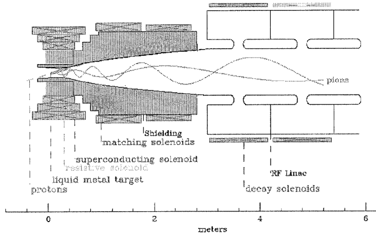
Figure 3: Possible target and initial capture system. A high intensity proton beam hits a liquid metal target inside a high-field solenoid, capturing \pi 's which are focussed into a lower field solenoidal transport system for \pi \rightarrow \mu + \nu decay; the \mu 's are captured and cooled.
