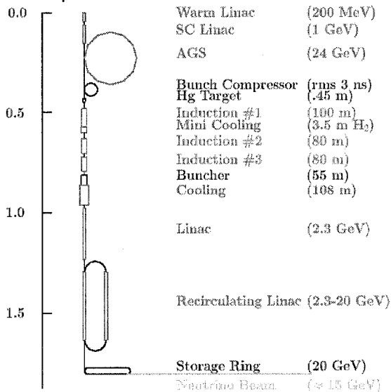
Figure 2. A schematic view of a \mu -storage ring \nu -factory. A proton driver produces \mu 's which are cooled and accelerated to 20 GeV and inserted in a storage ring. \mu -decay ( \mu \rightarrow e + \nu_\mu + \bar{\nu}_e ) in the storage ring straight section provides collimated electron and muon neutrino beams suitable for long baseline oscillation experiments.
