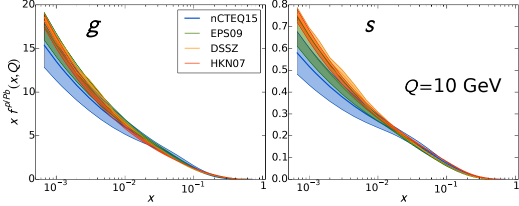
Figure 3: Selected PDF flavors from nCTEQ15 [1] compared with results from the literature [3–5].
