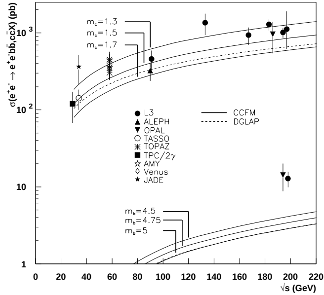
Fig. 1. Cross sections for charm and beauty production in e^+e^- collisions [2].
