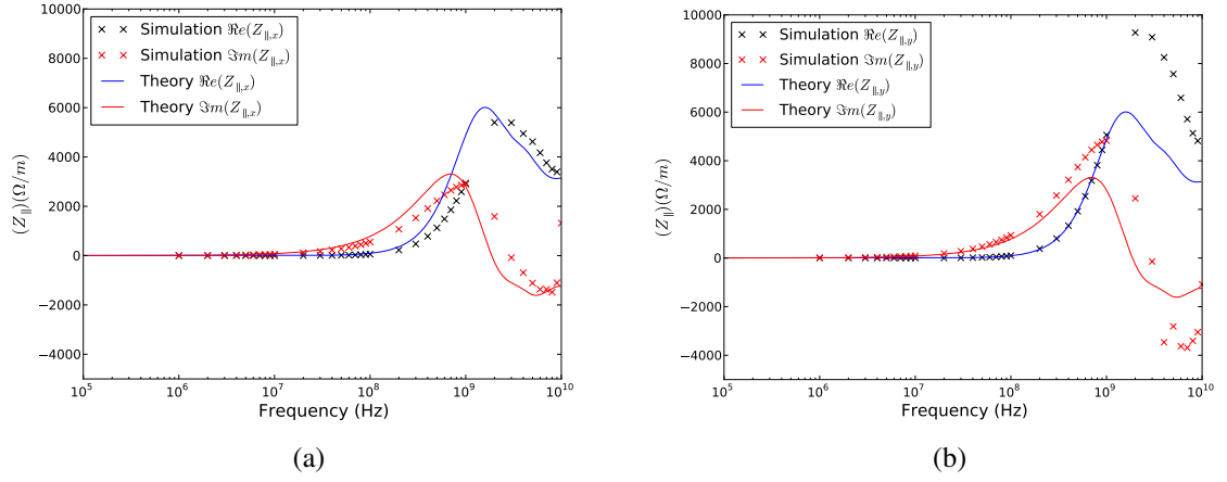
Figure 4.10: The longitudinal impedance of two parallel ferrite plates simulated using a longitudinal coaxial wire. Presented is the impedance as measured in the horizontal plane ((a)) and in the vertical plane (b).
