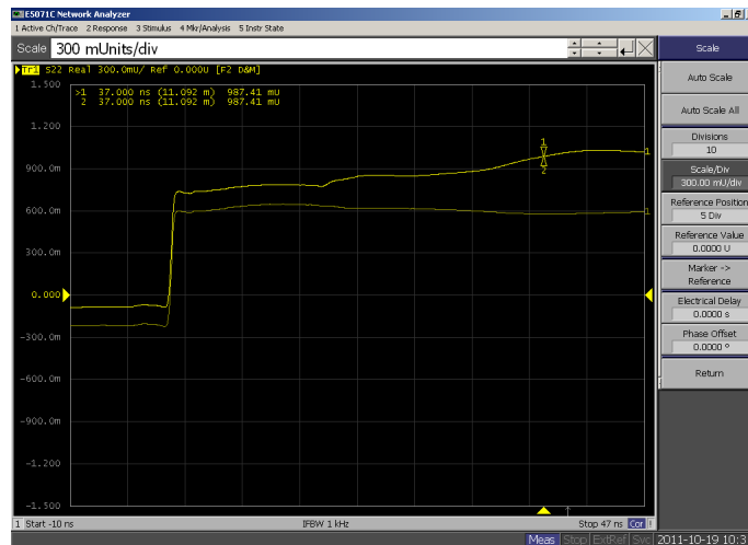
Figure 4.4: An example of a reflection measurement made with and without matching resistors. The faded line (lower trace) is the measurement with matching, the bold line (upper trace) that without. The reduction in the reflection can be seen due to the flatter line after the initial reflection.
