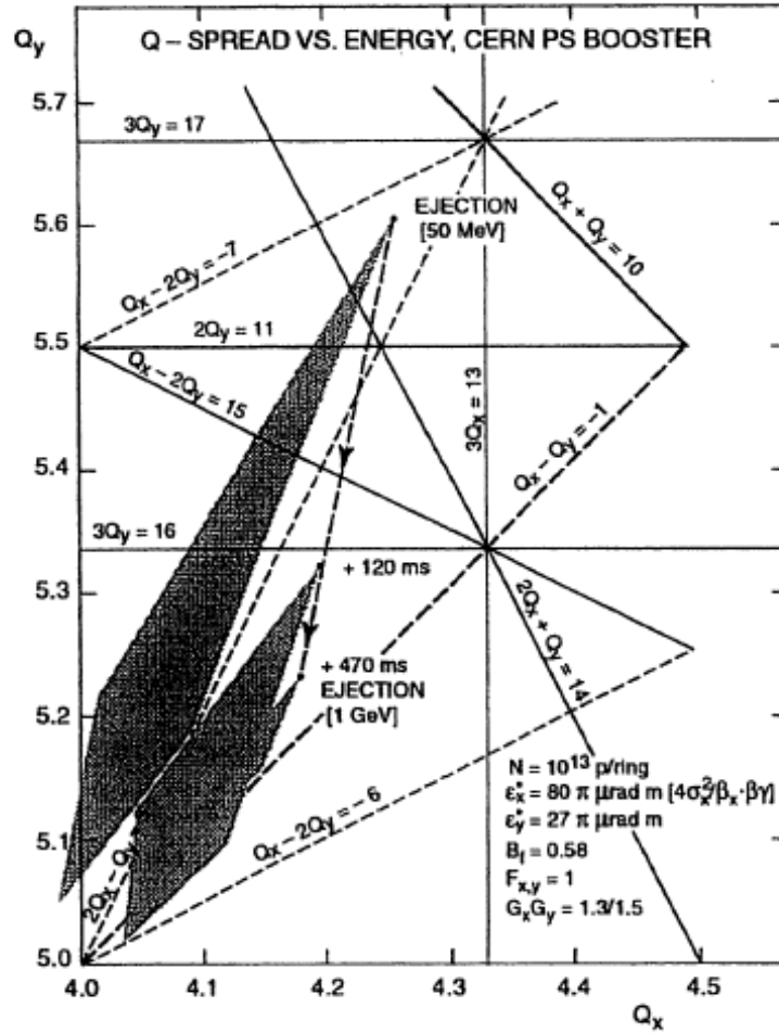
Figure 2.18: A tune diagram illustrating the unperturbed tune of a machine, and the resulting perturbed tune and the tune spread as a result of direct space charge interactions on a bunch. Note that the tune spread has caused some particles to lie upon a major resonance harmonic. Taken from K. Schindl [42].
