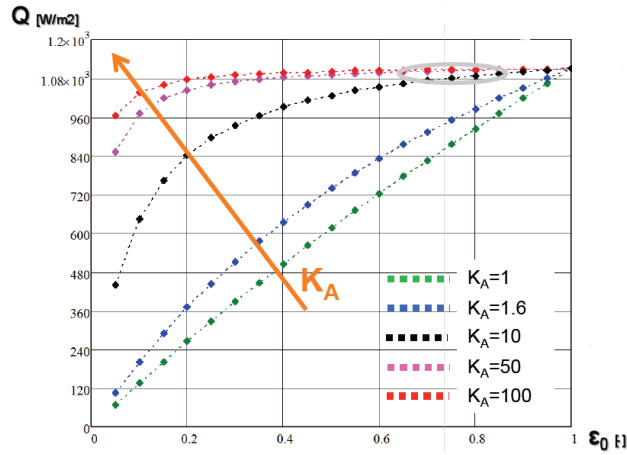
Figure F.1: The power transfer between two surfaces by radiative heat transfer as a function of emissivity of the absorbing component and the ratio of the visible surface areas of the components. K_A is the ratio of the surface of the absorbing component and the emitting component. Figure produced by Garlasche et al [125].
