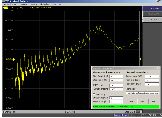
Figure 4.5: An example of the resonance pattern seen whilst performing measurements using the resonant method. Each peak corresponds to one data point in the final measurements. Taken from measurements of the LHC injection kicker magnets.
