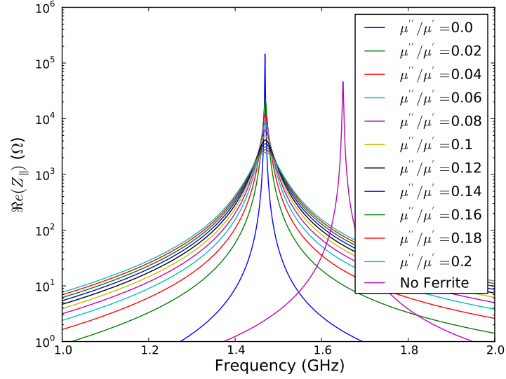
Figure 6.10: The real component of the longitudinal beam coupling impedance of a cavity without and with shielded damping material with \epsilon' = 10 , \mu' = 10 and \mu''/\mu' is varied. The non-damped cavity is shown for comparison. The change in resonance frequency and shunt impedance impedance is due to the increased \epsilon' of the damping material.
