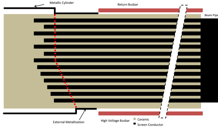
Figure 8.32: The proposed final MKI design. A combination of alternating and tapered screen conductors is used, along with a step out of the external metallization to a metal cylinder. The outline of the step out is shown by the red-dashed line.
