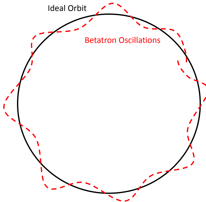
Figure 1.3: An illustration of betatron oscillations around the ideal orbit of a circular accelerator. These oscillations occur in both the horizontal and vertical planes.
