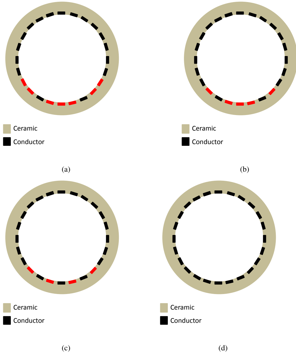
Figure 8.19: Beam screens with different numbers of screen conductors removed from the design quantity of 24. Models of 17 (a), 19 (b), 20 (c) and 24 (d) screen conductors are considered for the impedance simulations. Conductors that are coloured red are the removed in each case.
