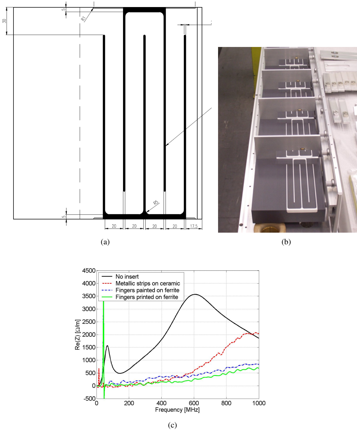
Figure 6.4: An example of serigraphy in the SPS Extraction Kicker Magnets (SPS-MKE). The layout of the interleaved fingers is shown in (a) and the actual serigraphed ferrites in (b). A comparison of the measured real component of the longitudinal beam coupling impedance with and without the serigraphy is shown in (c).
