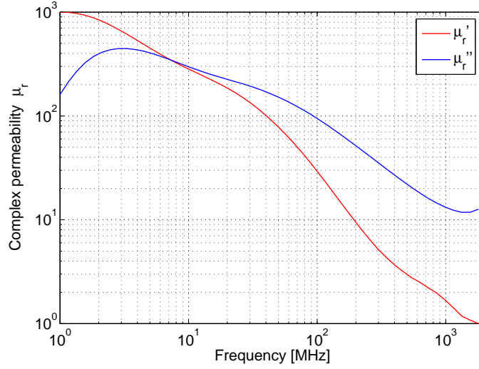
Figure 6.5: The complex permeability of a sample ferrite of the sort used for damping. In this case 8C11. In usage a high Curie temperature ( T_c ) ferrite is recommended, such as TT2-111R.
