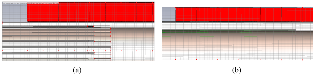
Figure 8.22: A comparison of the mesh that may be generated in CST Particle Studio using both the full model (a) and the cutdown model (b). Note the greatly increased mesh density in the important overlap region between the screen conductors and external metallization. The simulation time for the first is on the order a of day, for the second 30 minutes.
