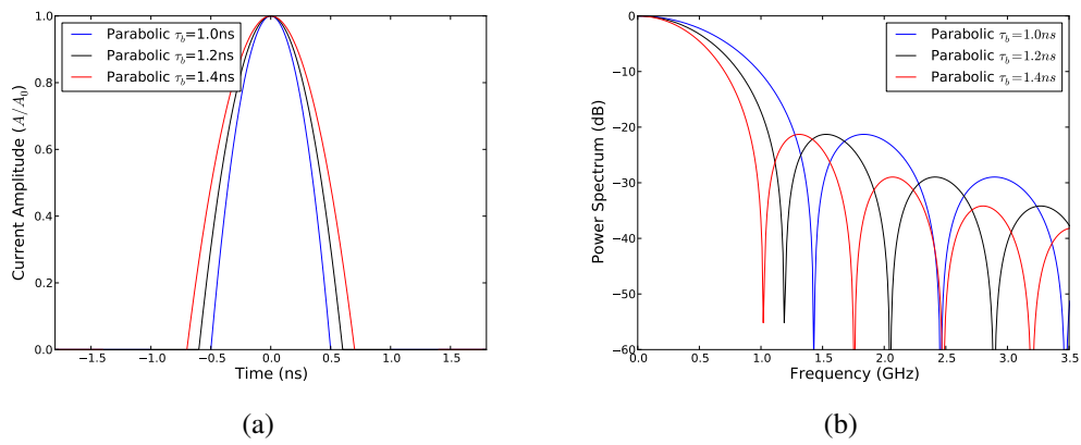
Figure 2.11: (a) The longitudinal profile and the (b) associated bunch power spectrum for a number of bunch lengths assuming a parabolic bunch profile.
