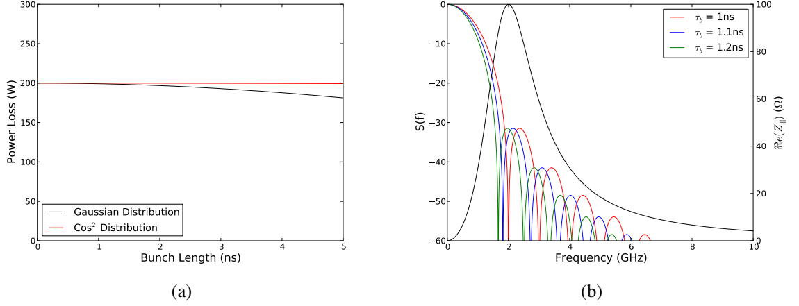
Figure 2.17: (a) The change in power loss due to a narrow band resonance characterised by \omega_0 = 2 \text{ GHz} , R_s = 100 \text{ } \Omega , Q = 1 interacting with a \cos^2 bunch distribution with different bunch lengths. The impedance and the beam power spectrum are shown in (b) to illustrate how this relates to the power loss.
