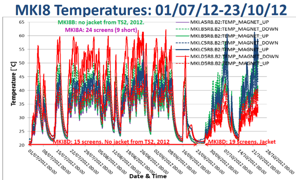
Figure 8.15: The temperature profile of the IP8 injection kicker magnets during the time period before and after technical stop 3 (TS3), when the MKI8d was changed from a kicker magnet with 15 screen conductors to one with 19 screen conductors. It can be seen this magnet (solid red trace) goes from being the magnet with the highest measured temperature to the magnet with the lowest measured temperature after TS3 (17/09/2012 - 27/09/2012).
