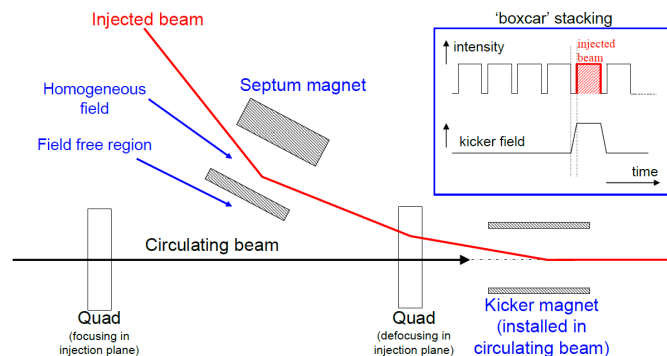
Figure 8.1: An example layout of an injection system for an accelerator with the timing of the kicker field with an injected bunch train. Taken from [91].
