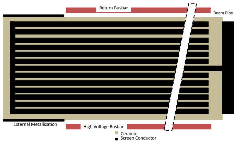
Figure 8.30: A MKI beam screen design using an alternative screen conductor layout in which 2 (cross section shown here) conductors are connected to ground at one end of the screen, and all conductors are connected together at the other end. Both ends have capacitive coupling.
