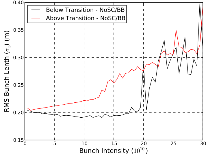
Figure 2.19: The change in the bunch length of a proton beam in the SPS due to the effects of a broadband resonator impedance ( f_{res} = 1 \text{ GHz} , R_s = 10 \text{ } \Omega , Q = 1 ) without space charge. Note that the bunch length increases when the beam is above transition, and decreases below transition, as the bunch intensity is increased.
