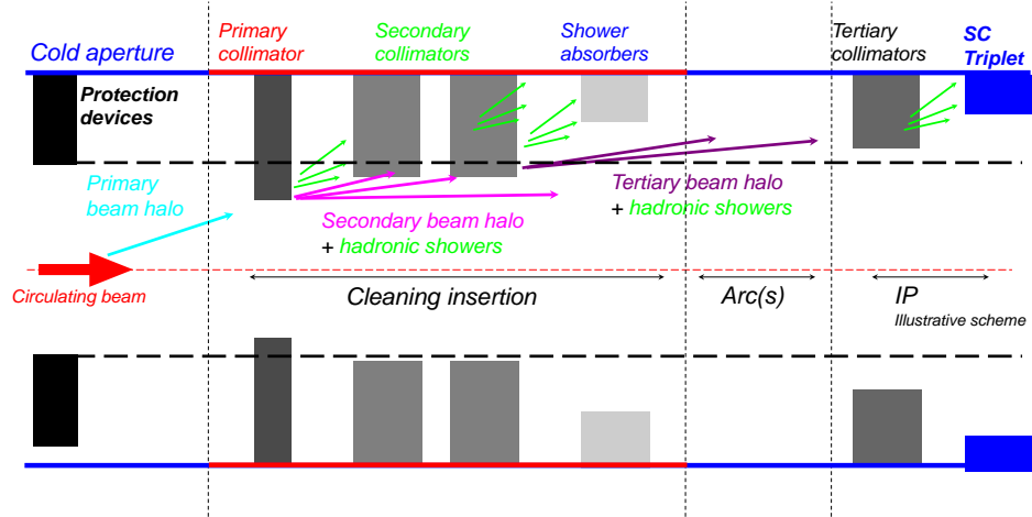
Figure 7.1: The processes by which the collimation system in the LHC acts to clean the beam and manage losses in a controllable way. Taken from [78].
