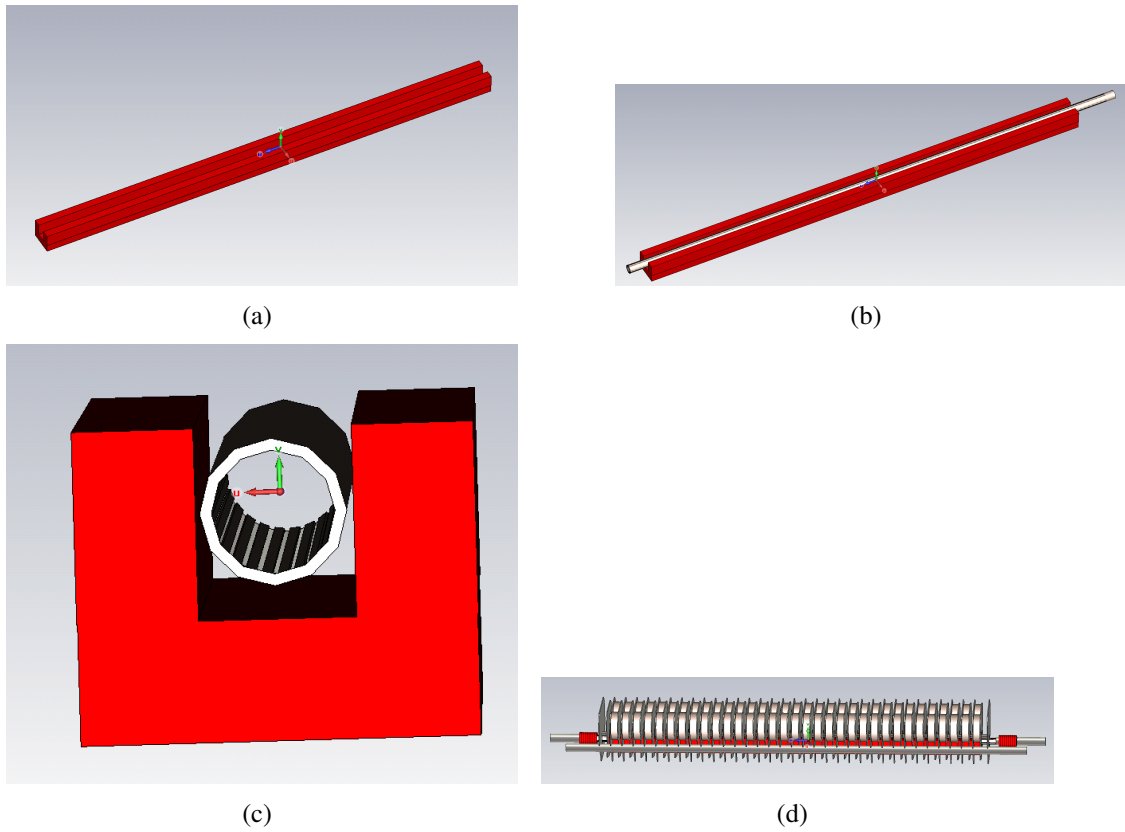
Figure 8.16: The geometries simulated for the various components in the LHC-MKI. These are c-core ferrite only (a), c-core ferrite and the ceramic tube (b), c-core ferrite with the ceramic tube containing 24 screen conductors (c) and finally the complete MKI magnet (without vacuum tank for clarity) (d).
