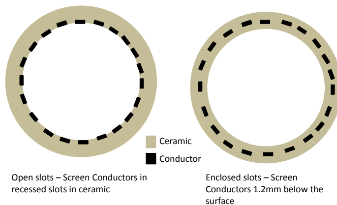
Figure 8.29: A MKI beam screen design with enclosed slots (shown in comparison to the usual beam screen design with open slots) for the screen conductors.
