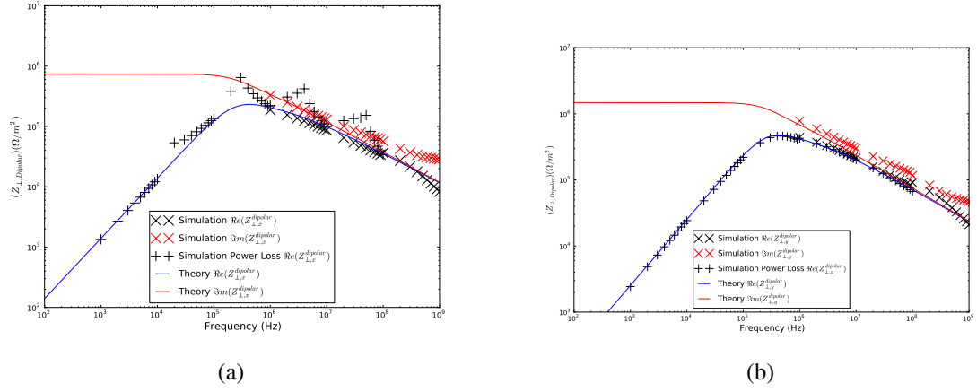
Figure 4.14: The dipolar impedance of two parallel graphite plates measured using two longitudinal coaxial wires. Presented is the impedance as measured in the horizontal plane ((a)) and in the vertical plane (b).
