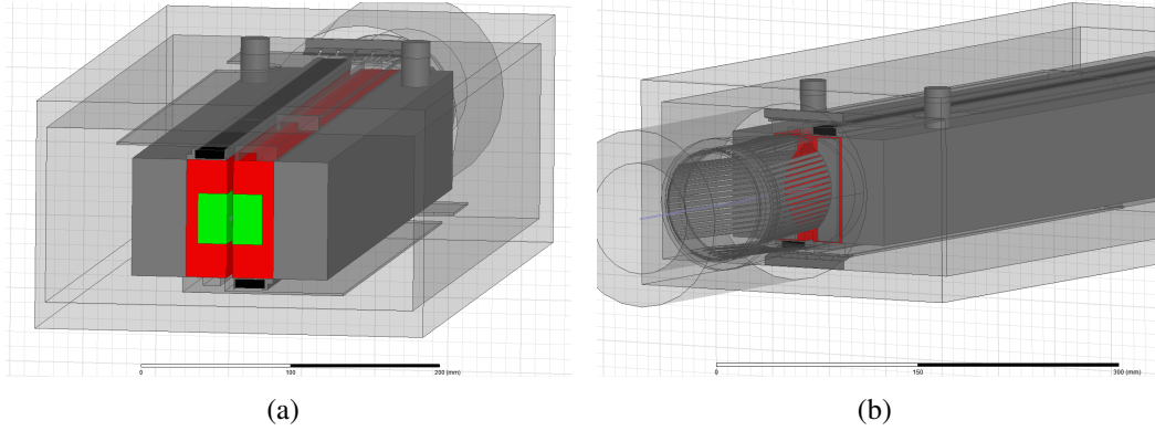
Figure 7.9: The TCTP collimator has a number of important impedance reduction techniques present in its design. Ferrite tiles replace the sliding transverse RF contacts of the phase 1 design, shown in (a) (ferrite tiles shown in black) to reduce the resonant Q of the structure. The longitudinal RF fingers, shown in (b), provide a good conducting path for the beam image current in the transition from the beam pipe to the collimator jaw.
