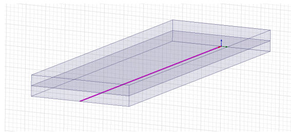
Figure 4.9: An example of the simulation model used for coaxial wire simulations. In this case a displaced single wire between two parallel plates. The wire is highlighted in purple.
