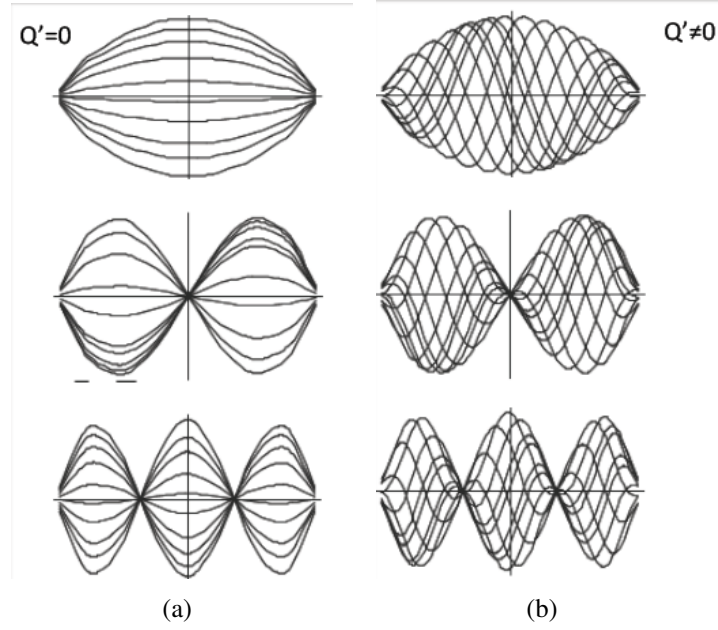
Figure 2.20: Examples of a number of modes of headtail oscillations without 2.20(a) and with 2.20(b) chromaticity. Note that radial and azimuthal modes may occur, as may coupled modes, in which the motion of the horizontal and vertical planes is coupled. Images courtesy of G. Rumolo [43].
