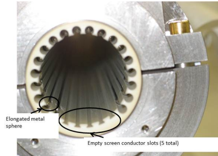
Figure 8.13: The additional screen conductors and the elongated spheres place in MKI8d to reduce both beam coupling impedance and the electric field.
