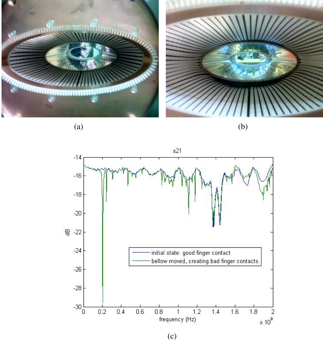
Figure 6.3: The layout of the RF fingers in the VMTSA both in (a) the fully operational configuration and (b) when some RF fingers lose contact. (c) shows the transmission parameter S_{21} for the VMTSA module with and without good electrical contact between the fingers and the beam pipe as acquired by coaxial wire measurements. Photos and measurements courtesy of J.L. Nougaret.
