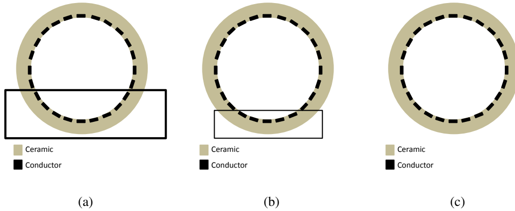
Figure 8.18: Beam screens with different numbers of screen conductors removed from the design quantity of 24. Models of 15 (a), 19 (b) and 24 (c) screen conductors are considered for the impedance simulations. Conductors surrounded by the boxes are removed in this case.
