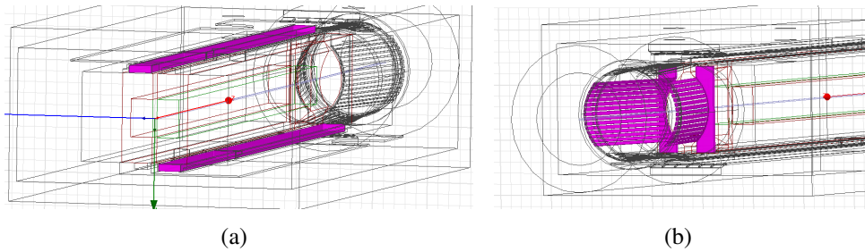
Figure 7.13: The different thermally sensitive components of the TCTP collimator highlighted in purple. (a) shows the ferrite tiles, and (b) the longitudinal RF fingers.
