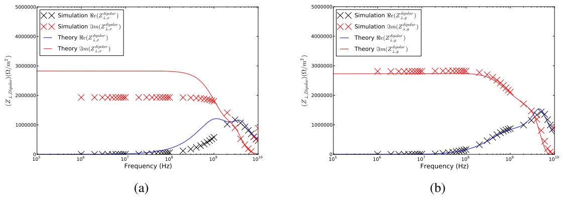
Figure 4.11: The dipolar impedance of two parallel ferrite plates simulated using two longitudinal coaxial wires. Presented are the impedances as measured in the horizontal plane ((a)) and in the vertical plane (b).
