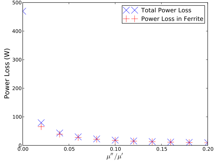
Figure 6.9: The power loss due to a beam with 1.15 \times 10^{11} particles per bunch, 288 bunches, a ring circumference 6911 m and a bunch length 4\sigma = 0.04 m assuming a Gaussian bunch distribution in the unscreened cavity.
