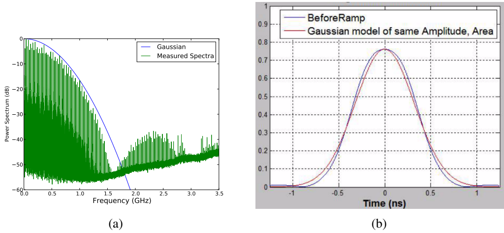
Figure 2.7: A comparison of (a) a measured beam power spectrum and a Gaussian bunch of the same bunch length in the frequency domain and (b) the resulting time domain beam profile. The Gaussian has a bunch length ( 4\sigma_z = 1.2 ns). Measured spectrum taken by P. Baundrenghien et al [32]. Time domain fit taken from E. Metral [33].
