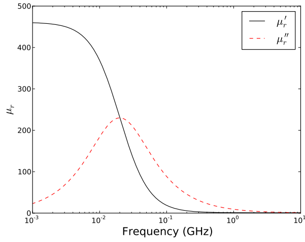
Figure 4.8: The complex permeability of 4A4 ferrite.
