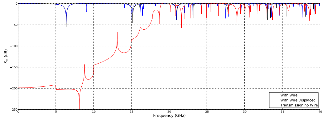
Figure 4.18: A comparison of the transmission parameters through a pillbox cavity with and without a coaxial wire. A displaced coaxial wire is also shown to illustrate the possibility of exciting dipolar modes also. It can be seen that the transmission signals are drastically changed depending on the presence or not of the wire.
