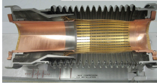
Figure 6.2: Example of RF fingers (in this case for the PIMS (Plug In ModuleS) module, placed between cryo-modules in the LHC).
