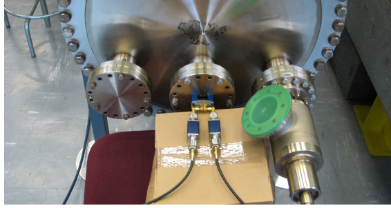
Figure 8.7: The measurement setup for the two wire measurement setup.
