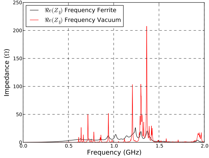
Figure 7.12: The real component of the longitudinal impedance for the TCTP collimator as simulated in the frequency domain for the case with and without ferrite damping tiles. The strong resonances present in the case without ferrite can be seen to be strongly damped when the ferrite tiles are added. However a substantial broadband component occurs in addition due to the broadened resonance peaks.
