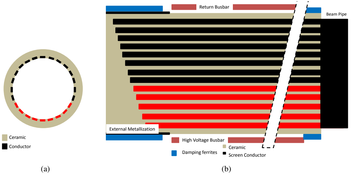
Figure 8.5: Cross sections of the beam screen perpendicular to (a) and parallel to (b) the direction of beam travel. The screen conductors removed from the majority of the MKIs during the original construction phase are highlighted in red.
