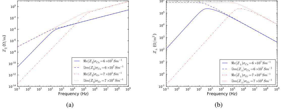
Figure 2.6: Examples of the longitudinal (a) and transverse (b) resistive wall impedance per unit length of a beam pipe of aperture a = 2 \text{ cm} made of either copper ( \sigma = 6 \times 10^7 \text{ Sm}^{-1} ) or graphite ( \sigma = 7 \times 10^4 \text{ Sm}^{-1} ).
