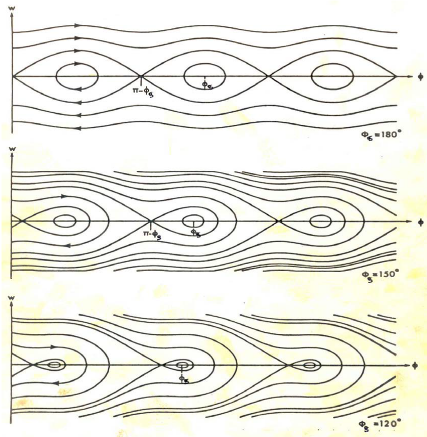
Figure A.2: The separatrix for different synchronous phase values. Note that the acceptance decreases as \phi_s \rightarrow \pi/2 . Taken from [121].
