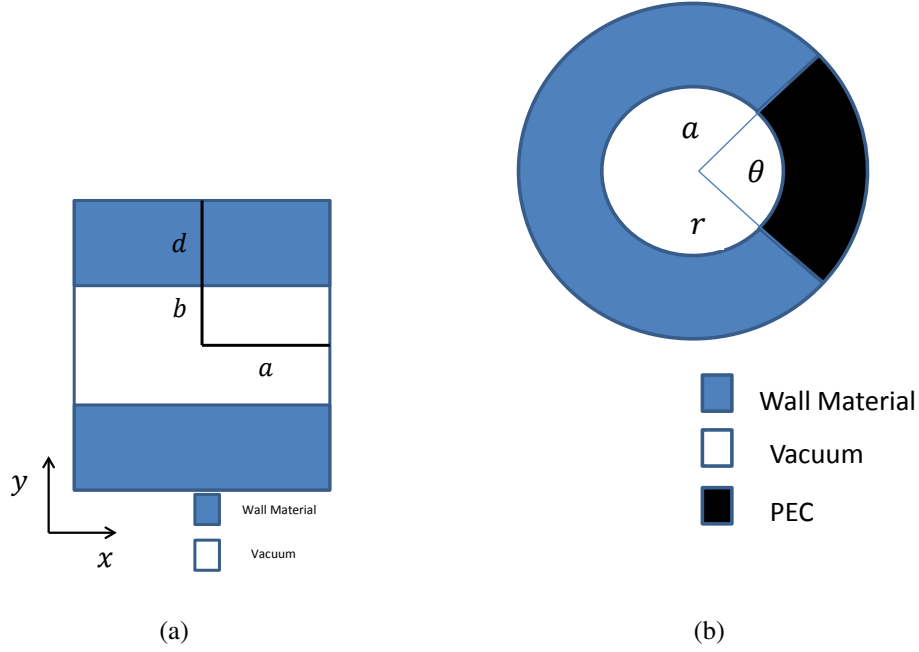
Figure 4.7: The geometries used for coaxial wire measurement simulations. For the geometry with top/bottom, left/right symmetry we use the Tsutsui model ((a)) using two parallel plates. For the asymmetric structure we use the Zannini-model for a C-core ferrite kicker magnet ((b)), which generates a constant term and a noticeable asymmetric term.
