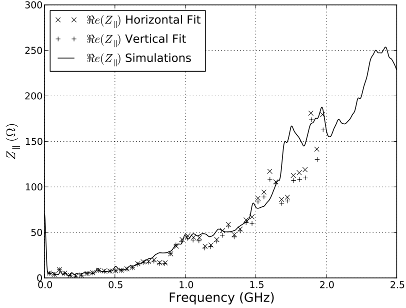
Figure 8.9: The real component of the longitudinal impedance of the LHC MKI acquired by measurements using the resonant coaxial wire method and time domain simulations using CST Particle Studio. (15 tapered screen conductors).
