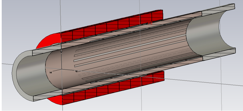
Figure 8.21: The cut down simulation model used for simulations of the MKI beam screen with 24 screen conductors.
