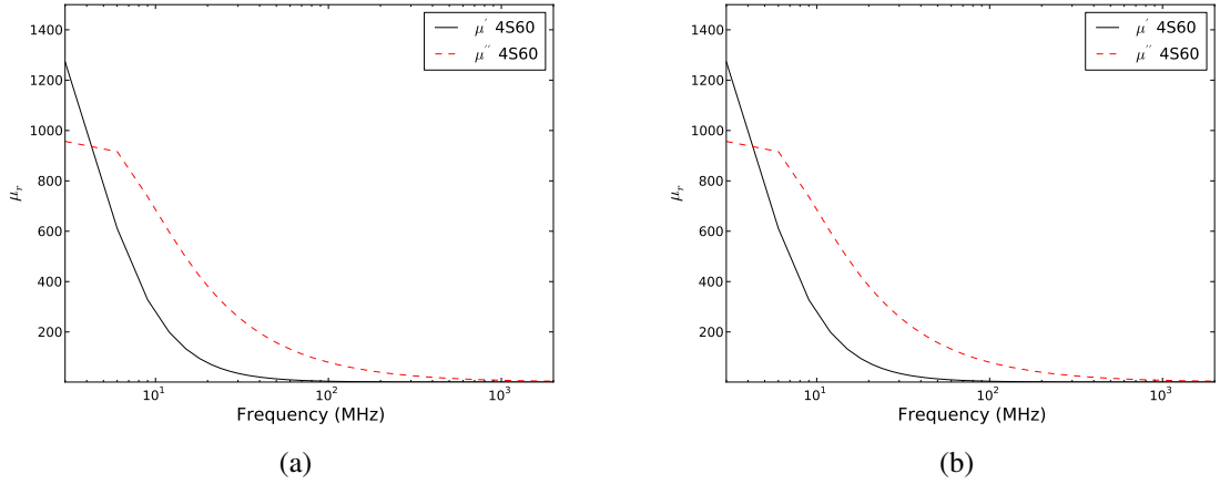
Figure E.2: The permeability (a) and penetration depth (b) for 4S60.
