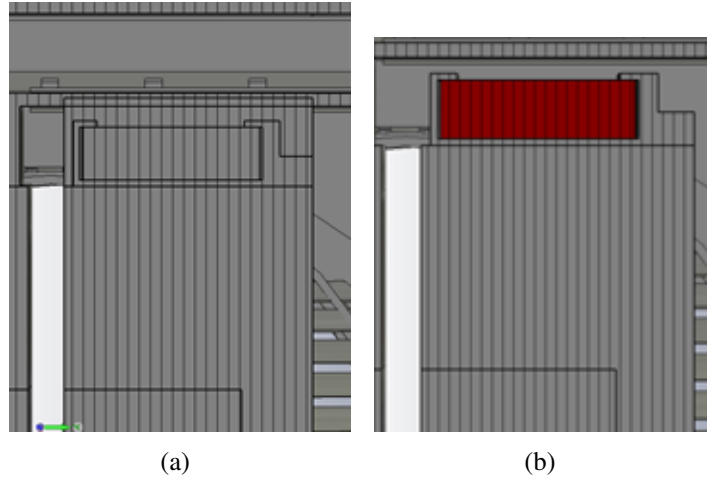
Figure 7.10: The different RF systems considered for the TCTP collimator. (a) shows an RF system similar to the phase 1 RF system. In these simulations the sliding RF contacts are replaced by a perfect connection - for frequencies lower than 2-3 GHz this is a good approximation and greatly simplifies the simulation model. (b) shows the RF circuit complete with ferrite. Two further variants may be considered, where the ferrite is replaced by either vacuum (to identify how the ferrite damps the otherwise present modes) and replacing the ferrite with PEC (to see whether it is the ferrite or the small aperture that reduces the coupling of the beam to the surrounding vacuum tank).
