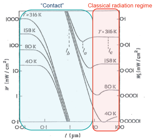
Figure F.2: An illustration of the change between the two regimes of thermal transfer by radiation and by conduction as the distance between two surfaces is reduced. It can be seen that there is a period between radiation and the beginning of transfer by contact where-in the rate of thermal transfer greatly increases. This is due to an effect known as radiative tunnelling [126].
