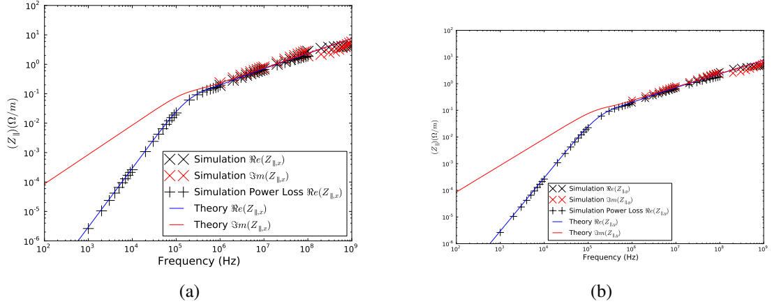
Figure 4.13: The longitudinal impedance of two parallel graphite plates as measured by taking the constant term of a quadratic equation fitted to a series of displaced single wire simulated measurements. Shown are simulated measurements acquired from fitting displacements in (a) horizontal axis and in (b) the vertical axis.
