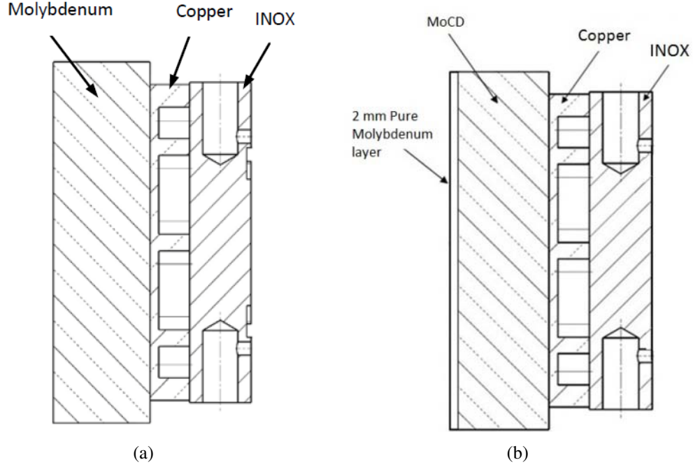
Figure 7.4: A number of the proposed jaw designs for the phase 2 secondary collimators. (a) shows the jaw made entirely from molybdenum. Glidcop may be substituted for molybdenum in this design. (b) shows the jaw made from a mixture of molybdenum diamond composite with a 2 mm coating of pure molybdenum on the surface. The composite ensures a mechanically strong jaw, whilst the coating screens the higher resistivity composite and provides a smooth surface on the beam-facing part of the jaw. In this case the composite may be substituted with copper diamond composite, and likewise the coating may be replaced with GlidCop.
