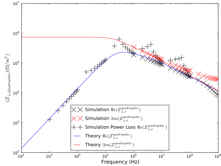
Figure 4.15: The quadrupolar impedance of two parallel graphite plates measured using a combination of displaced single wire measurements and two wire measurements.
