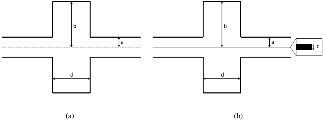
Figure 4.17: Comparison of the geometries of a cavity and attached beampipes (a) without and (b) with the coaxial wire in place. Note the dimensions and that the dashed line in (a) and the solid line in (b) represent the rotational plane of symmetry
