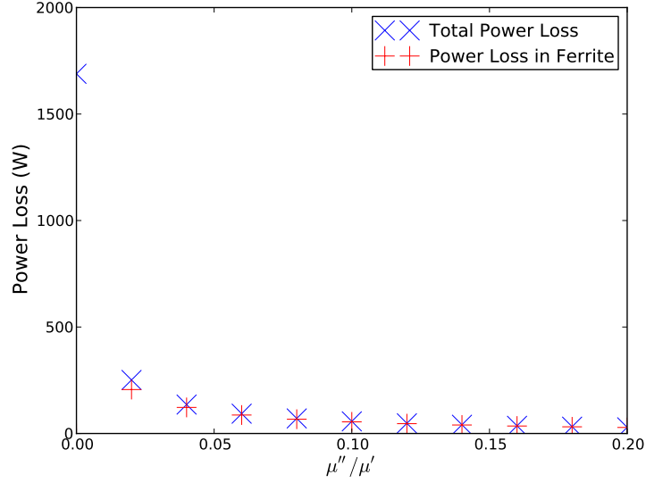
Figure 6.12: The power loss due to a beam with 1.15 \times 10^{11} particles per bunch, 288 bunches, a ring circumference 6911 m and a bunch length 4\sigma = 0.04 m assuming a Gaussian bunch distribution in the screened cavity.
