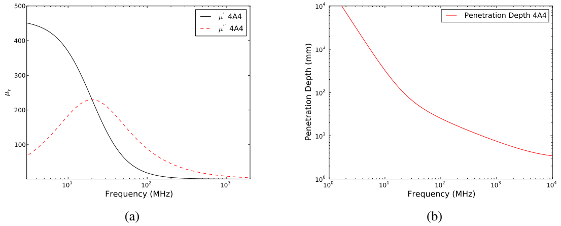
Figure E.3: The permeability (a) and penetration depth (b) for 4A4.
