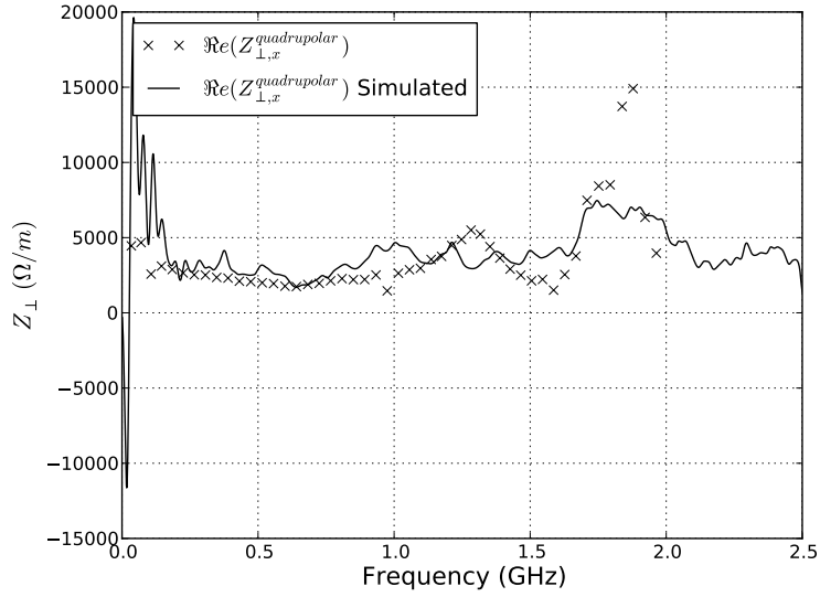
Figure 8.11: The real component of the quadrupolar impedances of the LHC MKI acquired by measurements using the resonant coaxial wire method and time domain simulations using CST Particle Studio. (15 tapered screen conductors).
