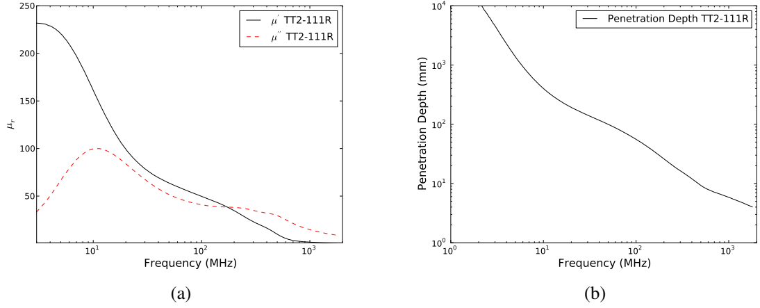
Figure E.1: The permeability (a) and penetration depth (b) for TT2-111R.
