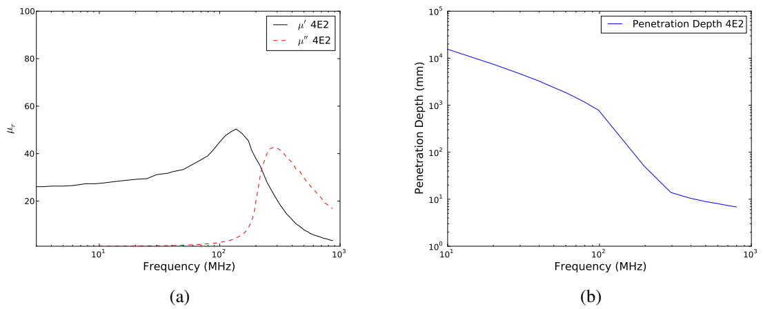
Figure E.4: The permeability (a) and penetration depth (b) for 4E2.
