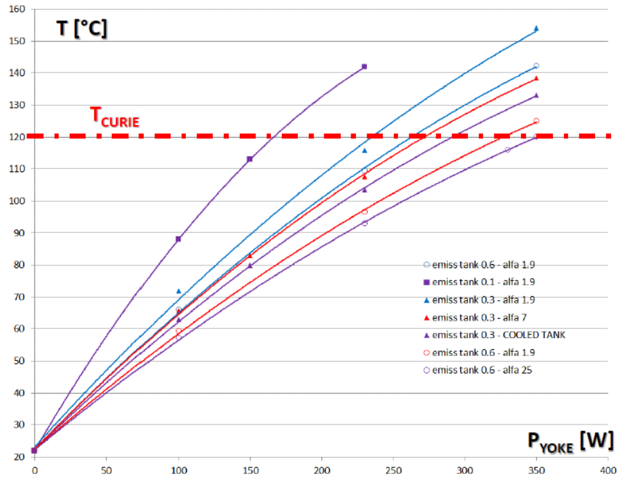
Figure 8.35: The maximum steady-state temperature reached by the ferrite yoke in the MKI depending on the power load in the ferrite yoke as calculated using a 2D cross section of the MKI assuming different tank emissivities and rates of convection outside of the tank ( \alpha ). P_{yoke} is the power lost in the ferrite yoke and T the maximum steady state temperature of the ferrite yoke. Provided by M. Garlasche et al [118]. The worst case scenario is for \alpha=1.9 W/(m² K).
