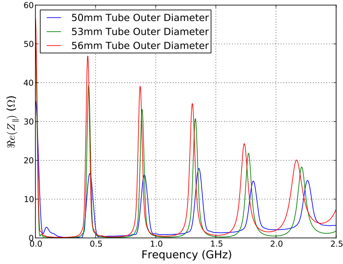
Figure 8.25: The variance of the real beam coupling impedance with the tube thickness. External diameters of 50, 53 and 56mm correspond to tube thicknesses of 4, 5.5 and 7mm respectively. The physical overlap is 100mm in all cases.
