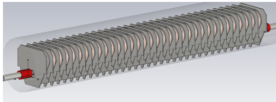
Figure 8.8: The simulation model of the LHC injection kickers implemented in CST Particle Studio.
