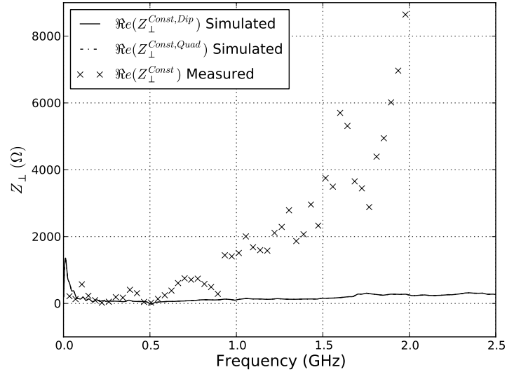
Figure 8.12: The real component of the constant transverse impedances of the LHC MKI acquired by measurements using the resonant coaxial wire method and time domain simulations using CST Particle Studio. The simulated results from taking the displaced source signal and the displaced witness signal lie on top of one another. (15 tapered screen conductors).
