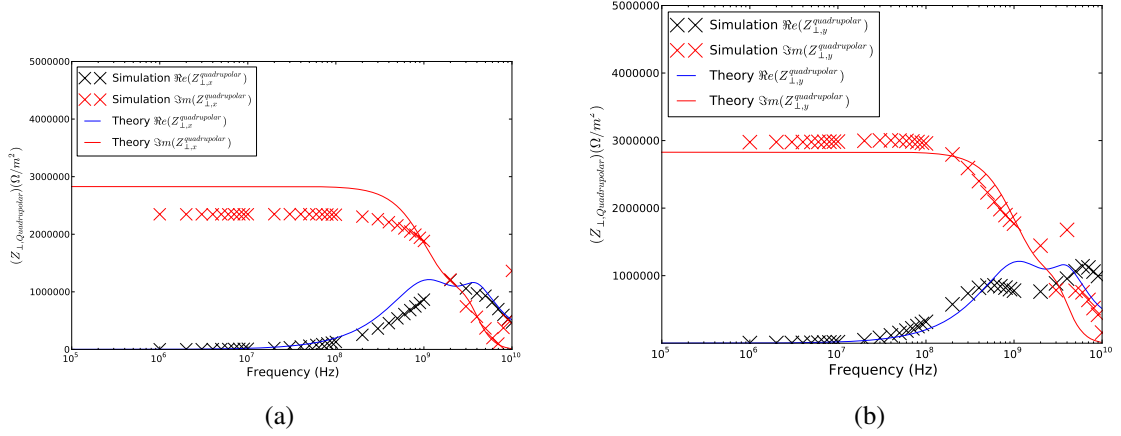
Figure 4.12: The quadrupolar impedance of two parallel ferrite plates simulated using a combination of displaced single wire simulated measurements and two wire simulated measurements. Presented is the impedance as measured in the horizontal plane ((a)) and in the vertical plane (b).
