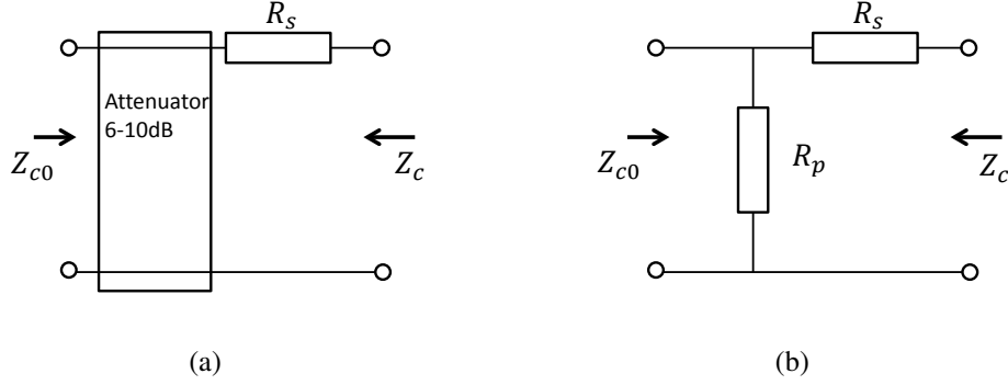
Figure 4.2: The resistive networks for matching a DUT to the attached measuring network (VNA and connecting cables). (a) shows series resistive matching and (b) shows a two way matching network.
