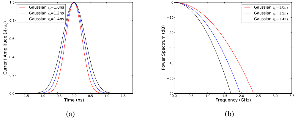
Figure 2.10: (a) The longitudinal profile and the (b) associated bunch power spectrum for a number of bunch lengths assuming a Gaussian bunch profile.
