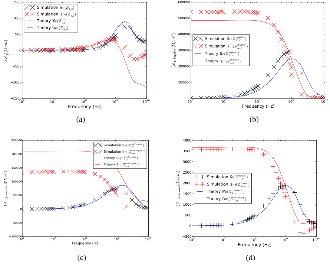
Figure 4.16: The impedance of the C-core ferrite kicker as acquired by simulating the classical coaxial wire method in HFSS. Shown is the (a) longitudinal impedance, (b) the dipolar impedance, (c) the quadrupolar impedance and (d) the constant transverse impedance.
