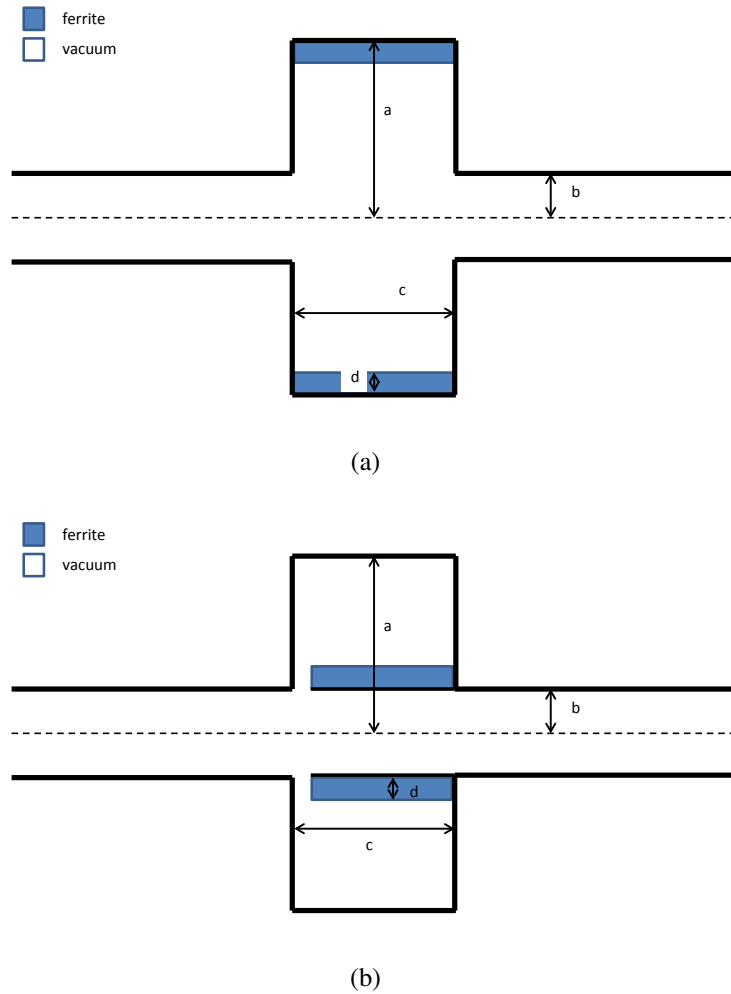
Figure 6.6: Two sample geometries used to examine the effects of ferrite damping material on cavity resonances. (a) shows a cavity with the ferrite unshielded, and (b) shows a more realistic case in which the ferrite is shielded from directly seeing the traversing beam.
