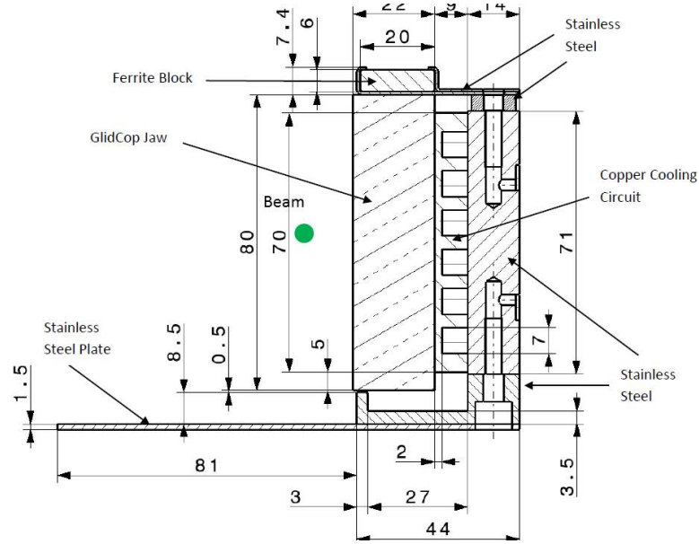
Figure 7.3: The RF system for use in the phase 2 collimation system. The sliding RF contacts of the phase 1 design are replaced with a ferrite damping system. The RF contacts are removed, allowing the beam to see the entire RF cavity, causing resonances at lower frequencies. The Q of these resonances are decreased by the use of ferrite damping tiles (see Sec. 6.6). The location of the beam is shown in green.
