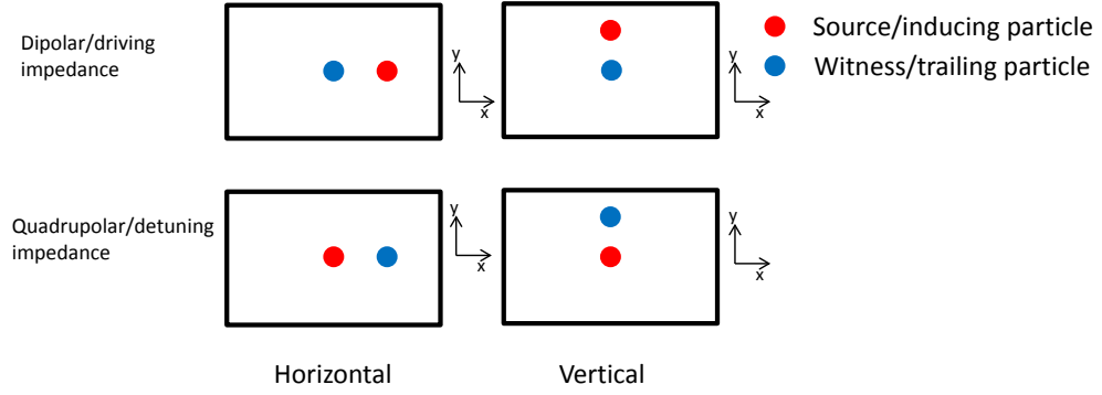
Figure 2.2: The relative displacements of the source particle and witness particle in the horizontal and vertical planes that identify the dipolar/driving and quadrupolar/detuning impedances.
