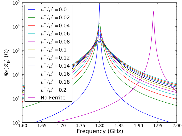
Figure 6.7: The real component of the longitudinal beam coupling impedance of a cavity without and with a damping material with \epsilon' = 10 , \mu' = 10 and \mu''/\mu' is varied. The non-damped cavity is shown for comparison. The change in resonant frequency and shunt impedance is due to the increased \epsilon' of the damping material.
