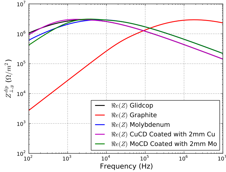
Figure 7.8: The real component of the vertical dipolar impedance of the various collimator jaw materials assuming a 2mm half gap.
