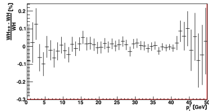
(b) pp \rightarrow W^+ + X \rightarrow e^+ \nu_e + X
