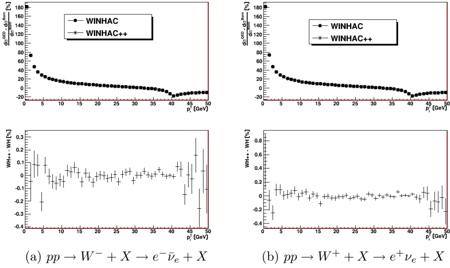
Fig. 3. Distributions of the transverse momentum of the electron (a) and the positron (b) from W decays for the relative QED corrections.
