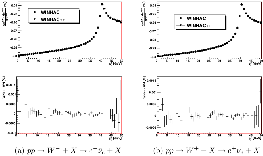
Fig. 4. Distributions of the transverse momentum of the electron (a) and the positron (b) from W decays for the relative electroweak corrections.
