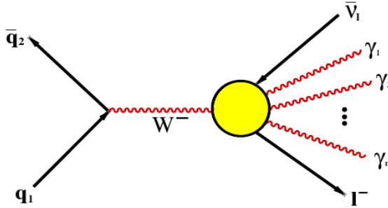
Fig. 1. Multiphoton radiation in W decay [3].
