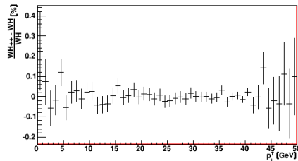
(a) pp \rightarrow W^- + X \rightarrow e^- \bar{\nu}_e + X
