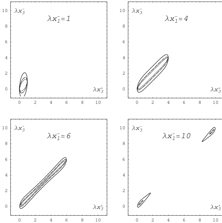
Fig. 1. The non-local Hamiltonian density is drawn on the LF in terms of contours of constant value of the function |\lambda(x_1 - x_2)^\perp h(x_1, x_2, x_3)| in Eq. (32) for \lambda \gg m for 4 different distances between x_1 and x_2 . Continuous contour line corresponds to 0.1, dashed line to 0.3, and dotted line to 0.6. x_3 lies on the 2-dimensional space-time plane containing x_1^\perp - x_2^\perp . In all four panels \lambda x_2 = 0 while \lambda x_1^- = \lambda |x_1^\perp| = 1, 4, 6 , and 10 , as shown. The contours show that point x_3 of annihilation of one effective particle must lie in the vicinity of a line that connects the two points x_1 and x_2 of creation of two effective particles. This figure corresponds to Fig. 2 in Ref. [4]. See the text for more details.
