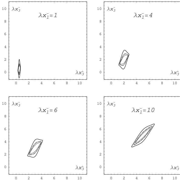
Fig. 3. The same result as in Fig. 1 but for \lambda = m and multiplied in addition by 6e^9 in order to remove the suppression that the vertex form factor implies for \lambda \sim m . This figure corresponds to Fig. 5 in Ref. [4]. See the text for further details.
