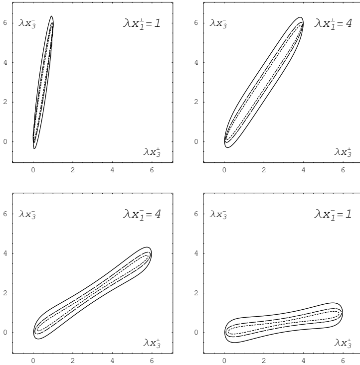
Fig. 2. Changes in the contour pattern drawn in precisely the same case and in the same convention as in Fig. 1 but for different choices of x_1 on the LF: \lambda(|x_1^\perp|, x^-) = (1, 6), (4, 6), (6, 4) , and (6, 1) , as indicated. The contours show the same relativistic pattern of x_3 lying in a vicinity of the line that connects x_1 and x_2 on the LF. This figure corresponds to Fig. 3 in Ref. [4]. See the text for more explanation.
