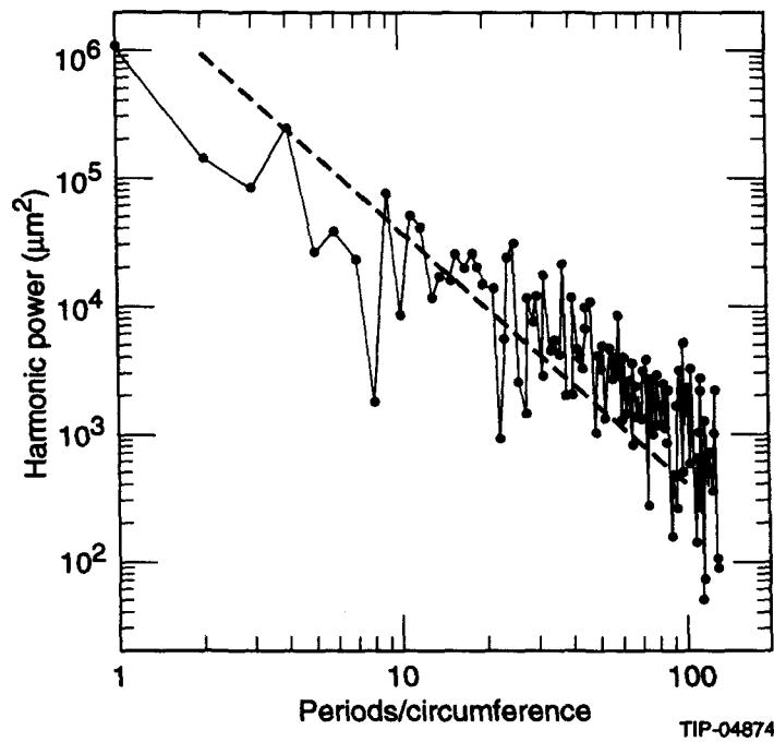
Figure 3. Spectrum of space harmonics found by Fourier transformation of primary 1988 data (i.e., FFT of Figure 1(b)).
