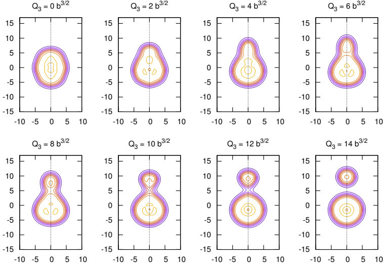
Fig. 3. Evolution of the shape of ^{114}\text{Ba} along the asymmetric fission path. Equidensity lines are plotted every 0.02 \text{ fm}^{-3} .
