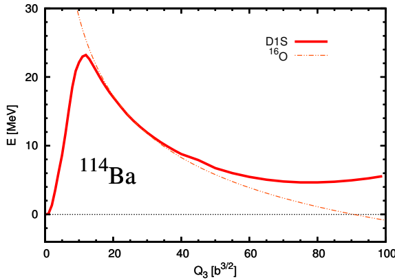
Fig. 2. Asymmetric fission barrier in ^{114}\text{Ba} as function of the octupole moment Q_3 . The thin dashed line corresponds to the classical Coulomb energy of two fragments ^{16}\text{O} and ^{98}\text{Cd} .
