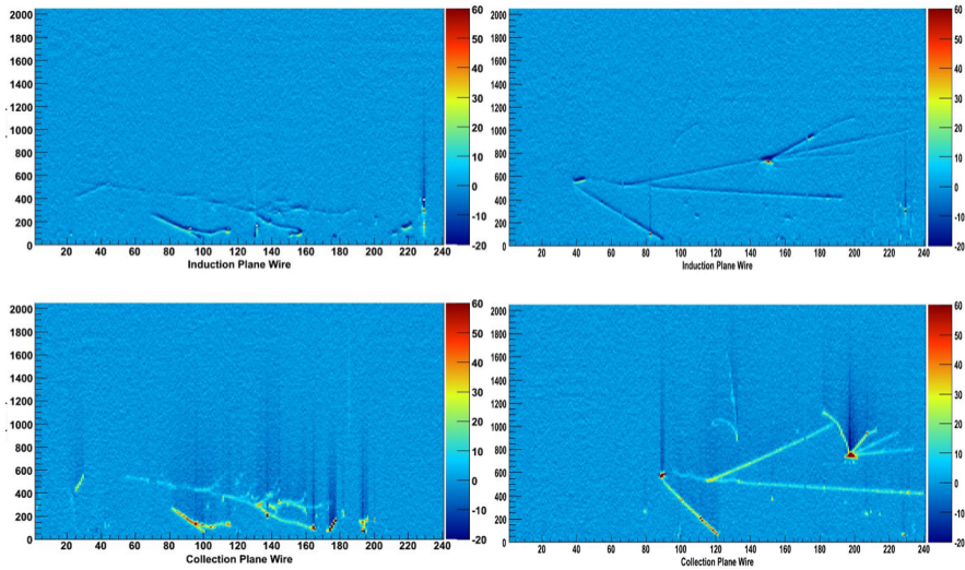
Fig. 2. Example of 2D (raw) images of \nu_\mu events from the two LAr TPC wire planes, collected with ArgoNeuT during the first neutrino run at NuMI-FNAL (May–June, 2009).
