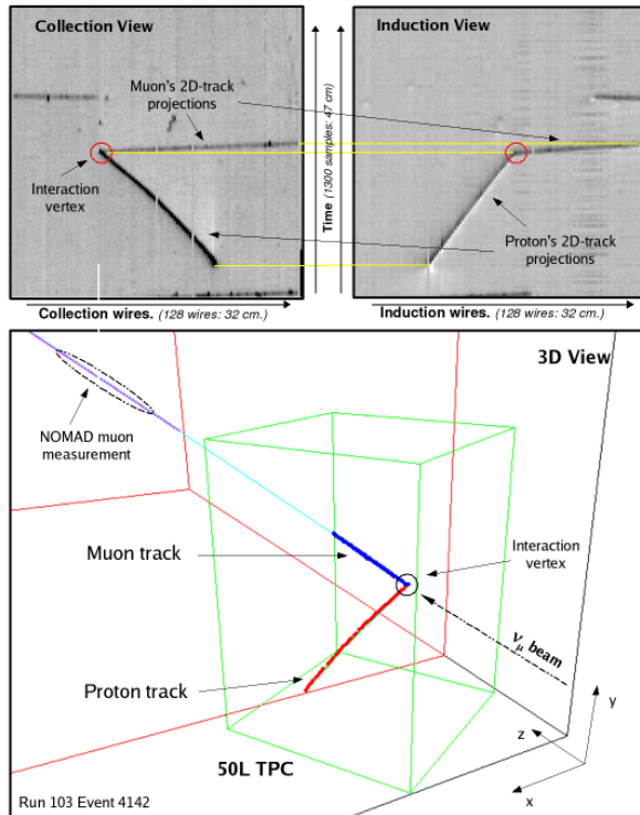
Fig. 1. Example of the 3D reconstruction of a low-multiplicity (QE) \nu_\mu CC event. The raw image from the two TPC wire planes (top): Hits and 2D track projections have been identified. Three dimensional view of the reconstructed event (bottom).
