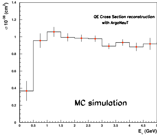
Fig. 3. MC simulation of QE cross-section reconstruction with ArgoNeuT.
