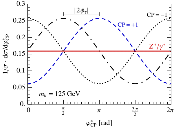
Figure 1: Normalized \varphi_{CP}^* distribution for pp \rightarrow h/Z^*/\gamma^* \rightarrow \tau^+\tau^- production at the LHC ( \sqrt{S} = 14 TeV) with subsequent \tau^\pm \rightarrow \pi^\pm + \nu_\tau/\bar{\nu}_\tau decay. The distribution for a CP -even ( CP -odd) Higgs boson is shown by the blue dashed line (black dotted line). For a Higgs boson of CP mixture with \phi_\tau = -\frac{\pi}{4} the distribution is given by the black long-dash dotted line. The distribution for the Drell-Yan background is shown by the solid red line.
