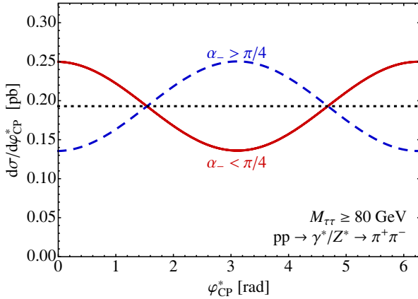
Figure 2: Drell-Yan production of \tau^+\tau^- at the LHC ( \sqrt{S} = 14 TeV, M_{\tau\tau} \geq 80 GeV, |\eta_{\pi^\pm}| \leq 1 ) with subsequent \tau^\pm \rightarrow \pi^\pm + \nu_\tau/\bar{\nu}_\tau decay. Events are split into two categories with \pi^- ‘nearly coplanar’ ( \alpha_- < \pi/4 , red solid line) and events with \pi^- ‘nearly perpendicular’ ( \alpha_- > \pi/4 , dashed blue line) to the q\tau production plane. The dotted black line indicates the sum of the two distributions divided by two.
