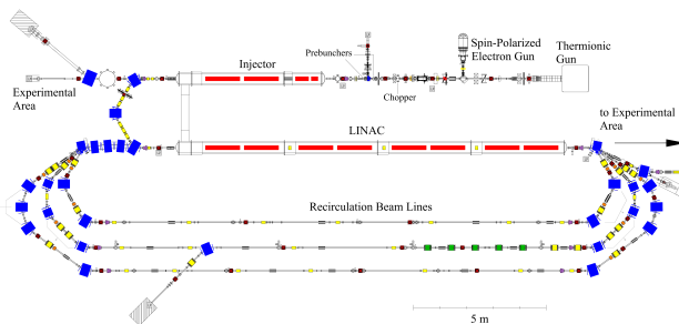
Figure 1: Current layout of the S-DALINAC.
