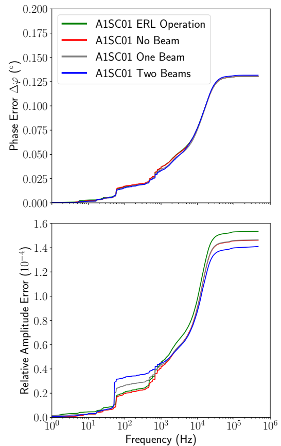
Figure 4: Integrated Fourier spectra of phase and relative amplitude errors of the rf control system during the four different operation modes for the first main accelerator cavity A1SC01 [4]. The total rms errors are corresponding to the maximum values. The similarity of the different spectra curves and maximum values shows that the stability of the rf control system is sufficient to be operated in energy recovery mode at 1 \mu A beam current.
