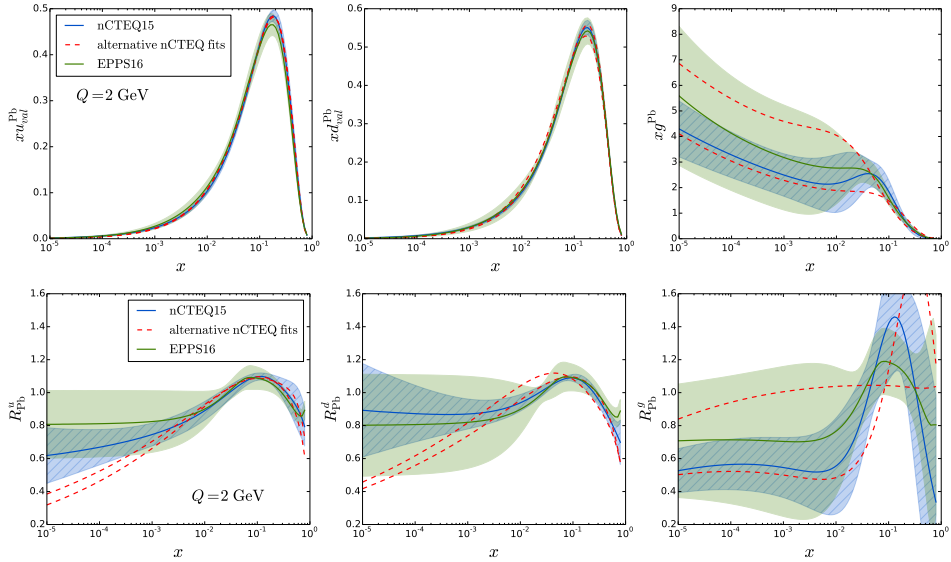
Fig. 2: (Color online) Comparison of lead nuclear nPDFs (upper plot) and a corresponding nuclear ratio, R_i^{\text{Pb}} = f_i^{\text{Pb}}/f_i^{\text{free-proton}} (lower plot), from nCTEQ15 [7] and EPPS16 [3] nPDF global analyses. The dashed/red curves represent alternative nCTEQ fits aiming at a more realistic representation of the gluon uncertainty [8].
