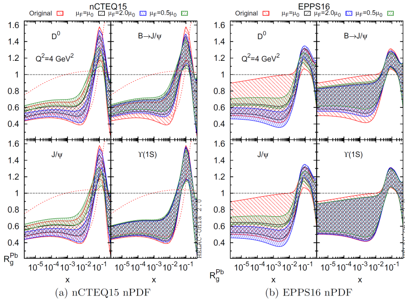
Fig. 4: (Color online) NPdf uncertainties for (a) nCTEQ15 and (b) EPPS16 after the reweighting.
