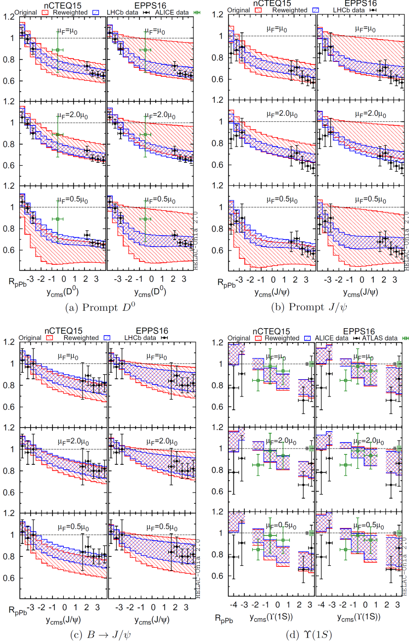
Fig. 3: (Color online) Selected R_{pPb} results before and after reweighting for (a) prompt D^0 , (b) prompt J/\psi , (c) B \rightarrow J/\psi , (d) \Upsilon(1S) . The experimental data are from [38, 44, 50, 82, 83].
