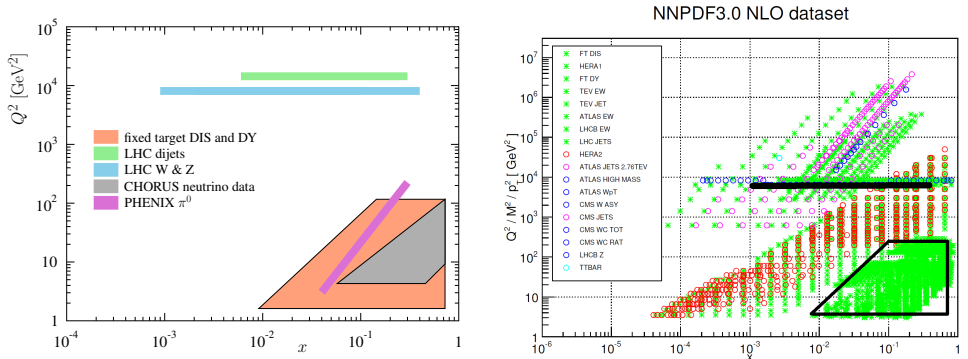
Fig. 1: Left: Kinematical range of data used in the most recent EPPS16 nPDF global analysis [3]. Right: Example kinematical range of data used in free-proton PDF global analysis NNP3.0 [4] (black lines correspond to nuclear data).
