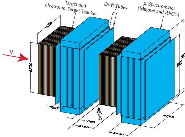
Fig. 2. The schematic view of the OPERA detector.
