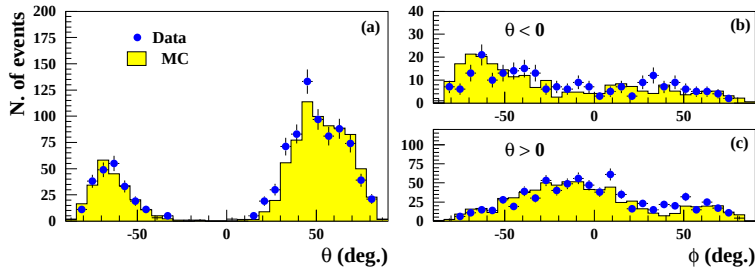
Fig. 5. Angular distributions of underground muons, measured with 4 spectrometer planes. Angles correspond to the slopes of the muon track (a) in the vertical and (b),(c) horizontal projections. \theta = 0 corresponds to the zenith direction.
