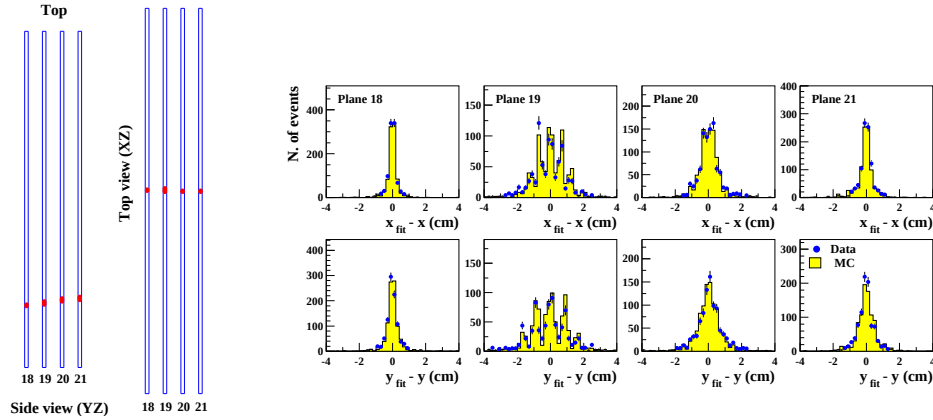
Fig. 4. An example of a single \mu event observed with the last 4 spectrometer planes (left). Residuals of the straight line fit to deposits in planes 18, 20, 21 (right).
