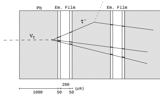
Fig. 1. The schematic structure of an ECC cell with the \nu_\tau CC interaction.
