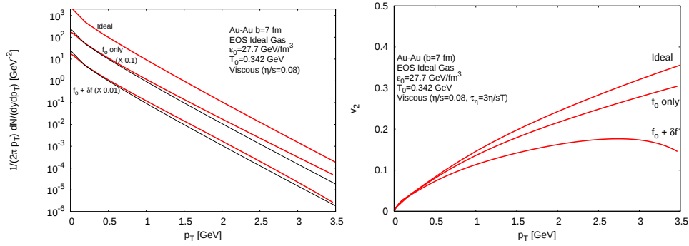
Fig. 1. Effect of shear viscosity on p_{\perp} spectra (left) and v_2(p_{\perp}) (right) of massless particles. The thin black curves in the left plot show the rescaled ideal result for comparison to the viscous result.
