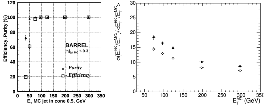
Fig. 5. (left) Jet reconstruction efficiency and purity using the barrel calorimeters for PYTHIA generated jets embedded in a Pb+Pb heavy ion background with dN_{\text{ch}}/dy|_{y=0} \approx 5000 , which is above the maximum expected at \sqrt{s_{NN}}=5.5 TeV. (Right) Jet transverse energy resolution determined for the same Pb+Pb heavy ion collisions (closed symbols) compared to proton+proton (open symbols).
