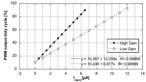
Figure 3: Dynamic and linearity of the amplifier for the two available gains.
