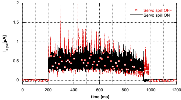
Figure 5: Servo-Spill intensity time profile for Protons with energy 90 mm W.E. (110.96 MeV/u).
