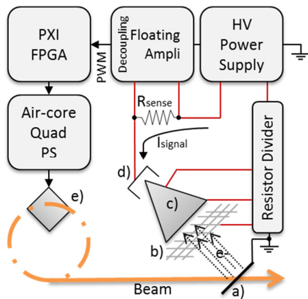
Figure 2: FIM servo-spill block diagram; a) is the thin foil, b) the grid, c) the CEM, d) the electrons collector, e) the fast quadrupole.
