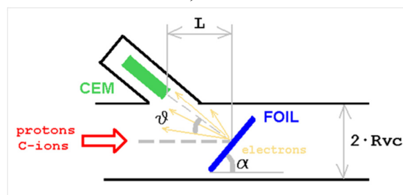
Figure 1: FIM detector mechanical layout; R_{vc} (33 mm) is vacuum chamber radius, L is 42mm.
