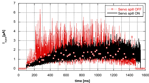
Figure 6: Servo-Spill intensity time profile for Carbon Ions with energy of 90 mm W.E. (208.57 MeV/u).
