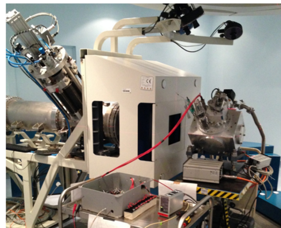
Figure 4: FIM installation after the dose delivery system, for its commissioning with beam.
