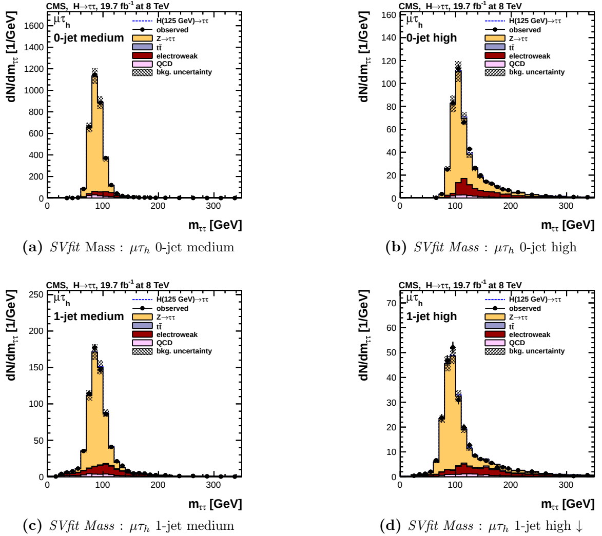
Figure 7.31: Di- \tau mass distribution for the categories used in the Standard Model analysis in the \mu\tau_h channel after the maximum likelihood fit is performed.
