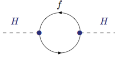
Figure 1.8: One loop fermion contribution to the Higgs boson mass [66].
