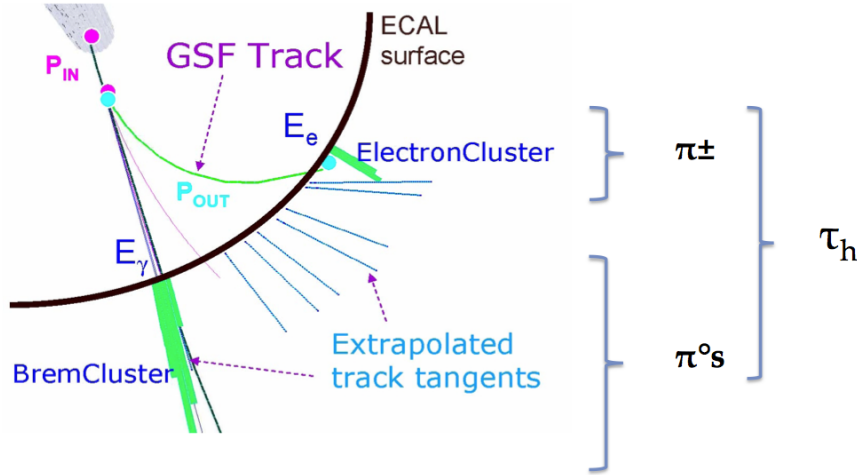
Figure 5.1: Electron mis-reconstructed as a 1-prong \tau_h .
