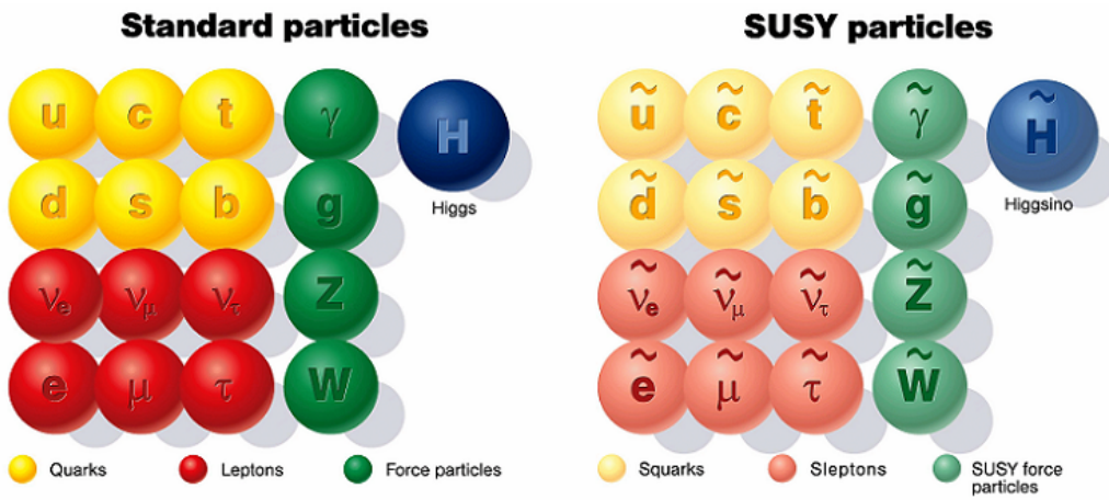
Figure 1.9: Standard Model particles and their supersymmetric partners.
