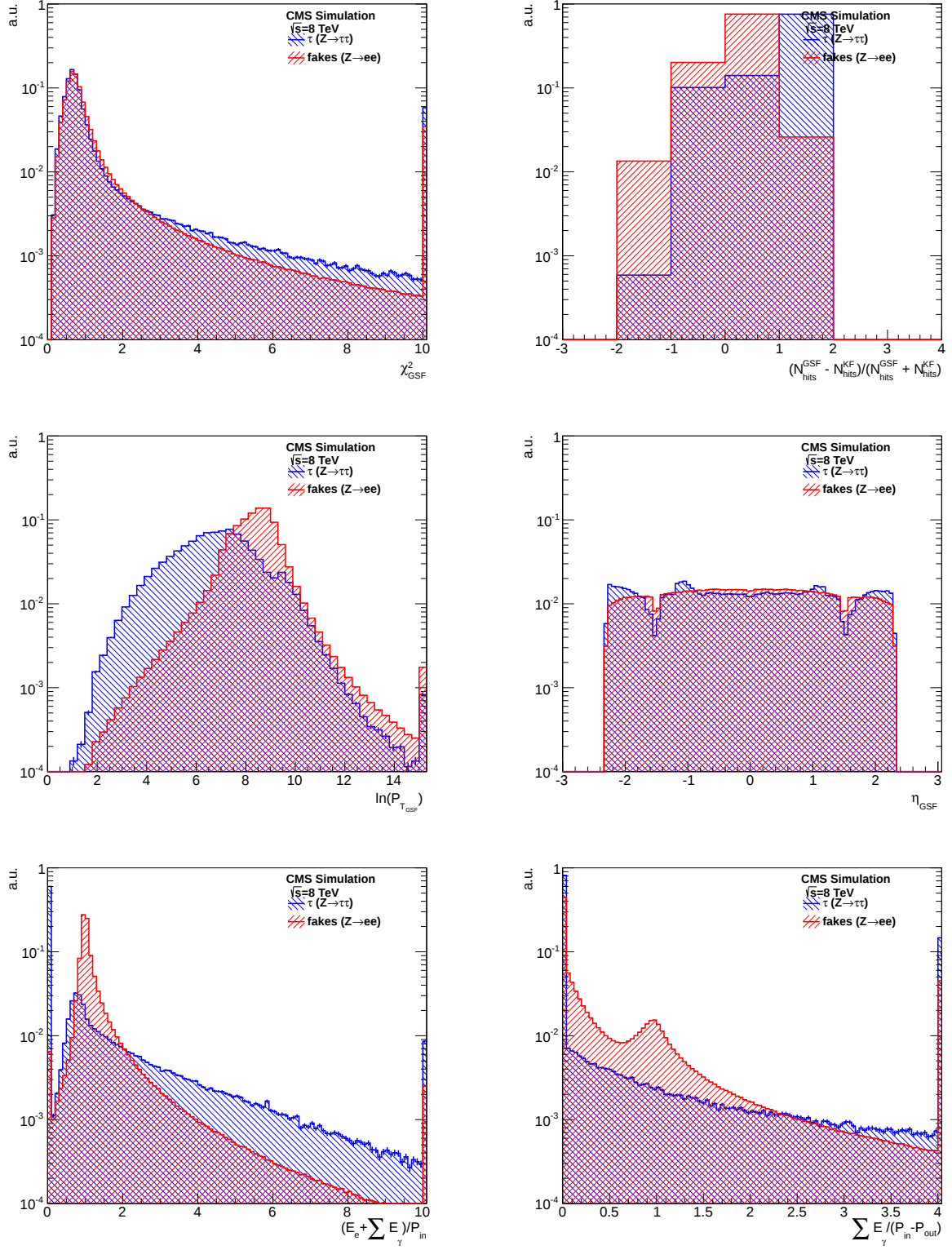
Figure 5.5: Input variables distributions described in the text, normalized to unity, for the MVA based anti- e discriminator for simulated signal and background Z/\gamma^* \rightarrow \tau\tau (blue) and Z/\gamma^* \rightarrow ee (red) events respectively.
