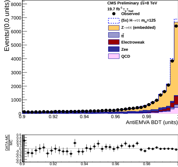
Figure 5.8: BDT output of the anti-electron discriminator.
