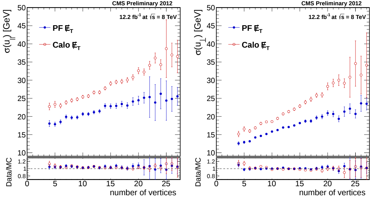
Figure 3.23: Parallel (left) and perpendicular (right) recoil component resolution for the PF \vec{E}_T and Calo \vec{E}_T algorithms as a function of the number of reconstructed vertices for Z \rightarrow \mu\mu events. From [137].
