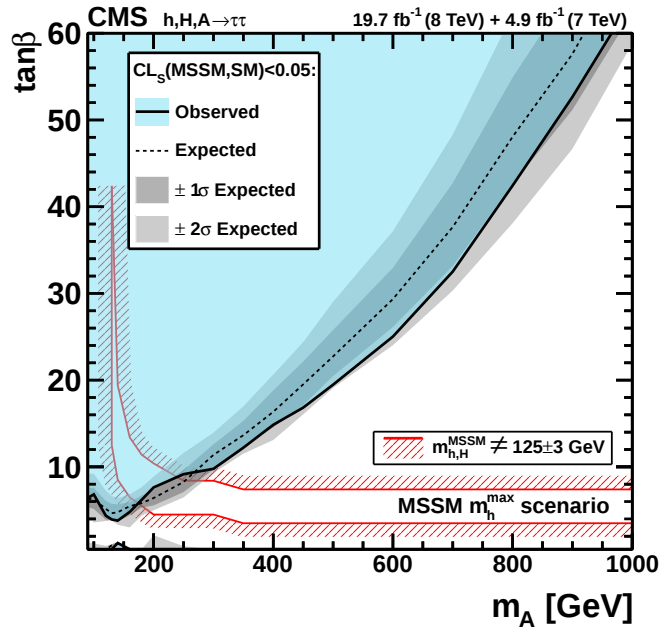
Figure 2.22: MSSM vs SM limit in the MSSM m_h^{\max} scenario. At each (m_A - \tan\beta) point a Hypothesis test is performed testing the MSSM ( A+H+h+\text{BKG} ) hypothesis against the SM ( h\text{SM}+\text{BKG} ) hypothesis. From Ref. [108].
