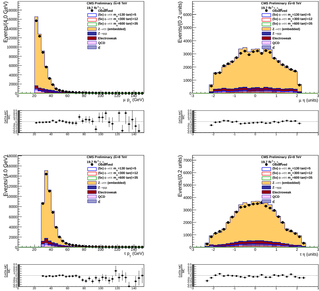
Figure C.1: Distribution of the muon (up) and \tau_h (bottom) transverse momenta (left) and \eta (right) in the \mu\tau_h channel after the baseline selection.
