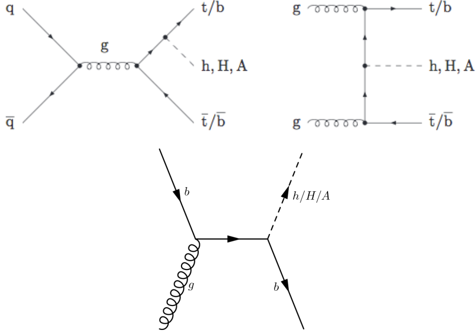
Figure 2.17: Main Feynman diagrams at leading order for the heavy quark associated production mode: gg/q\bar{q} \rightarrow Q\bar{Q} + h/H/A (up), gb \rightarrow b + h/H/A (down).
