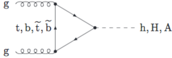
Figure 2.16: Main Feynman diagram at leading order for the gluon fusion ( gg \rightarrow h/H/A ) production mode.
