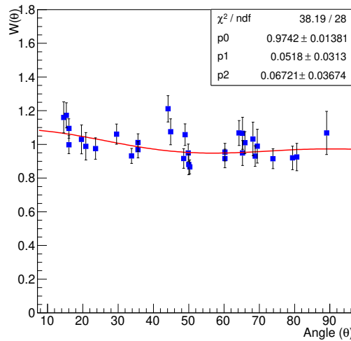
Fig. 5. Preliminary results of the measured angular correlation intensities W(\theta) of the 151–245 keV cascade in ^{111}\text{Cd} , for a quarter of all possible angles of the iThemba LABS segmented clover detector, because for low-energy \gamma rays, only the front segments are sensitive. The uncertainties on the data points represent the statistical errors on the measured areas. The coefficients p_0 , p_1 and p_2 represent the measured values of the parameters A_0 , a_2 and a_4 , respectively.
