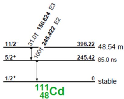
Fig. 2. Partial level scheme of ^{111}\text{Cd} [6].
