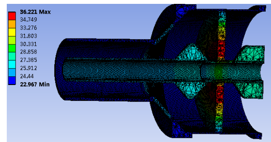
Figure 5: Thermal Simulation in ANSYS.
