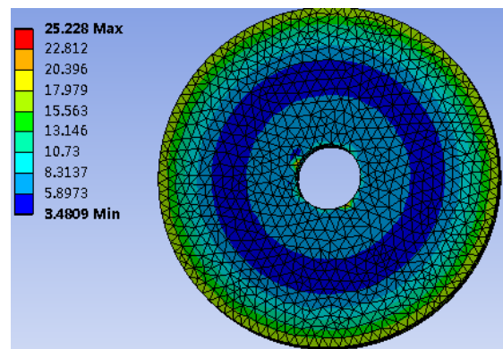
Figure 6: Thermal stress on the ceramic surface.
