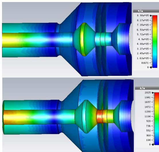
Figure 4: Electromagnetic field simulation by CST. Upper is electric, lower is magnetic field.
