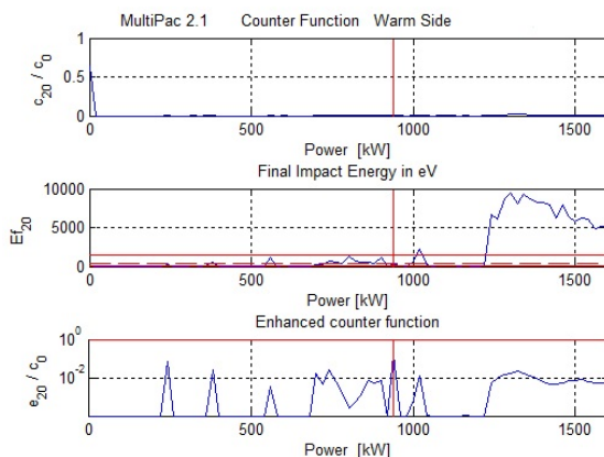
Figure 7: Secondary electron emission on the ceramic with 5 nm TiN coating simulation result in multipacting.
