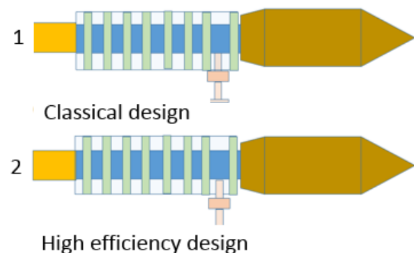
Figure 1: Klystron development strategy.
