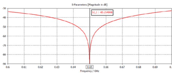
Figure 3: Return loss (S11) and insert loss (S21).
