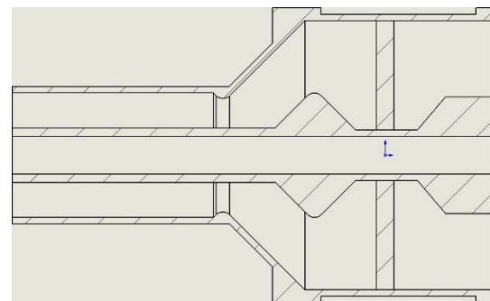
Figure 2: Schematic drawing of CEPC klystron output window.
