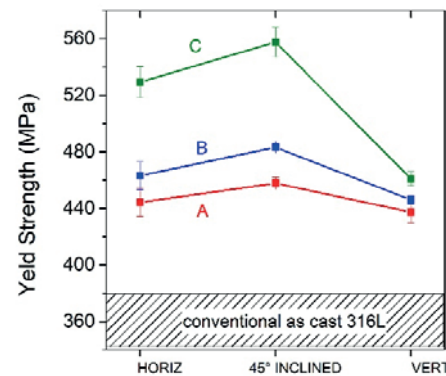
Figure 4: Yield strength determined on AM 316L tensile test specimens from different manufacturers (A, B, C), for horizontal, vertical and 45^\circ inclined growth with respect to the build plate and comparison with the one of as cast counterparts [1].
