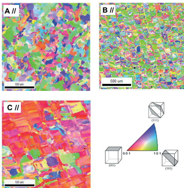
Figure 3: EBSD images for AM 316L samples, side parallel to the build plate, from different manufacturers (A, B and C) and standard stereographic triangle.
