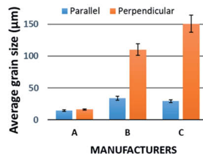
Figure 2: Average grain size for samples produced by different manufacturers and for two different orientations: parallel or perpendicular to the build plate.
