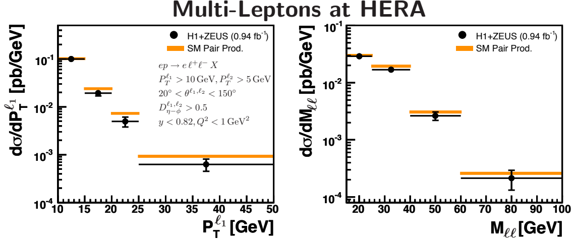
Figure 1: The cross section for lepton-pair photoproduction in a restricted phase space as a function of the leading lepton transverse momentum P_T^{l1} (a) and the invariant mass of the lepton pair M_{ll} (b). The total error bars are shown, representing the statistical and systematic uncertainties added in quadrature. The bands represent the uncertainty in the SM prediction.
