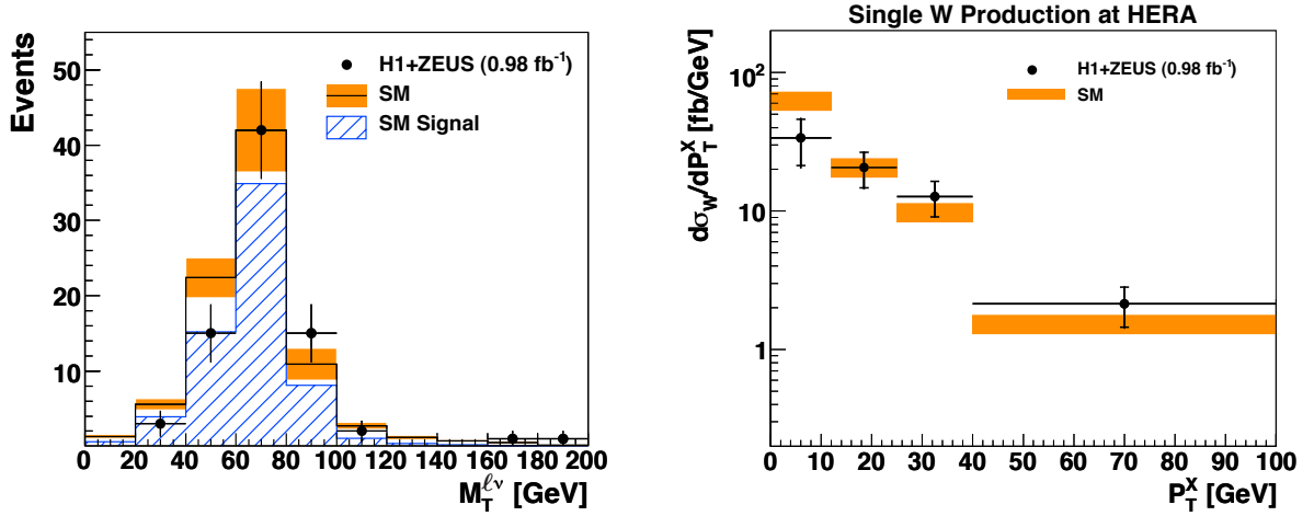
Figure 2: Left: The lepton-neutrino transverse mass M_{l\nu} of events with an isolated electron or muon and missing transverse momentum. The data (points) are compared to the SM expectation (open histogram). The signal component of the SM expectation, dominated by single W production, is shown as the striped histogram. The total uncertainty on the SM expectation is shown as the shaded band. Right: The single W production cross section as a function of the hadronic transverse momentum, P_T^X . The inner error bar represents the statistical error and the outer error bar indicates the statistical and systematic uncertainties added in quadrature. The shaded band represents the uncertainty on the SM prediction.
