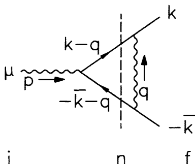
Fig. 3. Application of Cutkosky's rule to the Bf\bar{f} vertex form factor induced by the exchange of B between the two fermion legs.
