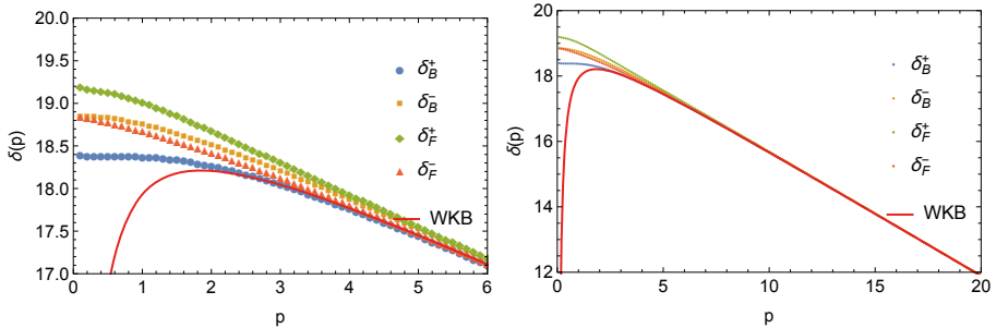
Figure 5.1. Numerical results for the phaseshifts.
