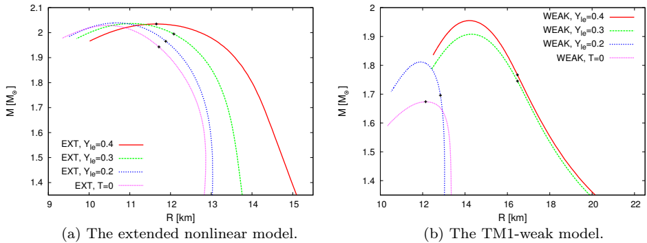
Fig. 4. The M-R relations calculated for different stages of neutron star evolution for the value of parameter \Lambda_V = 0.0165 in the case of hyperon-rich matter. Black points illustrate the evolutionary path of chosen neutron star configurations.
