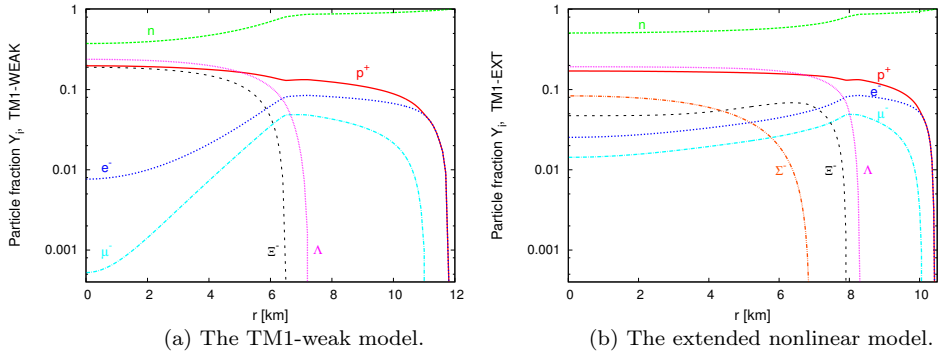
Fig. 3. The radial dependence of the particle fractions Y_i = n_i/n_b obtained for the maximum mass configurations. Calculations have been done for parameter \Lambda_V = 0.0165 in the case of the TM1-weak and extended nonlinear models.
