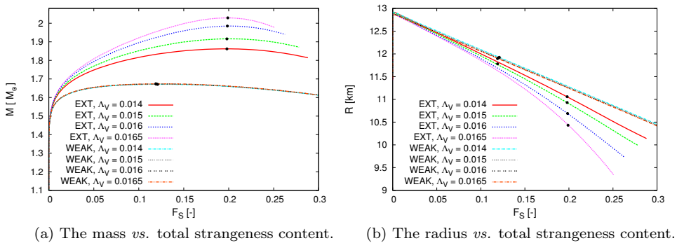
Fig. 2. The mass and radius as a function of the total strangeness content of system calculated for hyperon-rich neutron star matter. Calculations were done for different values of parameter \Lambda_V . Black dots represent the maximum mass configurations for considered models.
