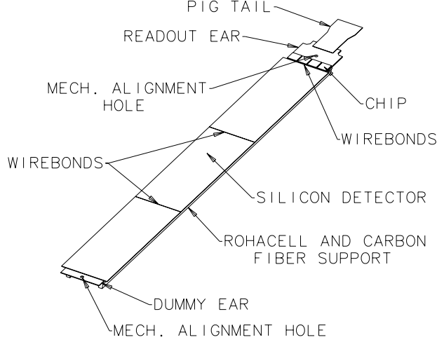
Figure 3.4: SVX ladder.
