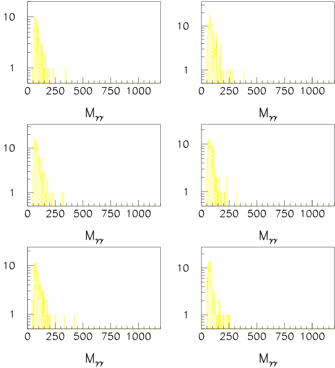
Figure 6.10: Invariant mass distribution for pseudoexperiments in absence of extra dimensions ( \eta = 0 ).
