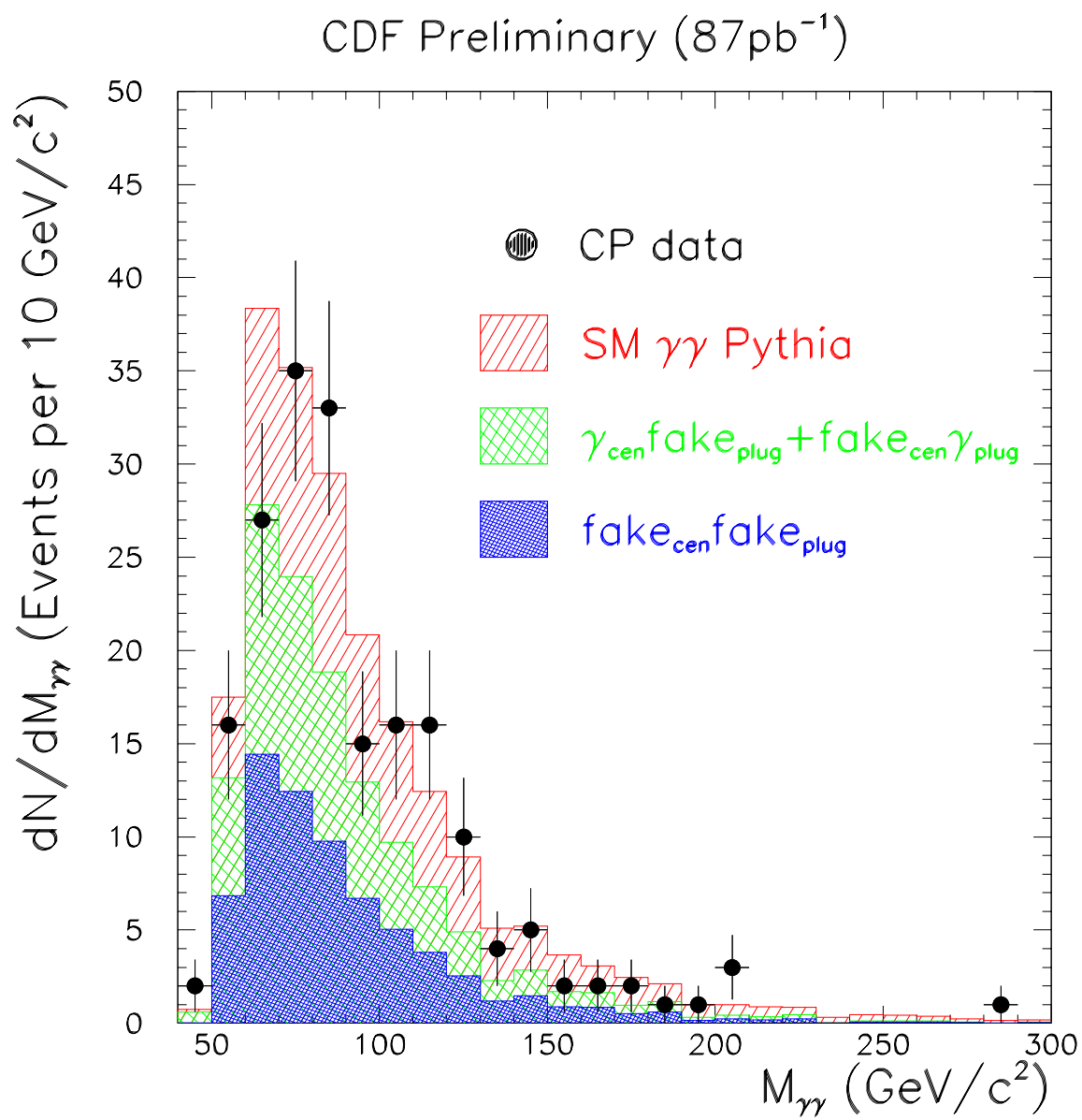
Figure 5.7: SM \gamma\gamma and fake contributions in the Central-Plug diphoton sample.
