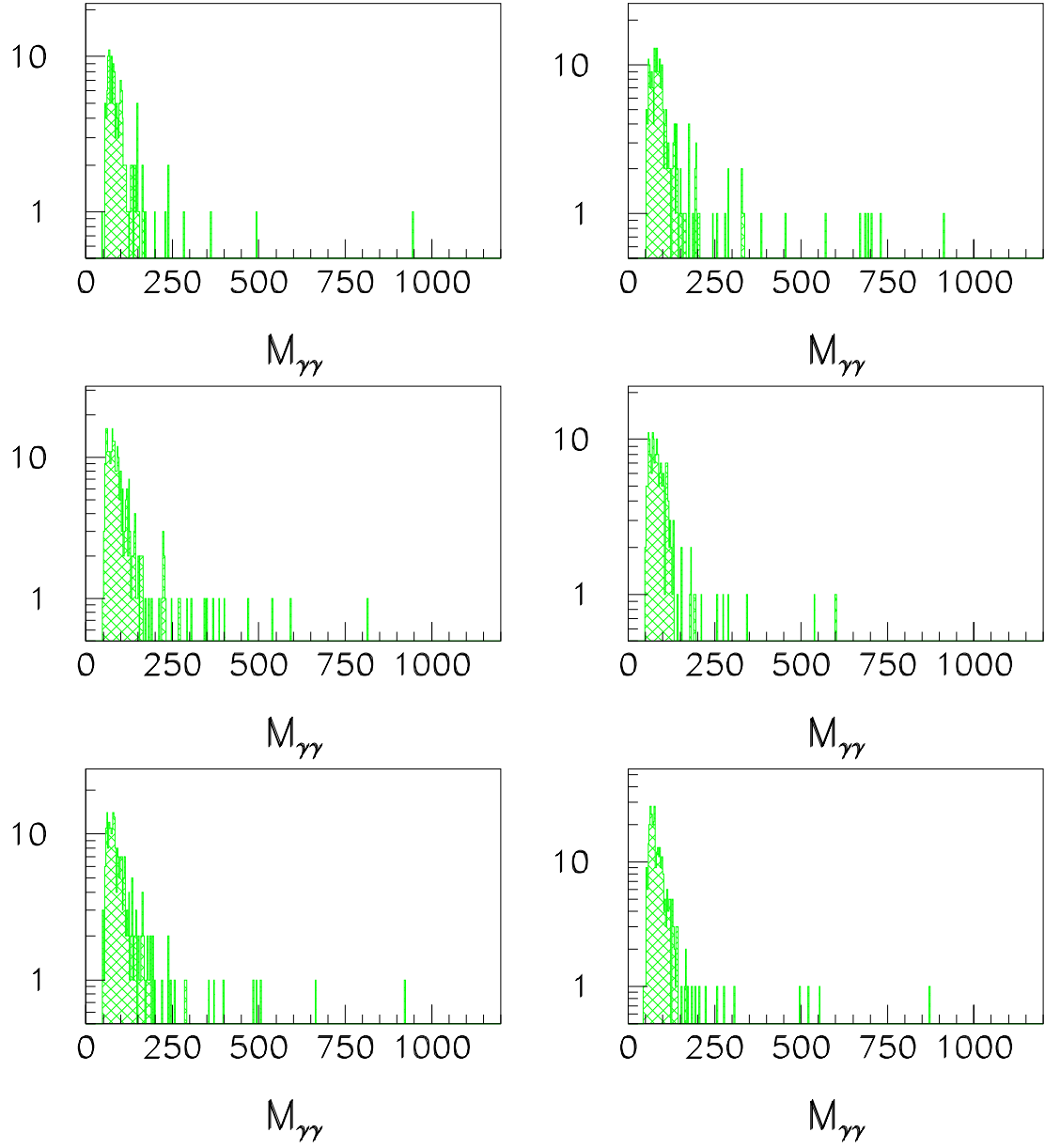
Figure 6.6: Invariant mass distribution for pseudoexperiments in presence of extra dimensions generated with \lambda = -1 and M_s = 600 \text{ GeV} .
