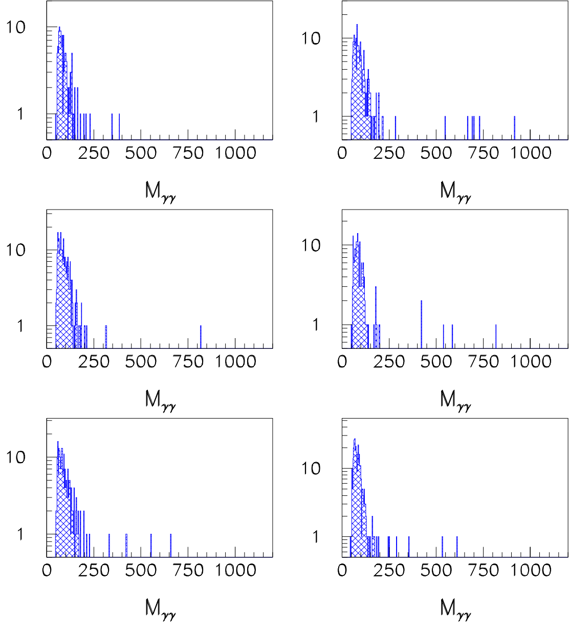
Figure 6.7: Invariant mass distribution for pseudoexperiments in presence of extra dimensions generated with \lambda = +1 and M_S=600 \text{ GeV} .
