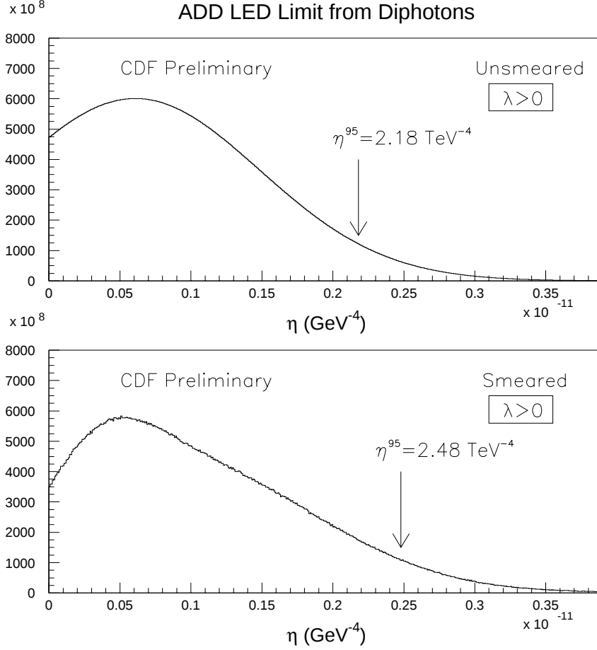
Figure 7.4: Unsmeared (top) and smeared (bottom) likelihood function for the combined CC+CP diphoton data sample for \lambda = +1 .
