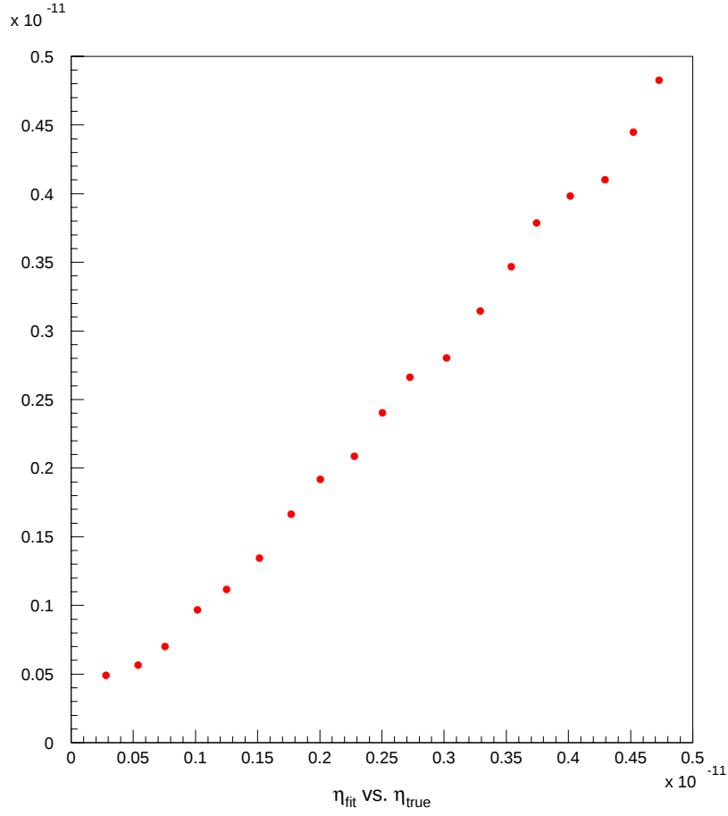
Figure 7.1: \eta_{\text{fit}} ( \eta that minimizes the likelihood function) versus \eta_{\text{true}} ( \eta used to generate pseudoexperiments). The linear correspondence exemplifies the fact that the likelihood function correctly interprets the data in the presence of extra dimensions.
