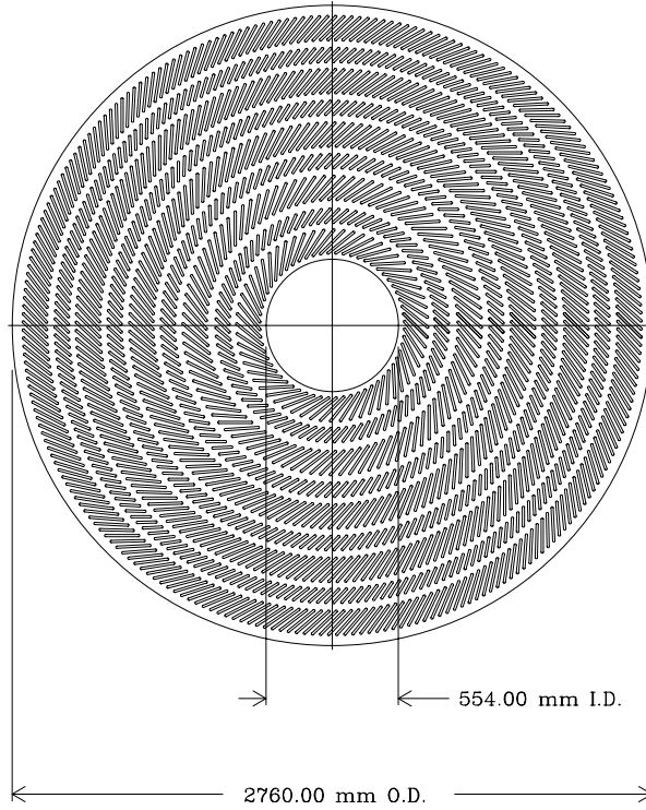
Figure 3.6: Transverse view of the CTC. The superlayers and the tilted cells are shown.
