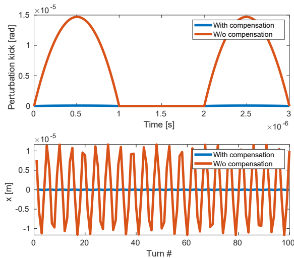
Figure 2: Compensation of the residual bump non-closure using sextupole correctors
