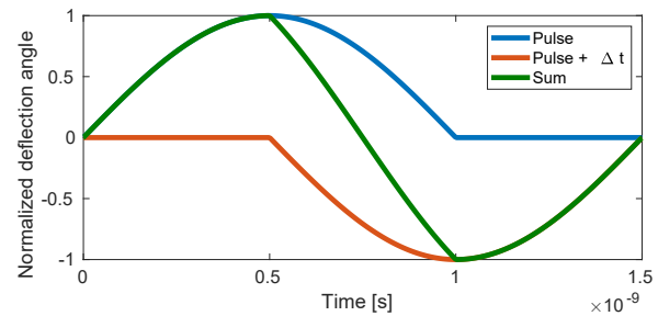
Figure 5: Combining two stripline pulse to reduce the fall time
