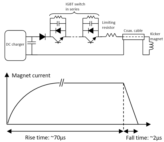
Figure 3: Topology (top) and pulse shape (bottom) of the new kicker power supply
