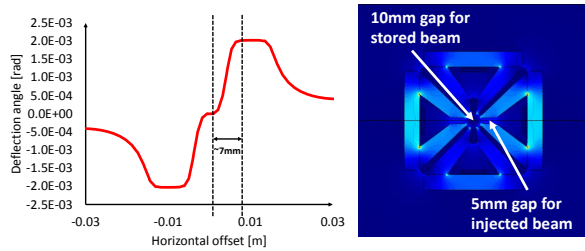
Figure 4: 2D studies of an octupole ferrite core kicker
