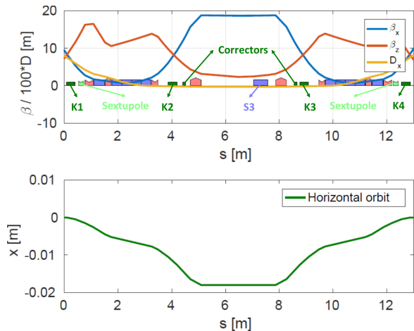
Figure 1: ESRF-EBS injection cells
