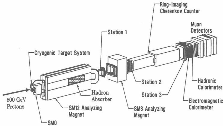
Figure 1: The E605/E772/E789/E866 Spectrometer 5) . The ring-imaging cherenkov counter and the two calorimeters were not used to provide data for the experiment.
