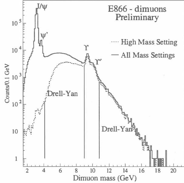
Figure 2: Preliminary dimuon mass spectra from the \bar{u}/\bar{d} run. The upper solid line shows the mass distribution for the sum of all three data sets while the lower dashed curve shows the high mass data set only.
