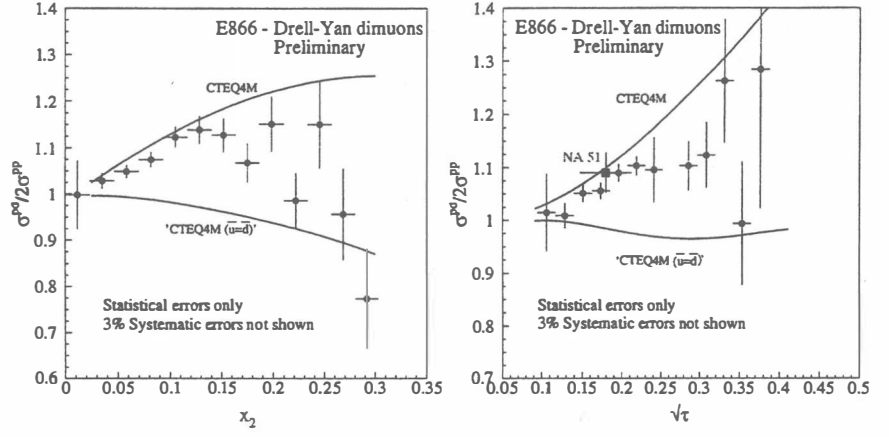
Figure 4: Preliminary results for \sigma^{pd}/2\sigma^{pp} versus x_2 and \sqrt{\tau} .
