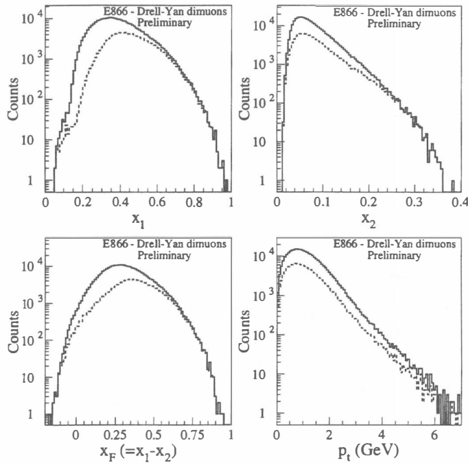
Figure 3: Spectra of the kinematic quantities x_1 , x_2 , x_F , and p_t for dimuons recorded from all mass settings (solid) and from the high mass setting (dashed).
