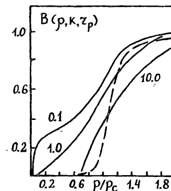
Fig.1. Function (5) at E = 1 keV (solid lines), E = 0.1 keV (dashed line). Numbers near solid lines are the values of parameter \gamma_p in units of R .
