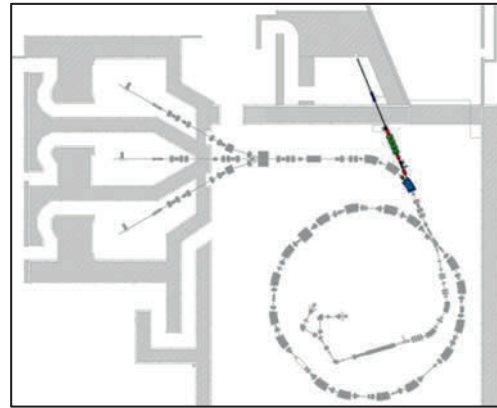
Figure 1: Layout of CNAO. Coloured the new implemented experimental line.
