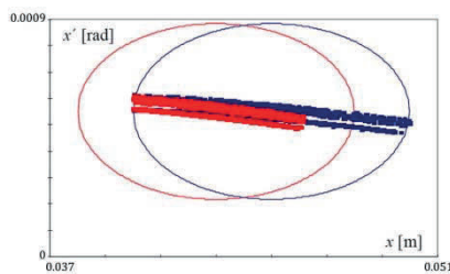
Figure 3: Bar of charge and empty ellipses for minimum and maximum \Delta p/p of the extracted beam. The red bar of charge corresponds to \Delta p/p = -0.001 and the blue one to \Delta p/p = 0.0 .
