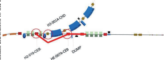
Figure 6: Chopper closure scheme and magnets involved.
