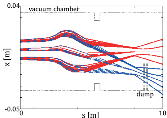
Figure 7: Beam sent to the experimental room (red) and to the dump (blue).
