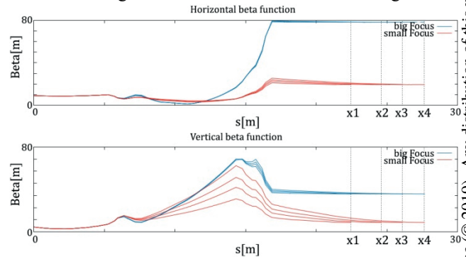
Figure 4: Betatron functions in the XPR beam line for small and large beam size at the four irradiation positions.
