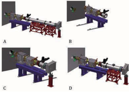
Figure 2: Beamline configurations in the XPR. Scanning magnets and nozzle are mounted on removable supports.
