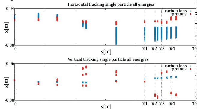
Figure 5: Tracking for both Protons and Carbon ions starting from measured beam position and divergence.
