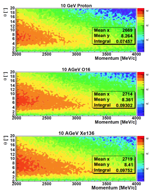
Figure 9: The momentum-angle distribution for the scaled yields of Pi+ for ^1\text{H} , ^{16}\text{O} and ^{136}\text{Xe} .
