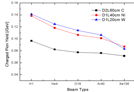
Figure 4: The production efficiency of forward charged pions within the range of 100 ~ 500 MeV/c.
