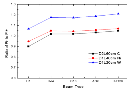
Figure 6: The ratio of \text{Pi}^- to \text{Pi}^+ for 100 ~ 500 MeV/c pions.
