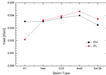
Figure 8: The production efficiency of Pi+ and Pi- within the 2 ~ 4 GeV/c range.
