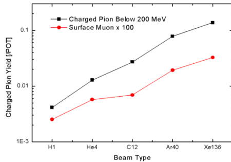
Figure 2: The yields of the charged pions below 200 MeV/c and surface muons for different beams with 1.5 GeV energy.
