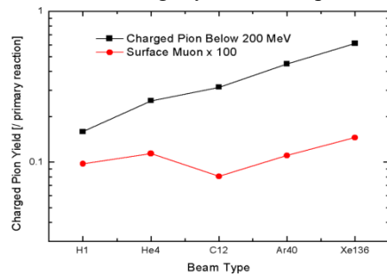
Figure 3: Same as Fig. 2 except that the yield is divided by primary reaction number instead of POT.
