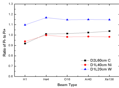
Figure 7: The ratio of Pi- to Pi+ for pions below 200 MeV/c.
