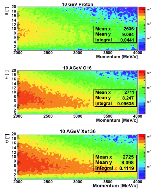
Figure 10: Same as Fig. 9 except for Pi-.
