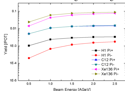
Figure 1: The yields of Pi+ and Pi- below 200 MeV/c for ^1\text{H} , ^{12}\text{C} and ^{136}\text{Xe} with energy varies from 0.5 to 2.5 AGeV with a 1-cm thick graphite target.
