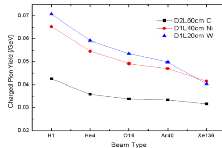
Figure 5: The production efficiency of charged pions below 200 MeV/c.
