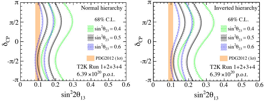
Fig. 3. Results of the T2K experiment. Fitted values of \theta_{13} as a function of \delta_{CP} for different hierarchies and values of \theta_{23} . Grey/orange band represents PDG2012 reactor average value of \sin^2(2\theta_{13}) = (0.098 \pm 0.013) . Note: These are 1D contours for various value of \delta_{CP} , not 2D contours. Pictures taken from [8].
