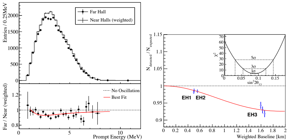
Fig. 2. Daya Bay results. Left: measured prompt energy spectrum of the far hall compared with the no-oscillation prediction based on the measurements of the two near halls along with the ratio of the two. Right: ratio of measured versus expected signals in each detector, assuming no oscillation and the result of fit in the inset. Pictures taken from [1].
