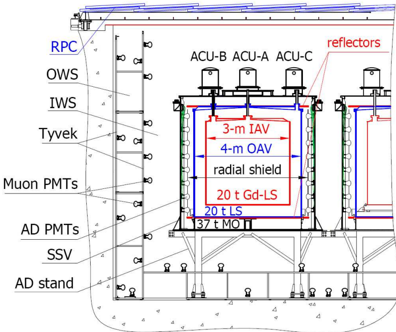
Fig. 1. Schematic view of a Daya Bay detection module. Picture taken from [1].
