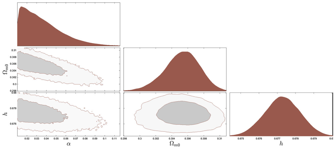
Fig. 3 The 2\sigma confidence level contour plots for various pairs of the free parameters (\alpha, \Omega_{m0}, h) for which the \phi CDM model with the Ratra-Peebles potential V(\phi) = V_0 M_{\text{pl}}^2 \phi^{-\alpha} is in the best fit with the \Lambda CDM model
