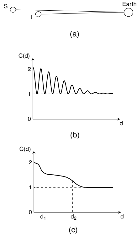
Fig.7. (a) Two stars, S , and T , along nearby lines of sight from the earth; (b) schematic of HBT measurement of correlated intensity from the two stars; (c) schematic of HBT measurement a bright star surrounded by a halo of dim stars.
