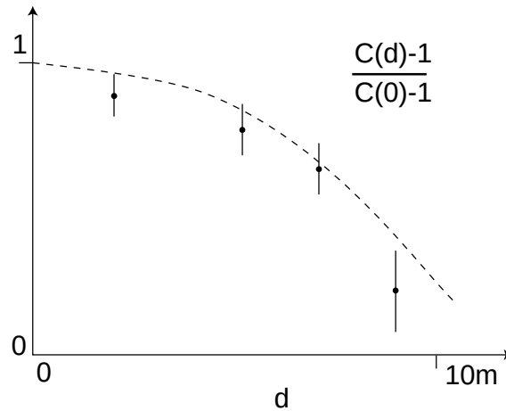
Fig. 4. Measurement of the angular diameter of Sirius [15]
