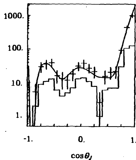
Figure 6-9. \lambda^0 decay distributions at 100 (row including the scatterplot) and 175 GeV/c (lower row). For this figure, |t_{pn}| < .15 \text{ (GeV/c)}^2 .
