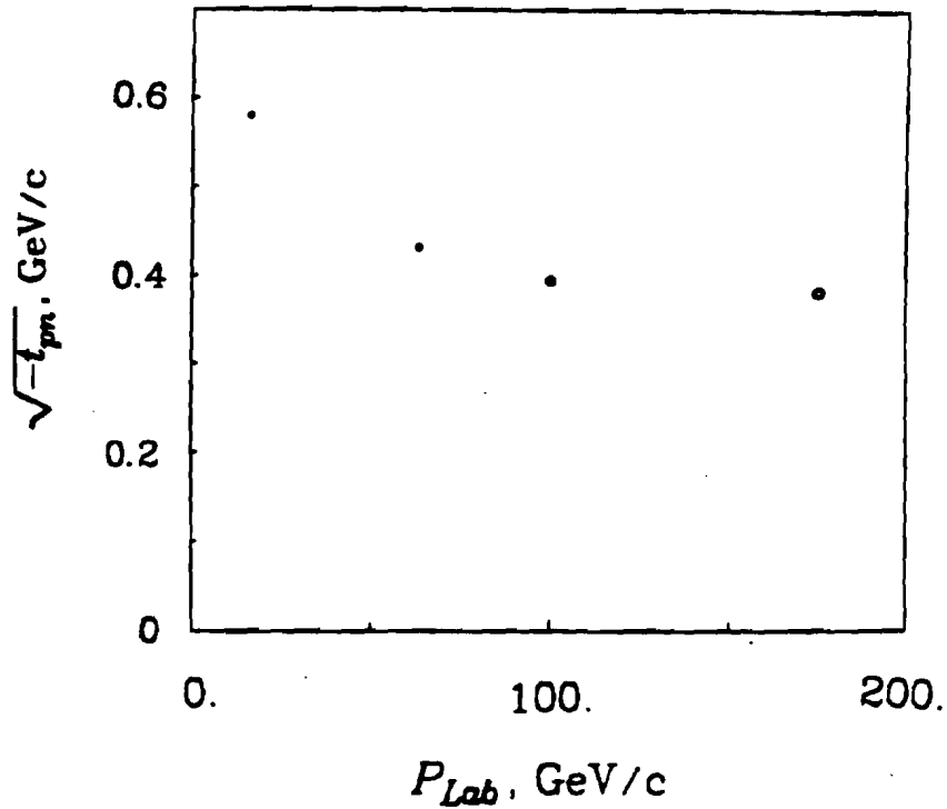
Figure 5-14. "Shrinkage" of the \rho^0 <Y_2^0> versus t_{pn} zero crossing point from 17 to 175 GeV/c. See text.
