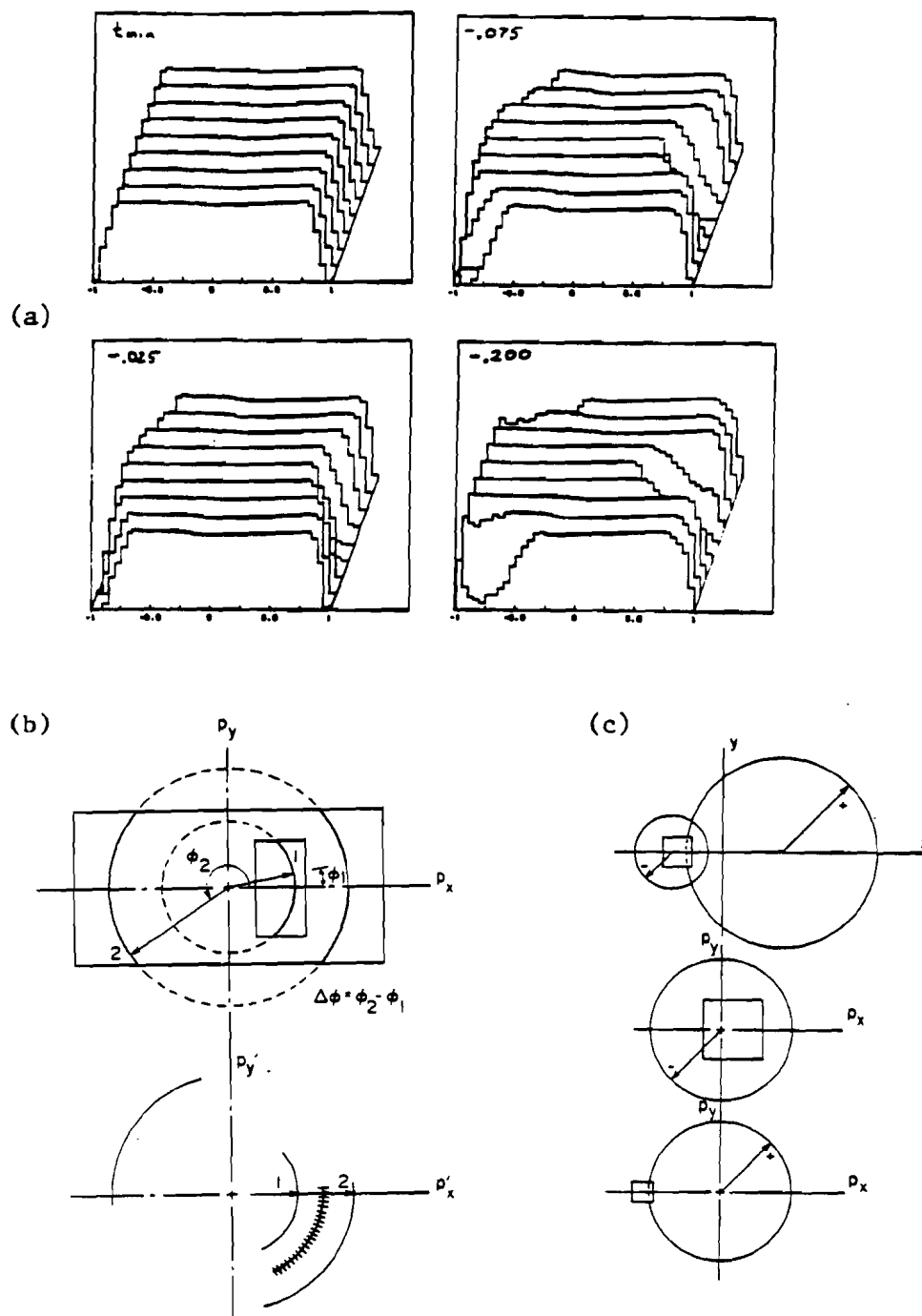
Figure 5-1. (a) 100 GeV/c acceptance at m_{\pi\pi} = 1.25 and several t_{\pi\pi} values. Nine slices in \phi_J are shown, the nearest one at -180^\circ , and the farthest at +180^\circ . Each \phi_J slice shown is an average of two neighboring slices in the grid. The horizontal axis is \cos\theta_J . (b, c) Arcs for MPS and 2 \times 2 apertures, arbitrary scale. Dashed arcs are forbidden. For the 2 \times 2 , the upper drawing is in position space, all other arcs are in p_i space. A rigid body rotation keeps \Delta\phi constant. Correlation calculations are shown for MPS arcs only (hatched arc is not accepted).
