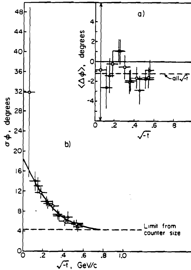
Figure D-8. Recoil neutron azimuth resolution at 100 GeV/c (b). Points were found in three sets of fits to a Gaussian plus flat background. Smooth line is the dependence used in E_{\pi\pi} measurement. This was not used for the study of figure D-6, but was used for our E_{\pi\pi} measurement. Also shown (a) is the error in surveyed counter orientation.
