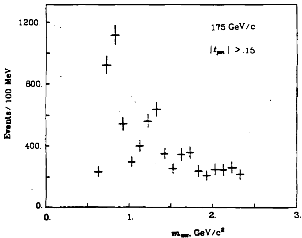
Figure 5-6. High t_{\pi\pi} mass spectra at 100 and 175 GeV/c. .15 < |t_{\pi\pi}| < 1.0 (GeV/c) 2 .
