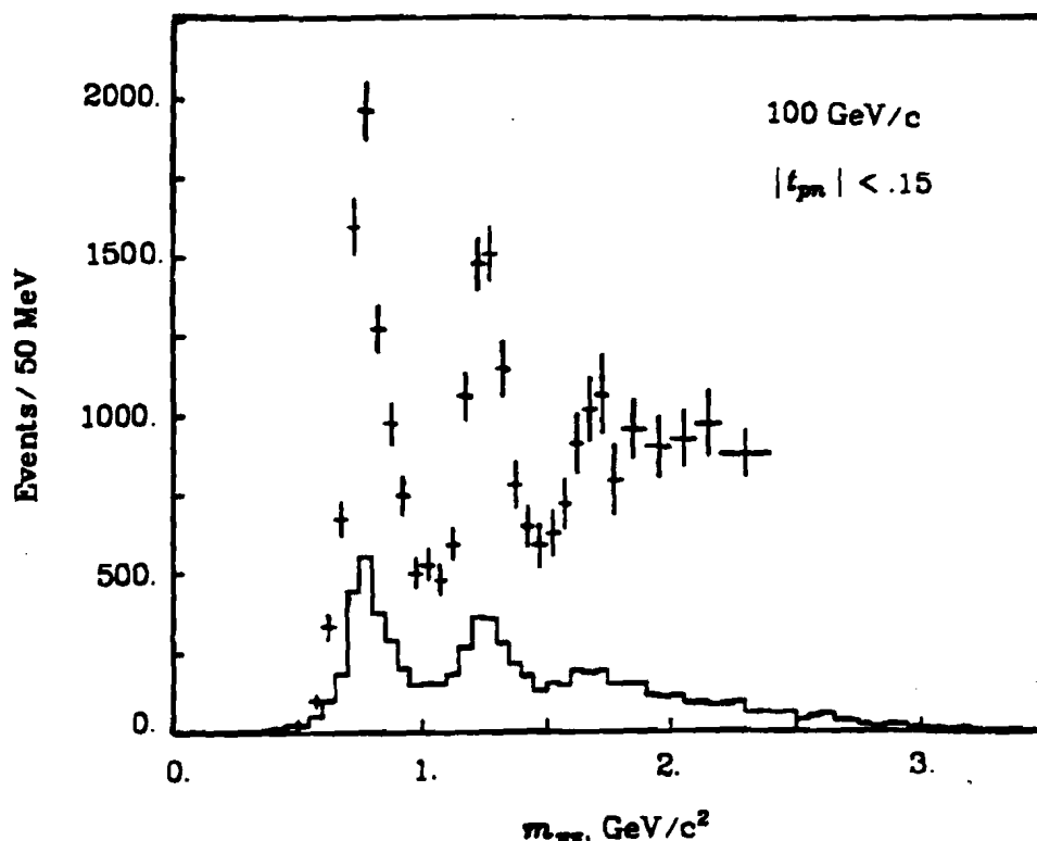
Figure 5-4a 100 GeV/c \pi\pi mass spectrum for |t_{pn}| < .15 (GeV/c) 2 . Points with error bars are produced event totals from moment fits with L_{max} = 8 and m_{max} = 1 . The histogram is the uncorrected event total in 50 MeV/c bins from figure 1-2.
