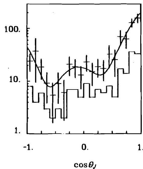
Figure 6-8. g^0 decay distributions at 100 (row including the scatterplot) and 175 GeV/c (lower row). For this figure, |t_{pn}| > .15 \text{ (GeV/c)}^2 .
