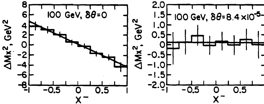
Figure C-2. \Delta Mx^2 before (a) and after (b) kink correction.
