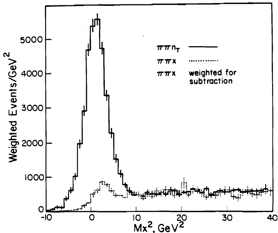
Figure 4-1. 100 GeV/c Mx^2 spectrum for \pi\pi n_T and fully weighted \pi\pi X spectrum. By construction, the veto weight gives cancellation at high missing masses. (Deviations result from averaging inefficiencies measured at 20, 50 and 100 GeV/c.) Under the neutron peak, the shape is mainly determined by measured failure rates at 20 and 50 GeV/c, and has a small model dependent \Delta(1236) component.
