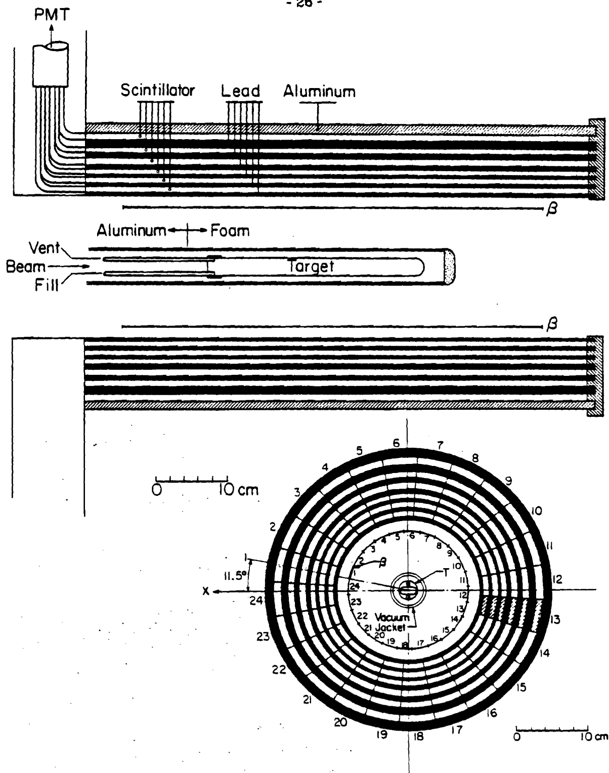
Figure 2-5. Side and front views of V1. Details of the target, vacuum jacket and counter orientation (surveyed at 11.5°) are also shown. Signal cables for the \beta proportional chamber exit the front of V1. Numbered segments refer to tag bits for V1 and \beta . The \beta and V1 segments overlapped. In the trigger, a hit in any \beta segment turned off the two V1 segments behind it.
