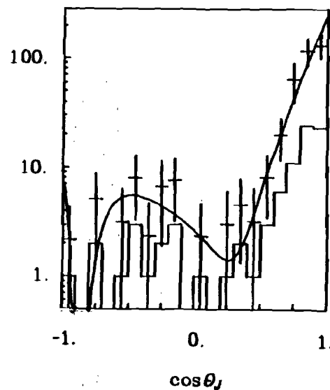
Figure 6-10. h^0 decay distributions at 100 (row including the scatterplot) and 175 GeV/c (lower row). For this figure, |t_{pi}| > .15 \text{ (GeV/c)}^2 .
