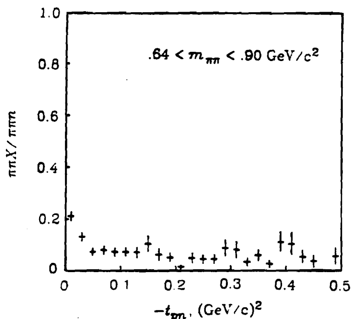
Figure 5-16. 100 \text{ GeV}/c \rho^0 region \pi\pi X / \pi\pi\pi ratio.
