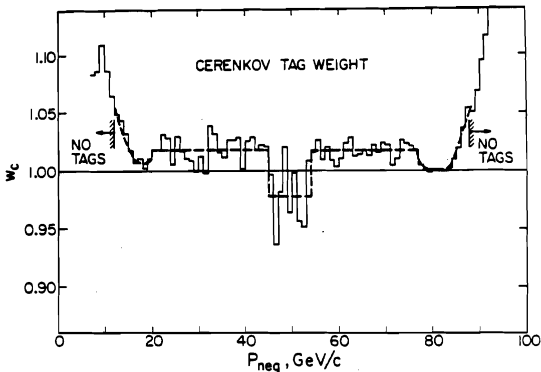
Figure 4-10. Weight for the C1 C2 \pi\pi tag. Dashed curve is the value actually applied. The data curve is from equation 4.13, the efficiencies in figure 4-9, and observed \pi\pi\pi\gamma events.
