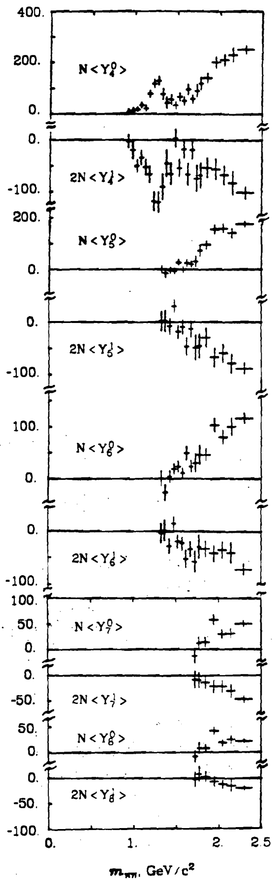
Figure 5-8. 175 GeV/c unnormalized moments. See text.
