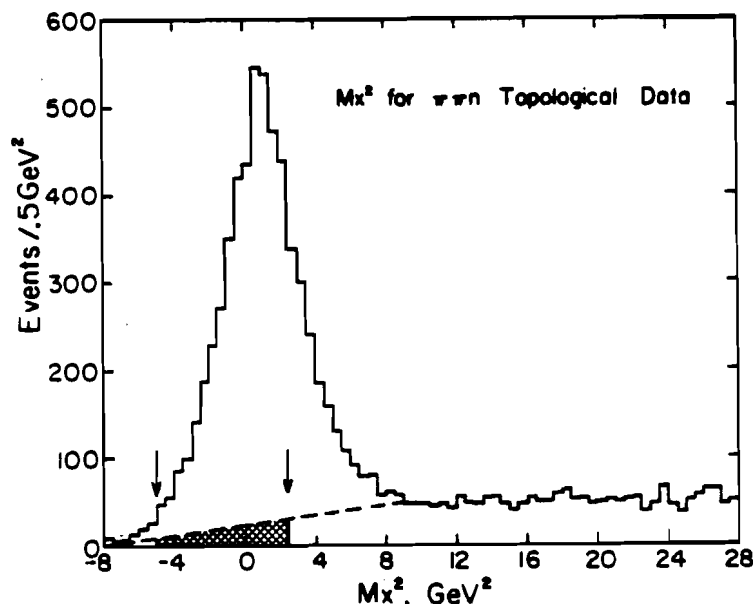
Figure D-5. Mx^2 spectrum for \pi\pi\pi\eta data used in neutron veto study. Shown are Mx^2 cuts used, and the rough background estimate used.
