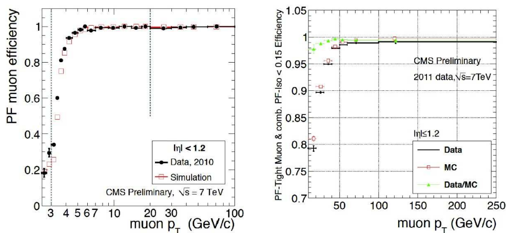
Figure 6. Reconstruction and isolation efficiency of muons as a function of momentum are compared between data and Monte Carlo.
