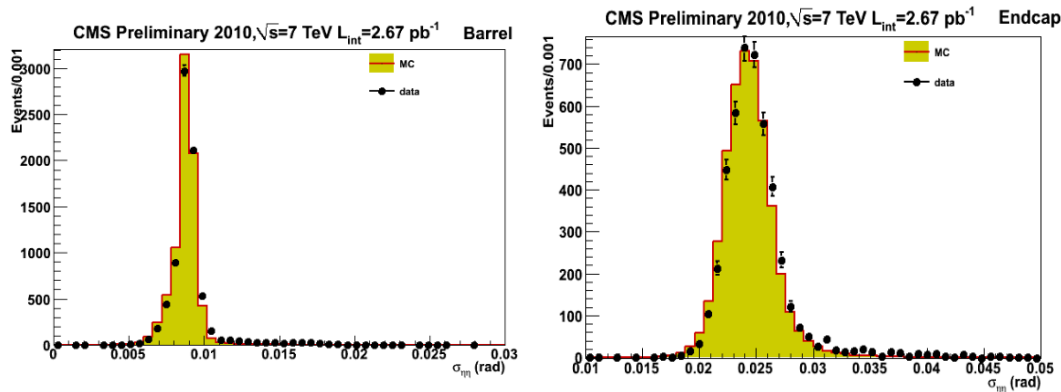
Figure 4. Comparison of widths of electromagnetic showers (along \eta direction) between data and Monte Carlo in the barrel and in the endcap electromagnetic calorimeter.
