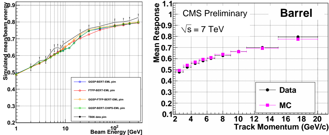
Figure 5. (a) Mean energy responses for \pi^- as a function of incident particle momentum. Predictions of the four physics lists QGSP_BERT_EML, QGSP_FTFP_BERT_EML, QGSP_BERT_CHIPS_EML and FTFP_BERT_EML are also shown. (b) Mean response measurements as a function of track momentum in the barrel calorimeter. Monte Carlo prediction is compared with the data.
