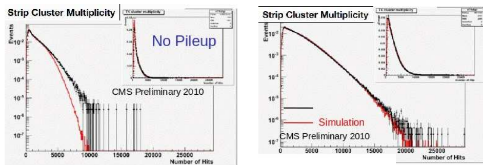
Figure 2. Comparison between data and Monte Carlo for occupancy in the silicon strip tracker with or without the effect of pileups.
