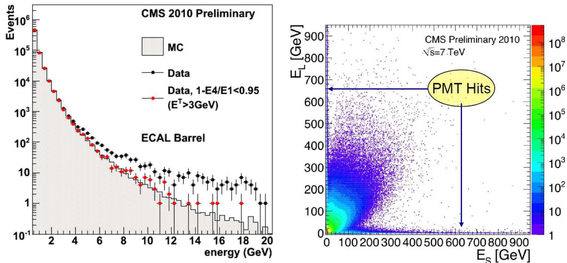
Figure 7. Distributions of energy deposit in the barrel ECAL (left) compared to the prediction of Monte Carlo. The red points refer to the data after the application of the noise filter. The plot on the right refers to a scatter plot of energy deposits in the long and in the short fibres.
