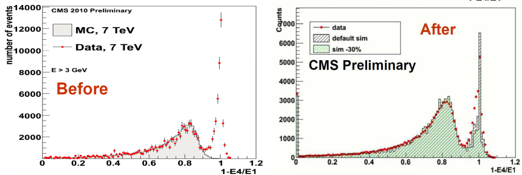
Figure 8. Comparison of data and Monte Carlo for the ratio of energy deposit in a 2 \times 2 crystal matrix to the energy in the most energetic crystal. The Monte Carlo distributions are obtained without (left plot) and with (right plot) the inclusion of energy deposits in the thin silicon layer of the APD.
