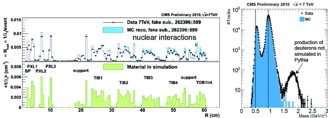
Figure 3. (a) Study of the tracker material using nuclear interactions in the data and in the Monte Carlo. (b) Estimation of mass of the charged particles from measurements of the momentum and dE/dx in the data and in the Monte Carlo.
