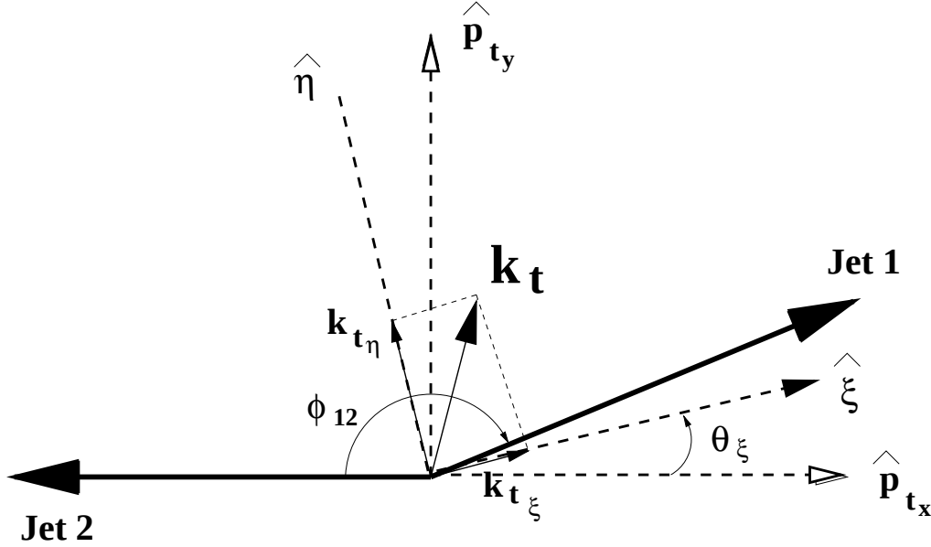
Figure 4.16: The total transverse momentum \vec{K}_T of the di-jet system is decomposed into two components K_{T_\eta} and K_{T_\xi} sensitive to different effects generating it. To have symmetric distributions the label 1 is randomly attributed to the lower \phi jet.
