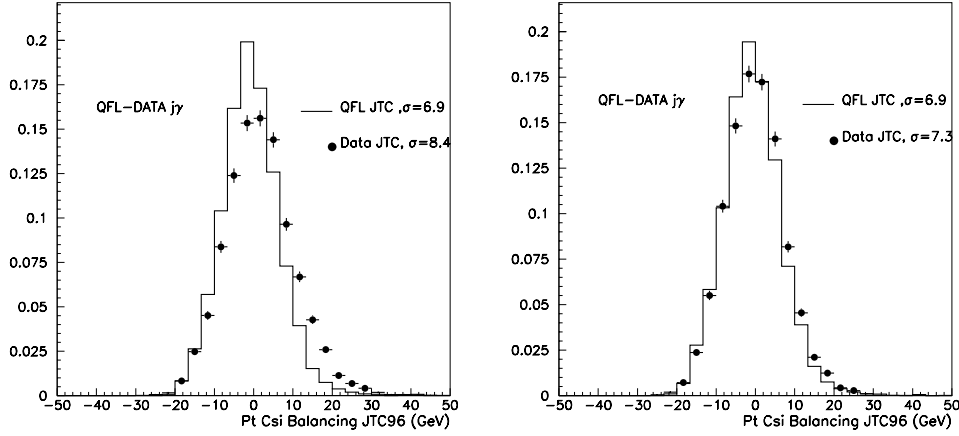
Figure 4.8: Distribution of the \gamma -jet balancing P_{T\gamma} component for the data (dots) and a Pythia+QFL sample (histo). JTC96 corrections are applied. Events are selected in the 25 < P_T^\gamma < 35 GeV bin and the distributions are normalized to 1. The new photon selection criteria (right) provide a better agreement between data and MC than the previous study of ref. [37] (left).
