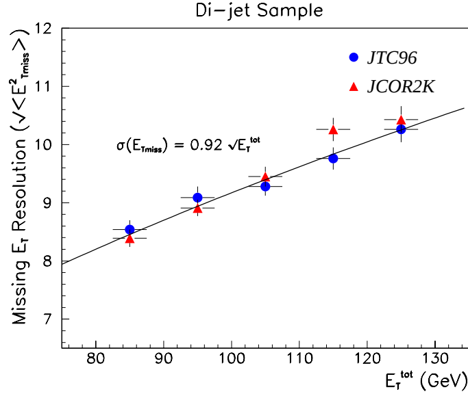
Figure 4.21: \sigma_{\vec{E}_T} as a function of the total scalar E_T of the event. The distributions are obtained after correcting the \vec{E}_T for the JTC96 or JCOR2K jet corrections. The trigger bias is removed applying standard cuts.
