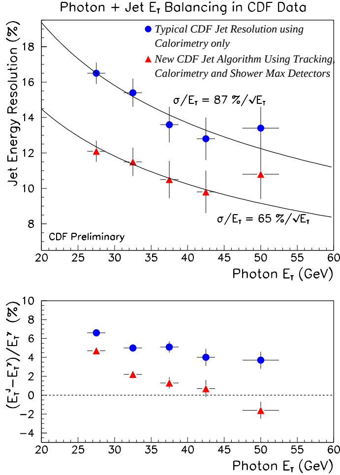
Figure 4.11: Top: The central detector resolution \sigma_D is plotted as a function of P_T^\gamma for the two methods. Bottom: The (E_T^{\text{jet}} - P_T^\gamma)/P_T^\gamma balancing offset is plotted as a function of P_T^\gamma for the two methods. The E_T of the jets has been used for the photon-jet balancing.
