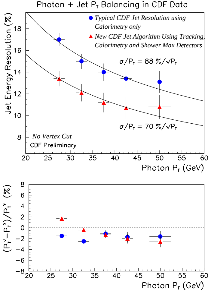
Figure 4.12: Top: The central detector resolution \sigma_D is plotted as a function of P_T^\gamma for the two methods. Bottom: The (P_T^{jet} - P_T^\gamma)/P_T^\gamma balancing offset is plotted as a function of P_T^\gamma for the two methods. The P_T of the jets has been used for the photon-jet balancing. No vertex cut has been applied.
