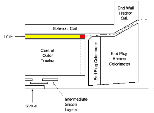
Figure 1.9: TOF scintillator bars in CDF II.
