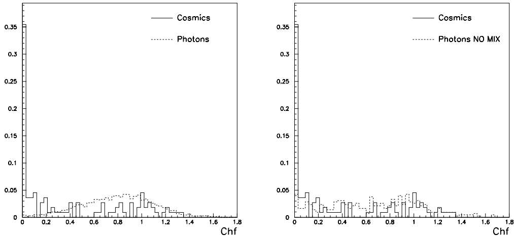
Figure 5.9: Chf distributions for photons and cosmics (left) and for photon NO MIX and cosmics (right). Values greater than 1 derive from the SCALAR sum on tracks P_T . No indication is seen of a significative cosmics background in the photon NO MIX sub-sample. All distributions are normalized to 1.
