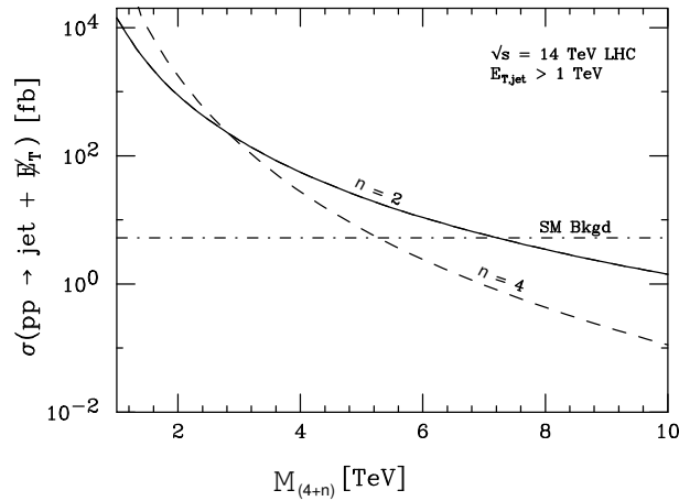
Figure 3. Missing energy due to graviton emission at LHC, as a function of the higher-dimensional gravity scale M_* , produced together with a hadronic jet. The expected cross-section is shown for n = 2 and n = 4 extra dimensions, together with the SM background.
