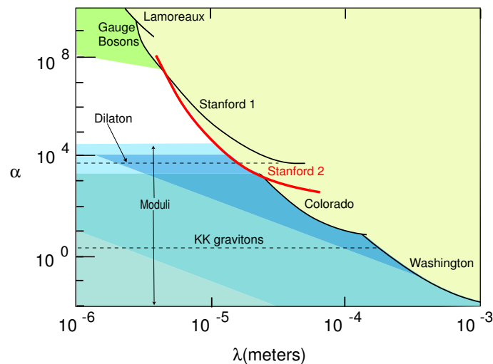
Figure 4. Present limits on non-Newtonian forces at short distances (yellow regions), as a function of their range \lambda and their strength relative to gravity \alpha . The limits are compared to new forces mediated by the graviton in the case of two large extra dimensions, and by the radion.
