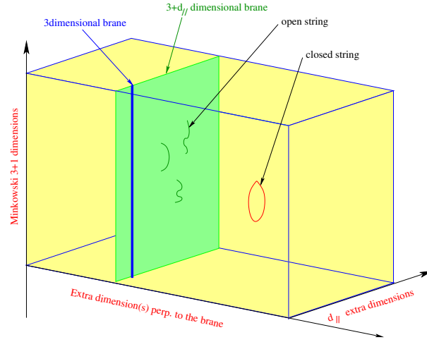
Figure 1. In the type I string framework, our Universe contains, besides the three known spatial dimensions (denoted by a single blue line), some extra dimensions ( d_{||} = p - 3 ) parallel to our world p -brane (green plane) where endpoints of open strings are confined, as well as some transverse dimensions (yellow space) where only gravity described by closed strings can propagate.
