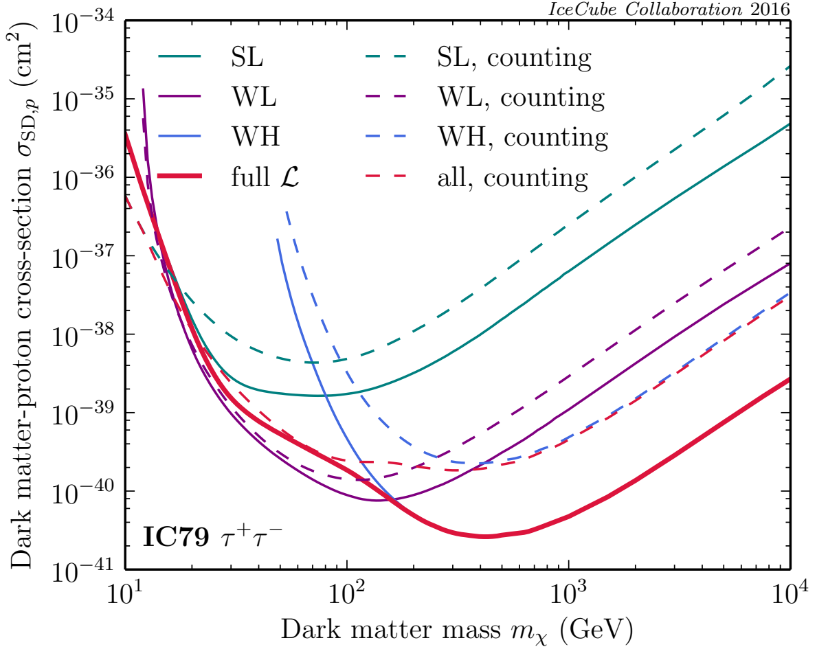
Figure 4. Limits on dark matter annihilation in the Sun using an analysis that takes into account neutrino energy information. We show limits separately for the three different IC79 event samples SL (summer low) WL (winter low) and WH (winter high) and their combination. The difference between dashed and solid lines indicates the improvement gained by moving from a simple counts-based number likelihood to a full unbinned one, incorporating the number of events, their arrival directions and energies. The full limit is weaker than the WL sample taken alone at low masses, because the SL sample exhibits a weak excess ( < 2\sigma local significance) of events above background expectation, not borne out in the WL sample. Here we have assumed an annihilation cross-section of \langle\sigma v\rangle_0 = 3 \times 10^{-26} \text{ cm}^3 \text{ s}^{-1} entirely into \tau^+\tau^- final states.
