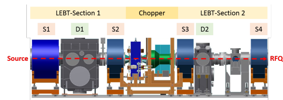
Figure 4: Scheme of the low energy beam transport for HBS. It consists of two sections with an E×B-chopper in between.
