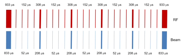
Figure 1: Pulse scheme of the HBS Linac. The spacing between beam pulses is 1.56 ms.
