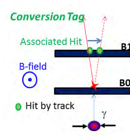
Figure 7.6: Conversion happened at B0 layer leaves two close-by hits in B1.
