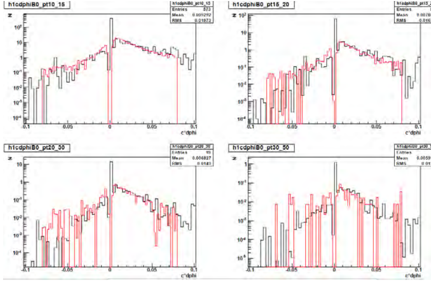
Figure 7.9: cd\phi distribution of the close by VTX hits in layer B0. Black is simulation and red is p + p data. abs(dz) < 0.05 cm cut is applied. 4 p_T bins are 1–1.5 GeV/c, 1.5–2 GeV, 2–3 GeV, 3–5 GeV
