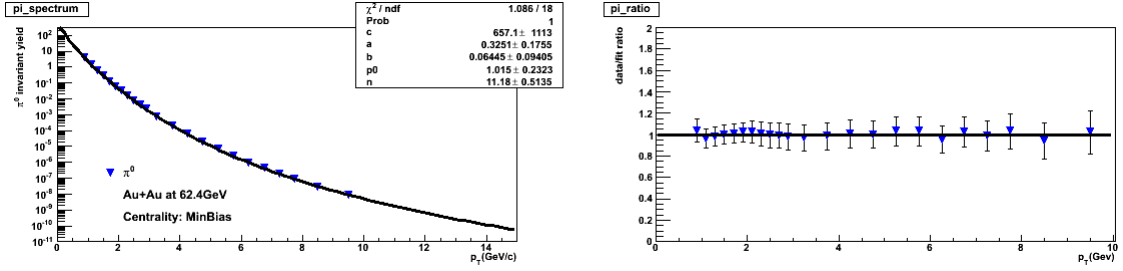
(a) MinBias
