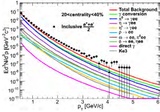
(c) Centrality 20-40%
