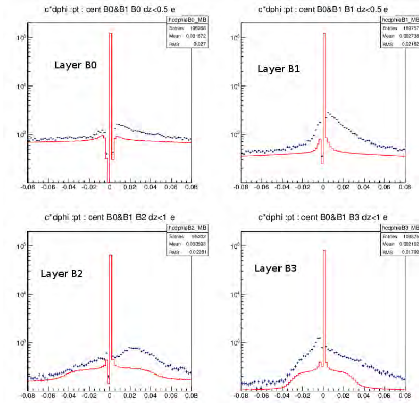
Figure 7.7: Data: hit distributions around a hit of electron tracks and hadron tracks in each of VTX layers [69]
