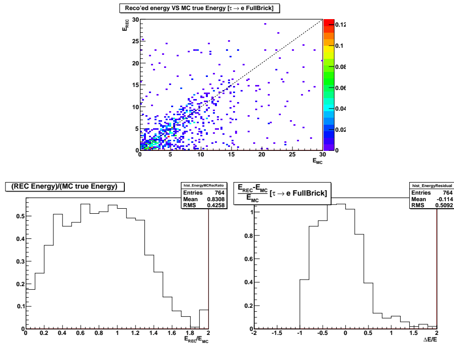
Figure 4.29: Idem with showers reconstructed over the full volume.
