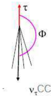
Figure 5.1: Sketch showing the definition of the \Phi_{\text{had}} angle.
