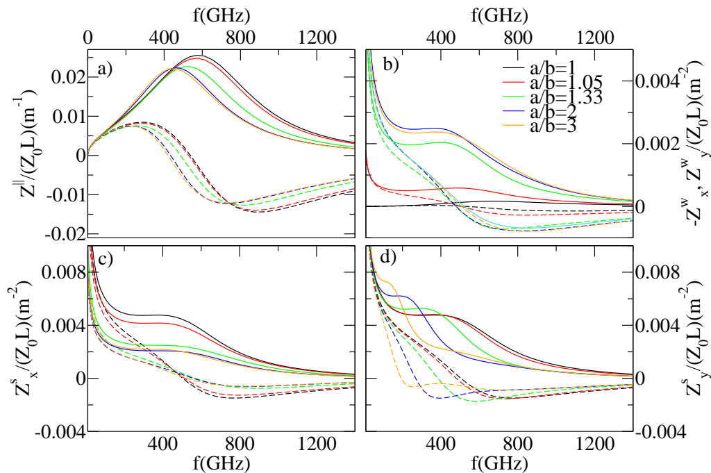
FIG. 2: Large frequency regime, \gamma = 1000 . The perturbation approximation fails when f \gtrsim 60GHz . The real (imaginary) part of the impedance is plotted with solid (dashed) line. At large frequencies the longitudinal impedance (a) decreases with increasing \frac{a}{b} , while the transverse impedances caused by the witness particle displacement (b) increase with increasing \frac{a}{b} . The transverse impedances caused by the source displacement (c) and (d) decrease with increasing \frac{a}{b} .
