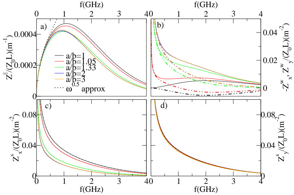
FIG. 3: Non-ultrarelativistic impedance, \gamma = 1.42 . The real and the imaginary part of the impedance fall on top of each other. Finite \gamma effects shows for f > \approx 0.4 \text{GHz} . The impedances corresponding to different value of \frac{a}{b} are not proportional to each other. a) Longitudinal impedance. At large frequencies (above 1 \text{GHz} ) the longitudinal impedance decreases with increasing \frac{a}{b} . b) The transverse impedances caused by the witness particle displacement, -Z_x^w (dashed-dotted line) and Z_y^w (solid line), increase with increasing \frac{a}{b} . The plots for \frac{a}{b} = 2 (blue) and \frac{a}{b} = 3 (orange) are on top of each other. Note that -Z_x^w \neq Z_y^w , unlike the ultrarelativistic case. c) The horizontal transverse impedance Z_x^s decreases with increasing \frac{a}{b} . d) The vertical transverse impedance Z_y^s show negligible dependence on \frac{a}{b} .
