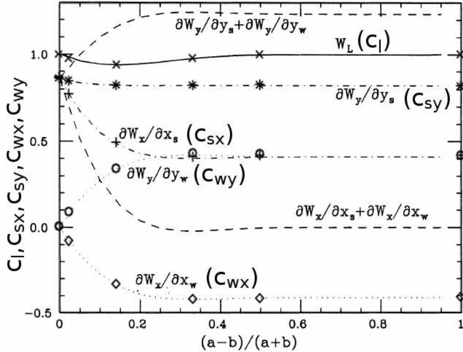
FIG. 1: Perturbative region defined by Eqs. 79. Ultrarelativistic limit, \gamma = 1000 . The longitudinal impedance is proportional to \omega^{\frac{1}{2}} while the transverse impedances are proportional to \omega^{-\frac{1}{2}} . The proportionality coefficients defined by Eqs. 81, 82, c_l (cross), c_{sx} (plus), c_{sy} (star), c_{wx} (diamond) and c_{wy} (circle), are plotted on top Yokoya's [17] Figure 8. Note that the impedances for \frac{a}{b} = 2 ( \frac{a-b}{a+b} = 0.33 ) are very close to the parallel-plane limit ( \frac{a-b}{a+b} = 1 ).
