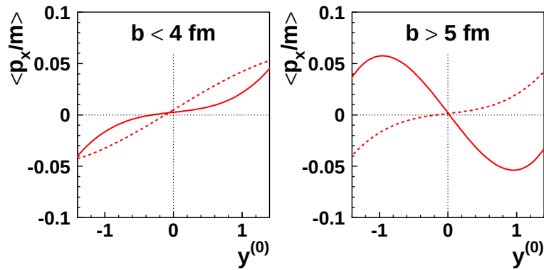
Fig. 2. Model predictions [10] for K^+ flow in Ru+Ru collisions at 1.69-A GeV with (solid curves) and without (hashed curves) in-medium effects ( b is the reaction impact parameter).
