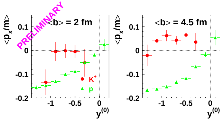
Fig. 3. Flow of K^+ (circles) and protons (triangles) in central (left) and semi-central (right) Ru+Ru events at 1.69-A GeV. Error bars represent statistical uncertainties.
