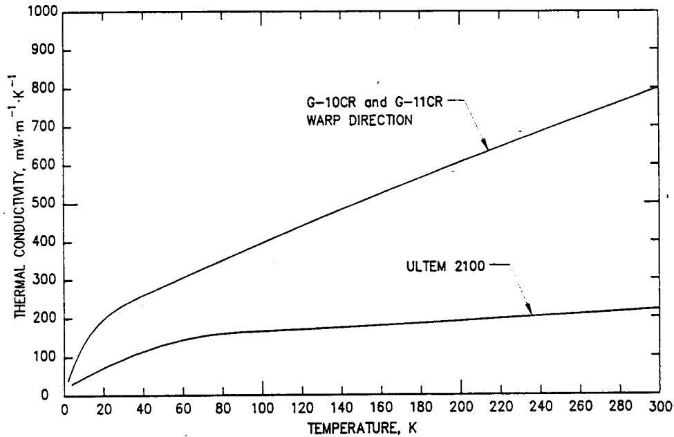
Figure 2. Thermal conductivities at cryogenic temperatures.
