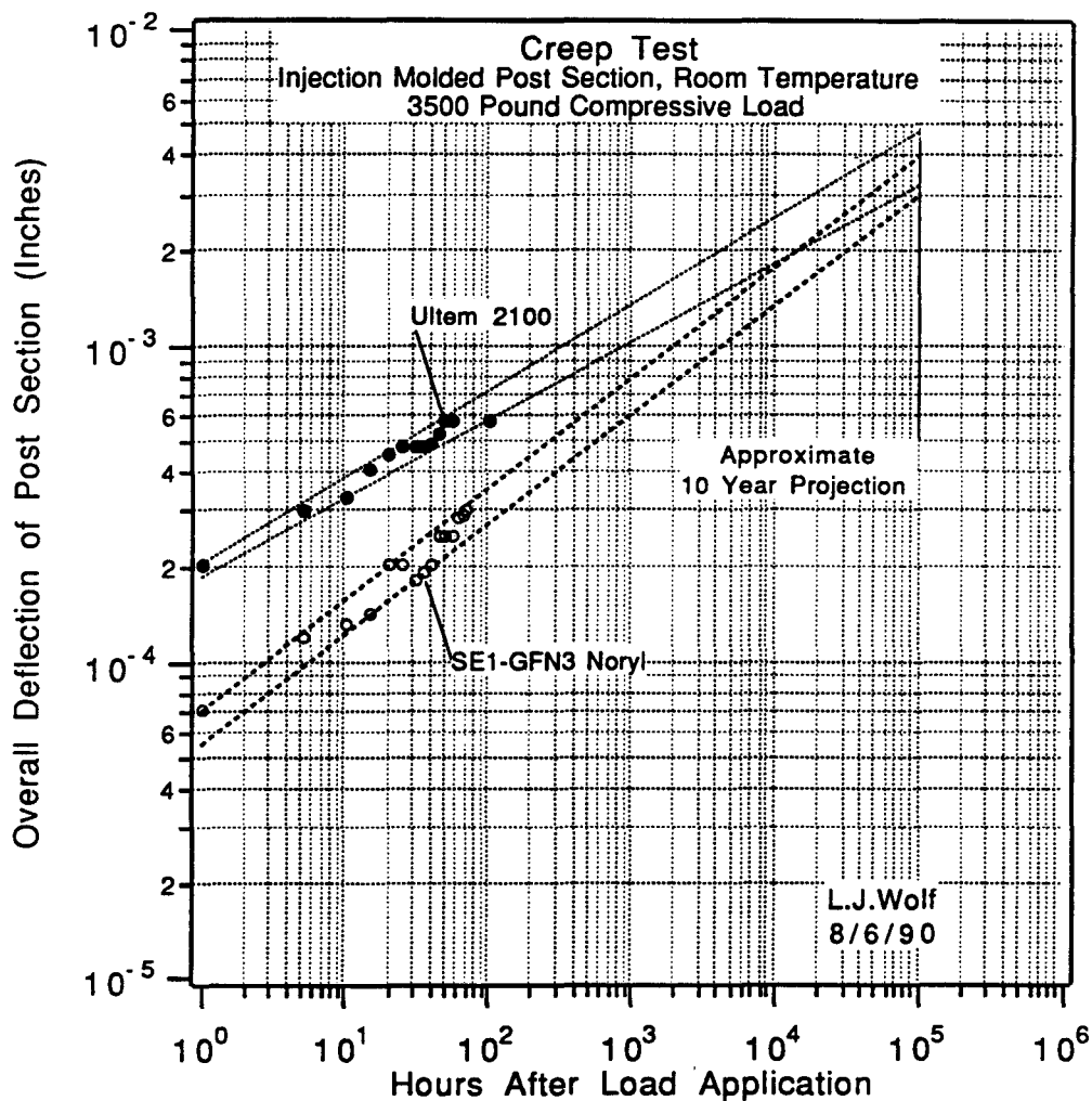
Figure 7. Room temperature creep test results.
