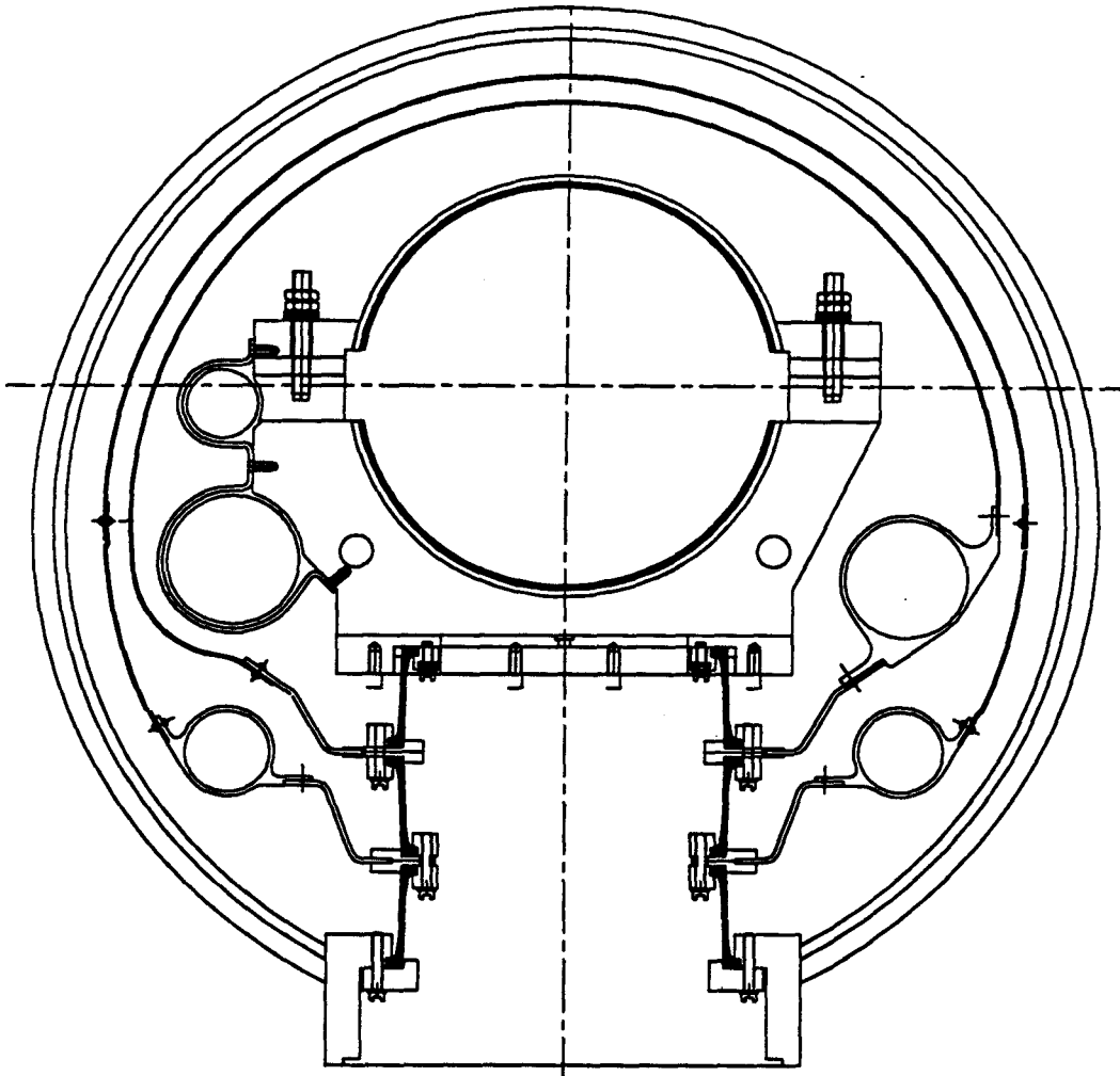
Figure 13. The SSC cryostat redesigned for a post constructed of three identical injection molded composite sections.
