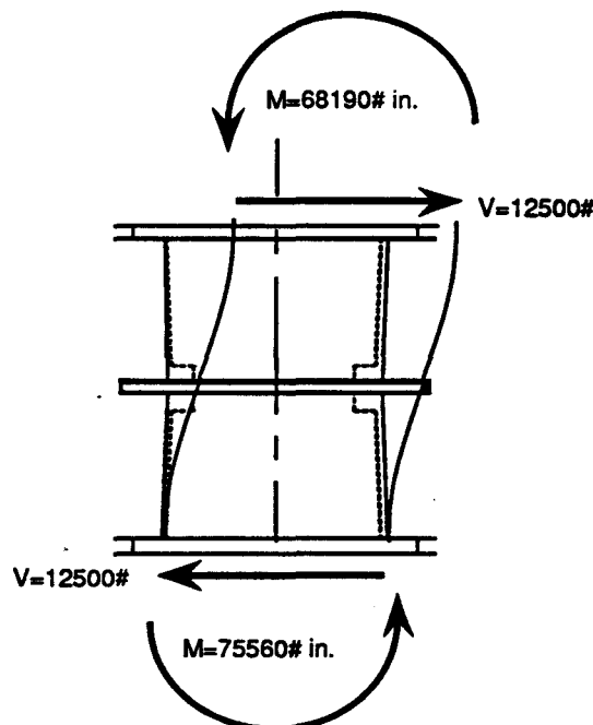
Figure 6. Forces, moments and deflections of the center post.
