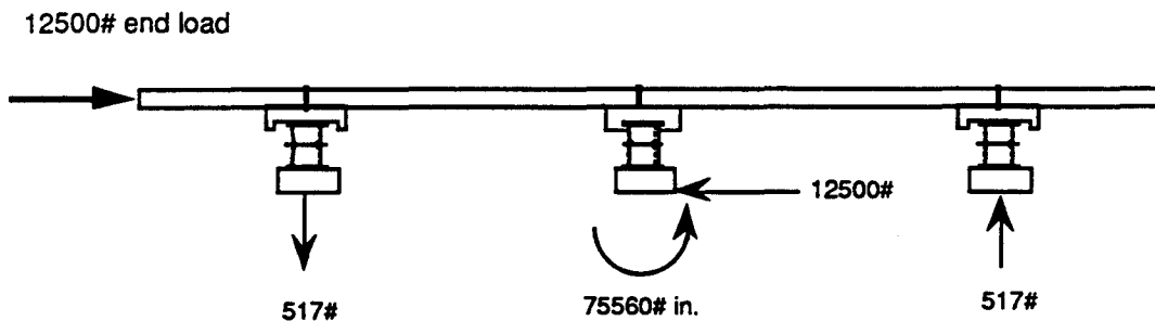
Figure 5. Support reactions on the RHIC fixed center post and sliding side posts due to an end load caused by a catastrophic quench.
