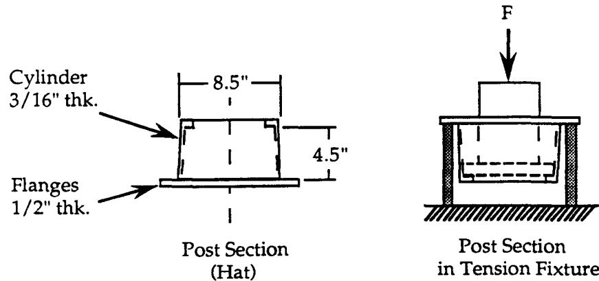
Figure 10. The quality control testing fixture.
