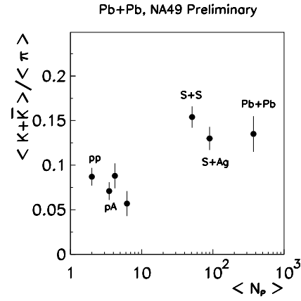
Fig.2. Ratio of the multiplicities of kaons and pions for various target-projectile systems as a function of the number of participants.
