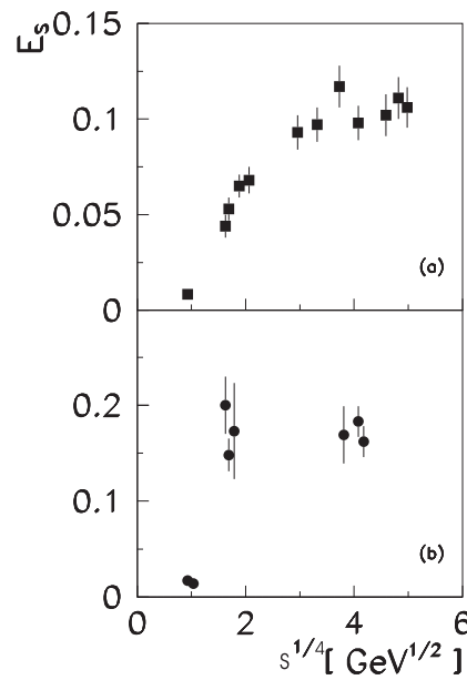
Fig. 3. Strangeness contents E_S for nucleon–nucleon interactions (top) and central heavy ion collisions (bottom) as a function of the bombarding energy.
