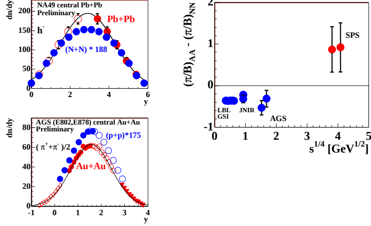
Fig.1. Pion rapidity distributions and pion production per participating nucleon for A + A collisions at various collision energies.
