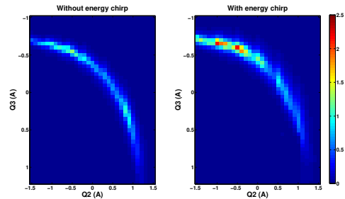
Figure 3: Pyrodetector measurements of coherent transition radiation at X24 as a function of upstream quadrupoles Q2 and Q3. No energy chirp on the beam (left) and with an energy chirp on the beam (right) at 40 degrees off crest.
