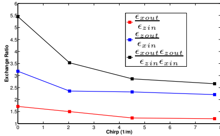
Figure 5: Measured value of the emittance exchange ratio and their products. As the RF-chirp increases, the ratio tends towards one. There is still some emittance dilution possibly due to second order effects and space charge.
