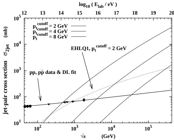
Fig. 2. Inclusive minijet cross section calculated for different minimum transverse momentum cutoffs. For comparison also data on total p - p and p - \bar{p} cross sections are shown together with the Donnachie–Landshoff (DL) model [26].
