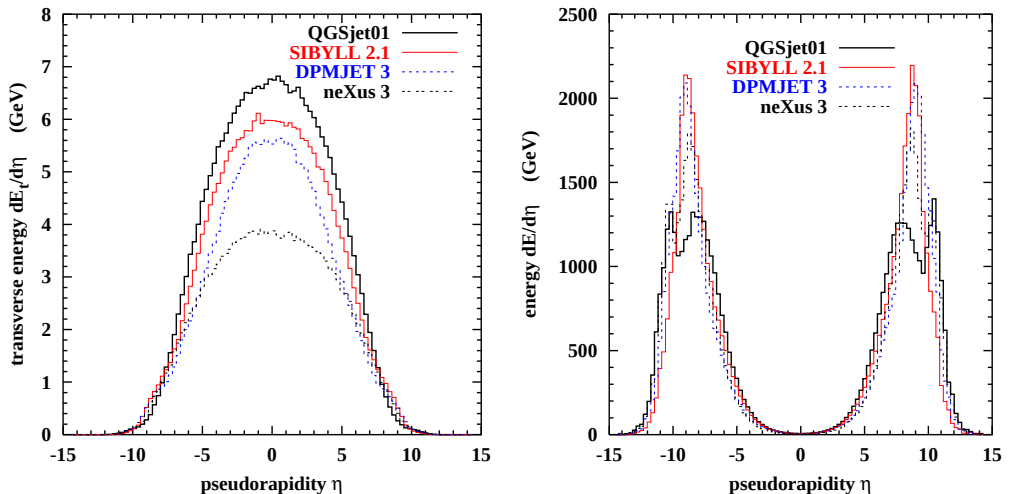
Fig. 3. Predicted transverse and total energy distributions for p - p collisions at LHC energy.
