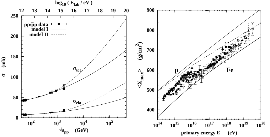
Fig. 4. Left panel: comparison of model results with data on total and elastic p - p and p - \bar{p} cross sections. Right panel: model predictions on mean depth of shower maximum X_{\text{max}} (for references to the exp. data see, for example, [1]).
