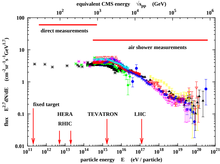
Fig. 1. All particle cosmic ray flux scaled by E^{2.7} . References to the measurements shown can be found in [1, 2].
