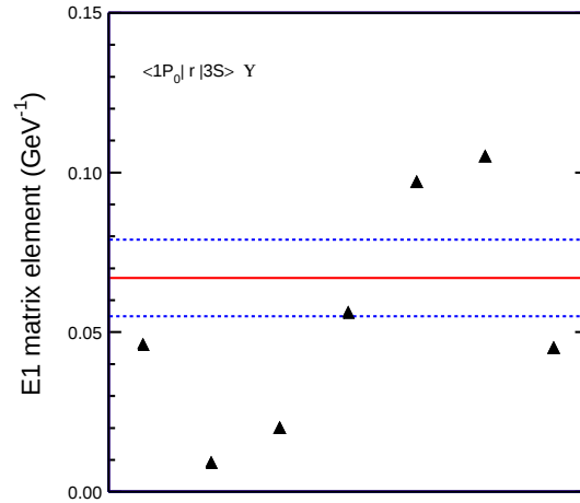
Fig. 5. Measured and predicted values of E1 matrix element for \Upsilon(3S) \rightarrow \gamma\chi_b(1P_0) . The measured value is calculated from the CLEO results for the branching ratio and the total width of the \Upsilon(3S) [17]. The central values and error bars for the measured values are indicated by the solid and dashed lines, respectively. The predictions [19] (triangles) are ordered according to the publication date.
