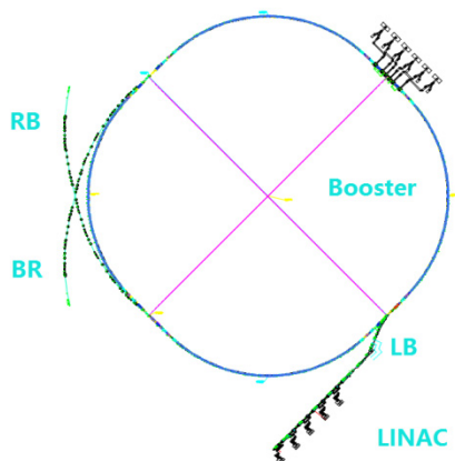
Figure 2: Layout of the HEPS injector.
