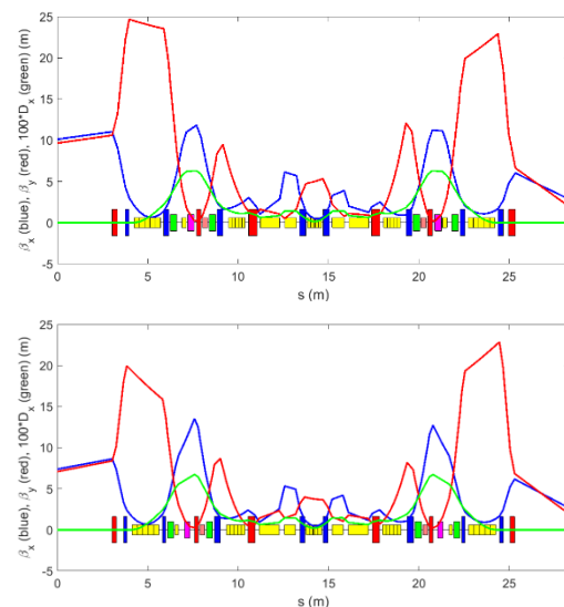
Figure 1: Optical functions and layout of one 7BA of the HEPS storage lattice, V2.0 (upper) and V2.4α (below).
